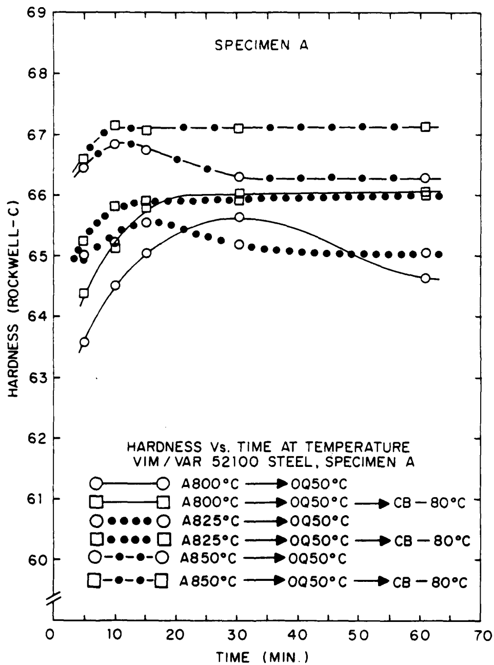
Figure 24. Hardening Response of Treatment-A
