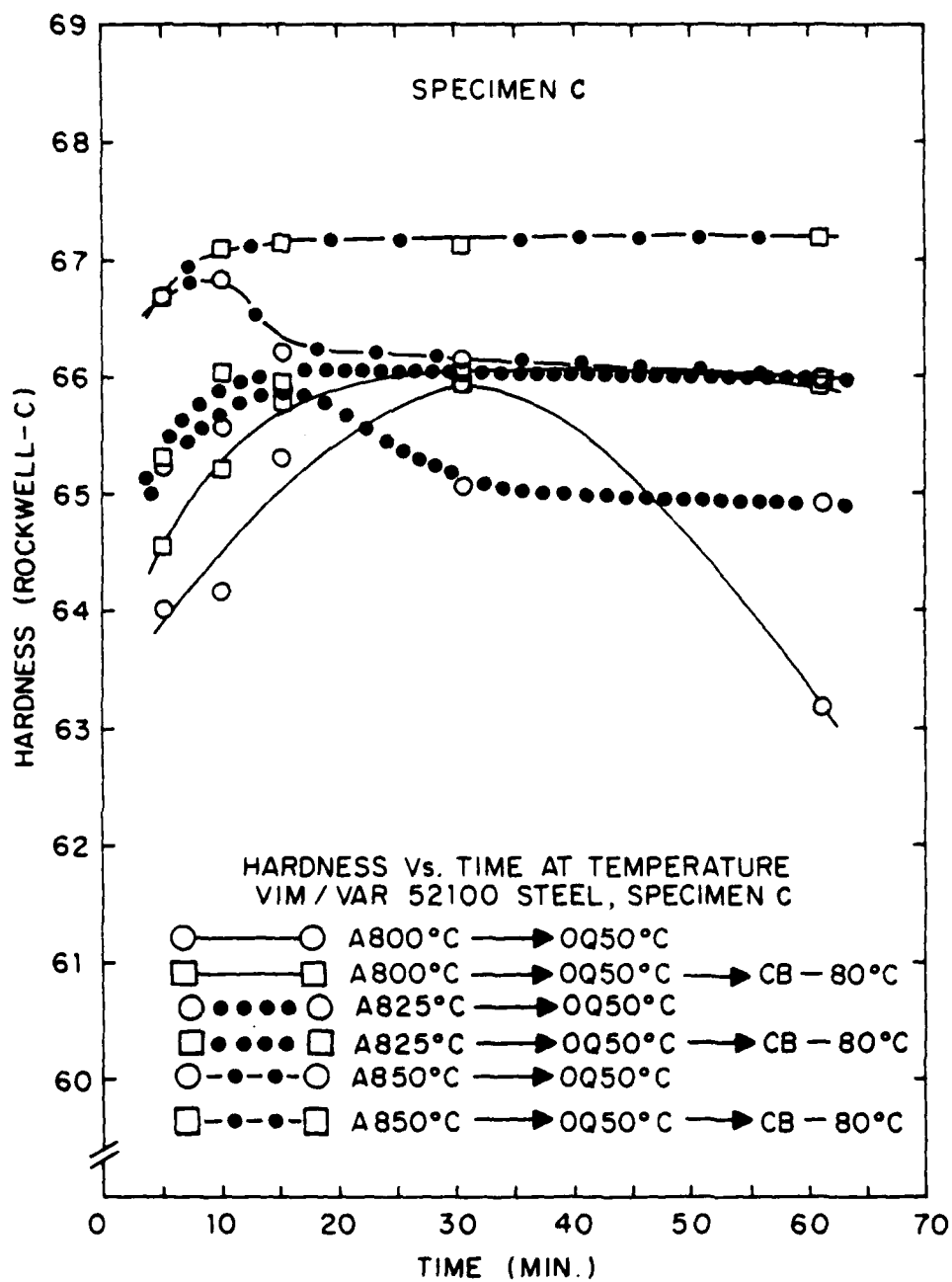
Figure 26. Hardening Response of Treatment-C
