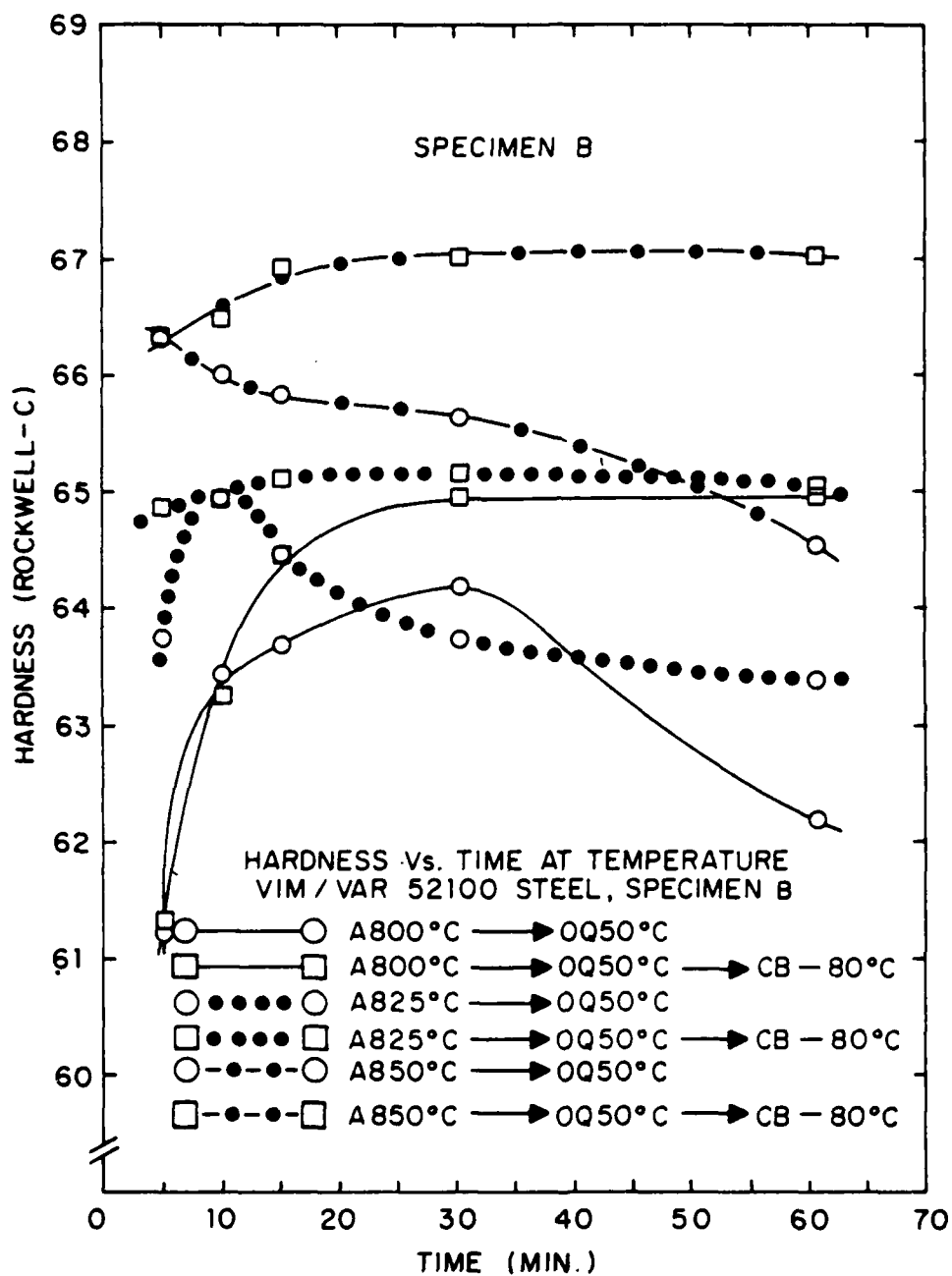
Figure 25. Hardening Response of Treatment-B
