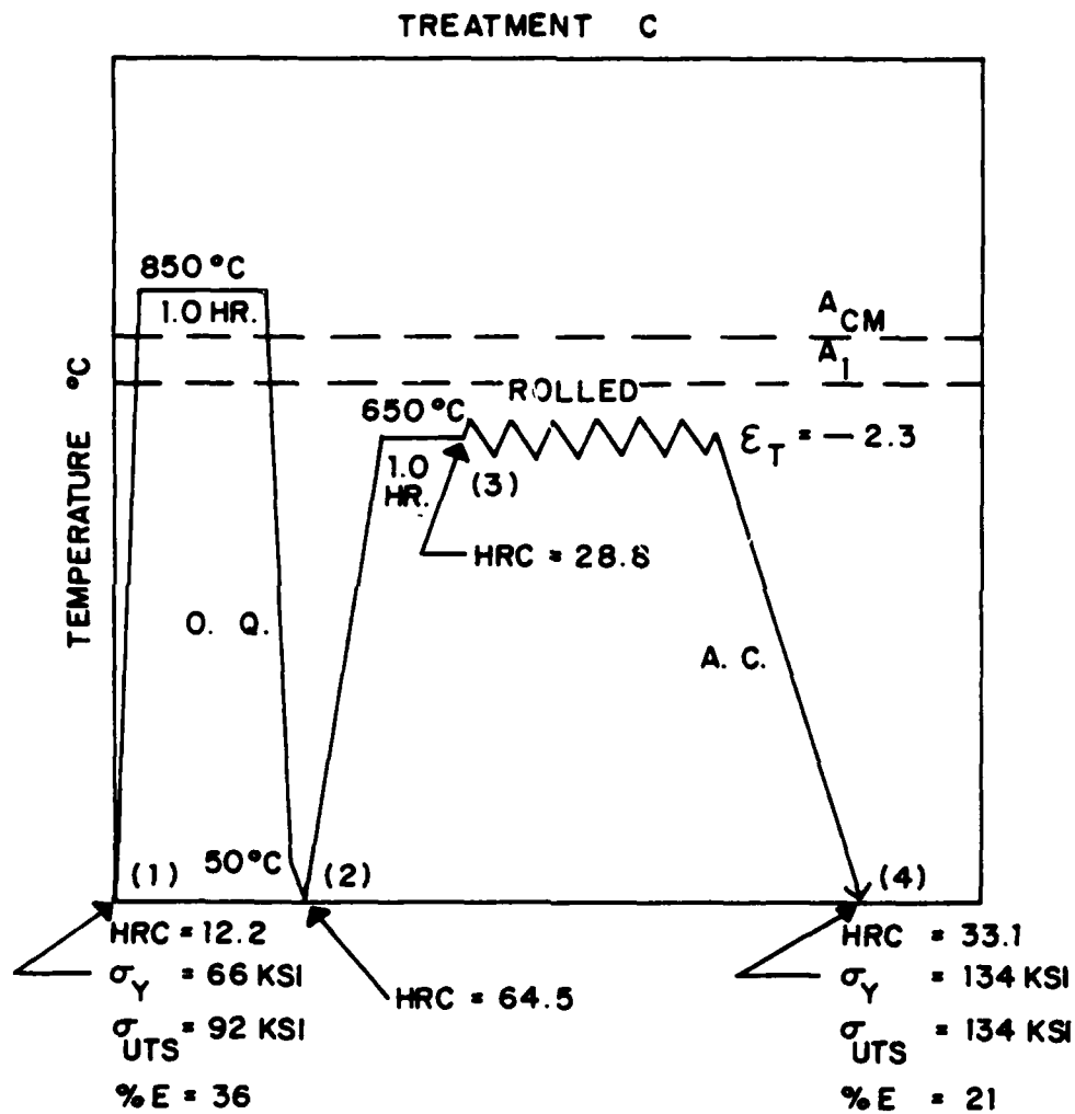
Figure 6. Schematic of Thermo-Mechanical Treatment-C.
