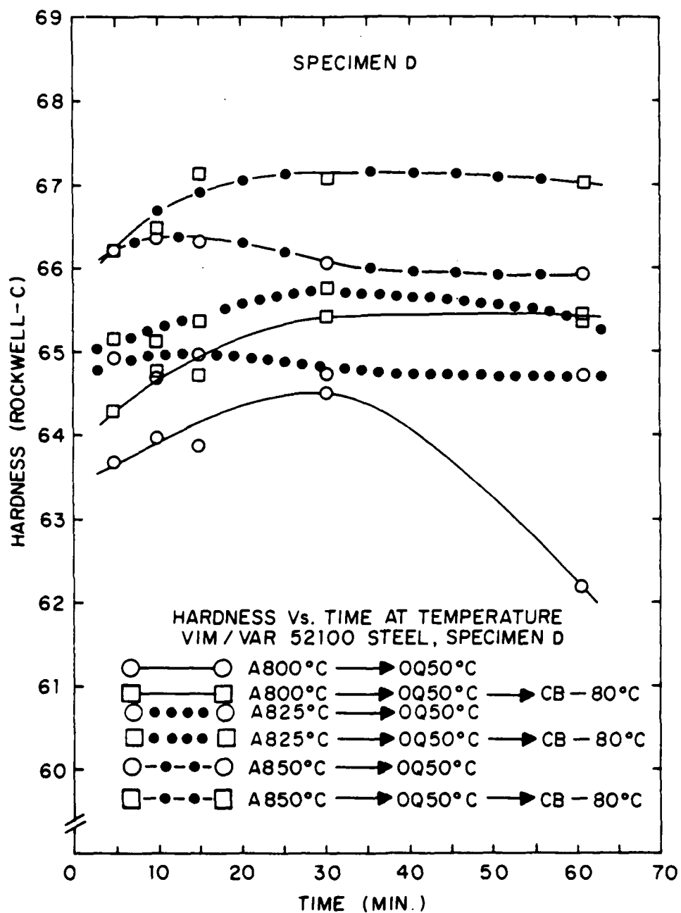
Figure 27. Hardening Response to Treatment-D
