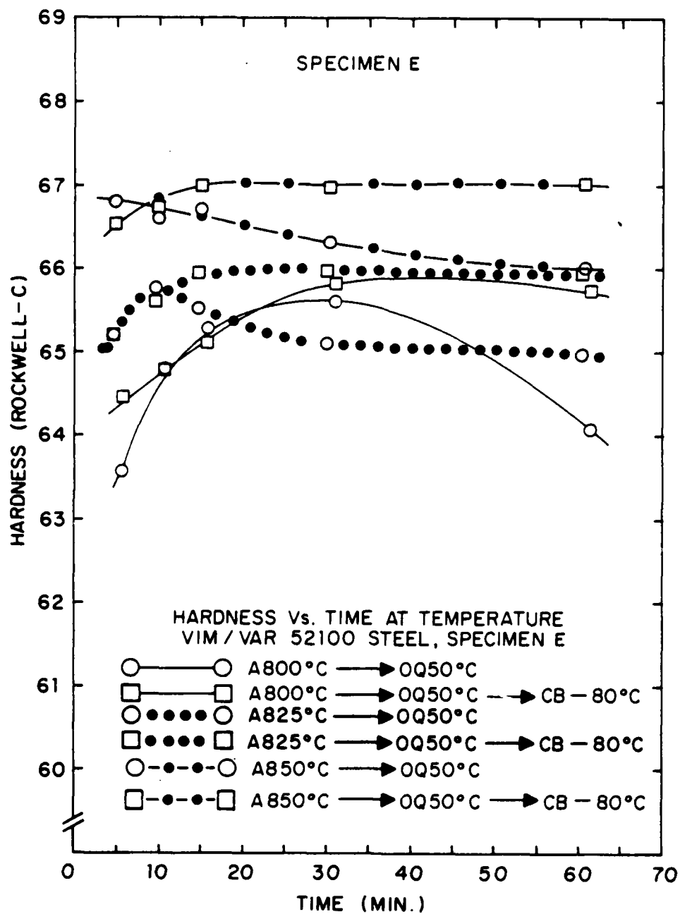
Figure 28. Hardening Response of Treatment-E
