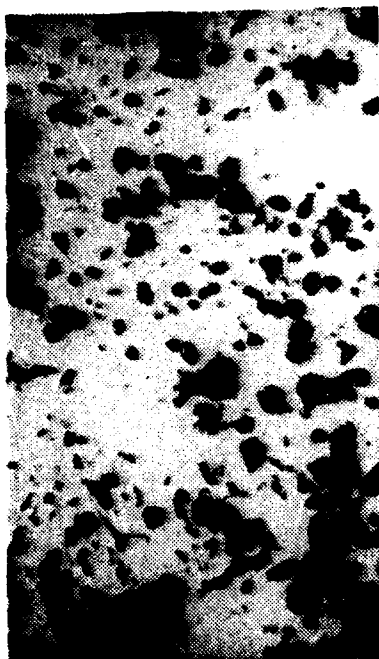
Figure 20. Carbon Extraction Micrograph of Treatment-D (prior to rolling): (a) Magnification 5,000X; (b) Magnification 10,000X; (c) Magnification 15,000X. Structure shows distribution of carbides.
