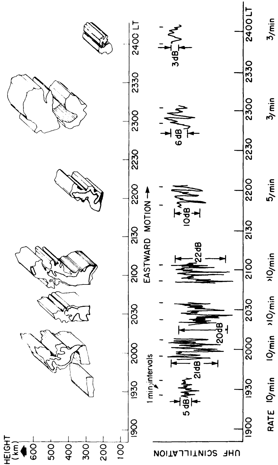
Figure 3. Typical patch development with associated scintillation amplitude and rates. ( From Aarons 1,2 )
