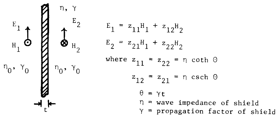
Figure 7. Two-port Impedance Representation
