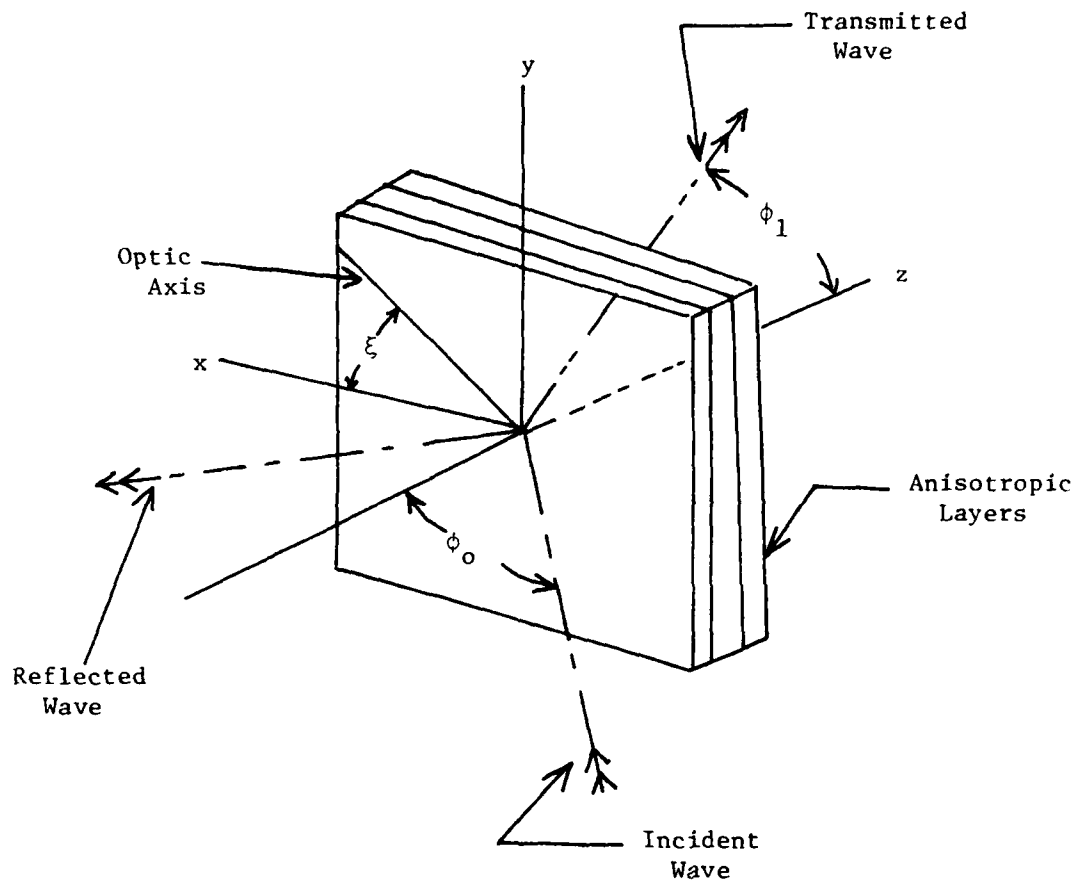
Figure 23. Multilayer Anisotropic Shield with Incident Plane Wave at Arbitrary Angle of Incidence. Shield Infinite in Extent in xy -Plane. Plane of Incidence is the xz -Plane.
