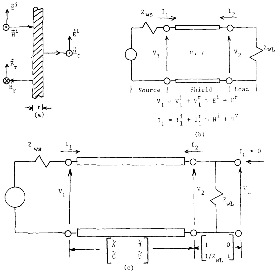
Figure 3. a) Elementary Plane Wave Shielding b) Transmission Line Analogy c) ABCD Parameter Representation
