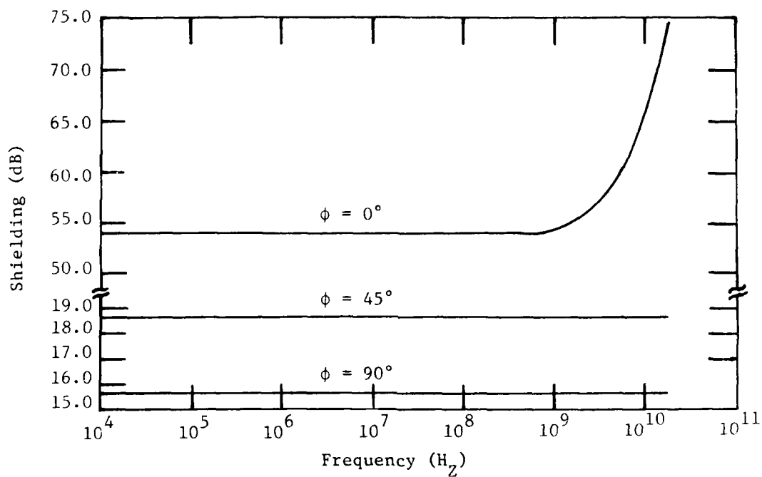
Figure 21. Shielding effectiveness of a single layer anisotropic shield for various fiber orientations. A plane wave polarized in the \phi = 0^\circ direction is normally incident on the input side of the shield, shield parameters are t = .00525 inches, \sigma = 2 \times 10^4 mhos/m, \sigma_2 = 2 \times 10^2 mhos/m, \epsilon_{r1} = \epsilon_{r2} = 3 .
