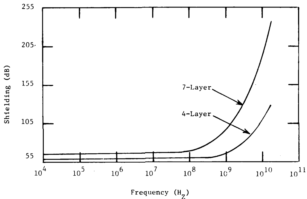
Figure 22. Shielding effectiveness of 4-layer and 7-layer anisotropic shields. Fiber orientations for 4-layer shield are (0^\circ, \pm 45^\circ, 90^\circ) ; for 7-layer shield are (0^\circ, \pm 45^\circ, 90^\circ, \pm 45^\circ, 0^\circ) . Each layer has t = .00525 inches, \sigma_1 = 2 \times 10^4 mhos/m, \sigma_2 = 2 \times 10^2 mhos/m, \epsilon_{r1} = \epsilon_{r2} = 3 .
