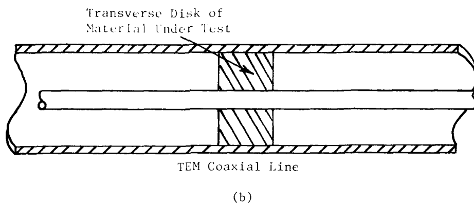
Figure 8. Two Types of Measurement Structures Included in the Generalized Analysis
