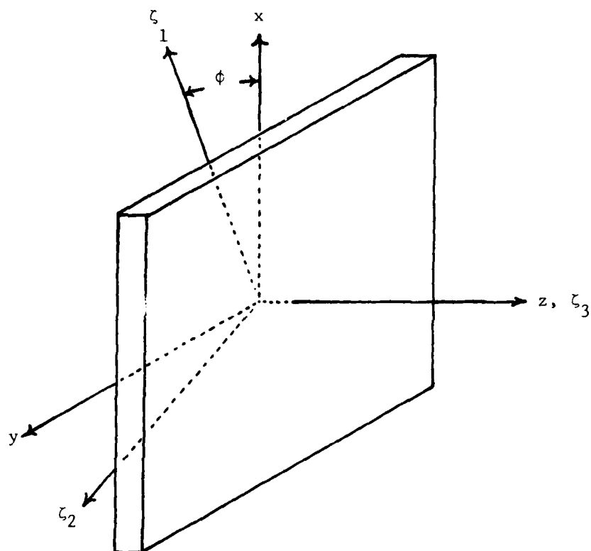
Figure 16. Propagation (x, y, z) and Material (\zeta_1, \zeta_2, \zeta_3) Coordinates for Treating Anisotropic Material with "OpticAxis" in z Direction.
