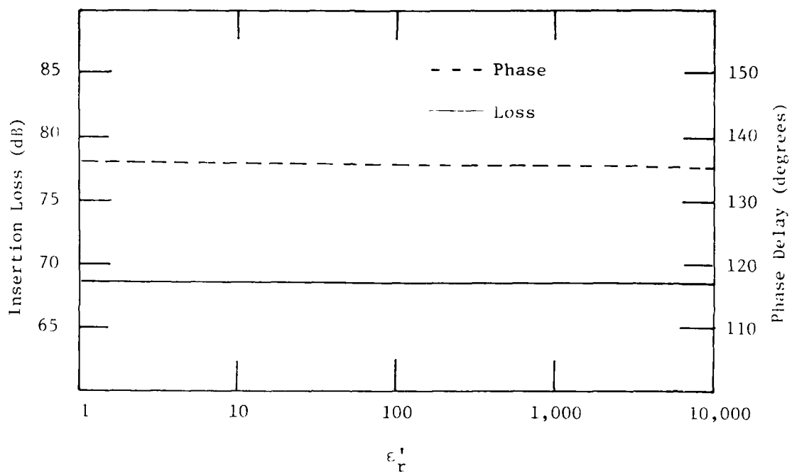
Figure 10. Insertion loss and phase delay for a lossy transverse slab in L-band rectangular waveguide, t = 0.02 inches, \sigma = 10^4 mhos/m. Loss and phase are both essentially independent of \epsilon'_r .
