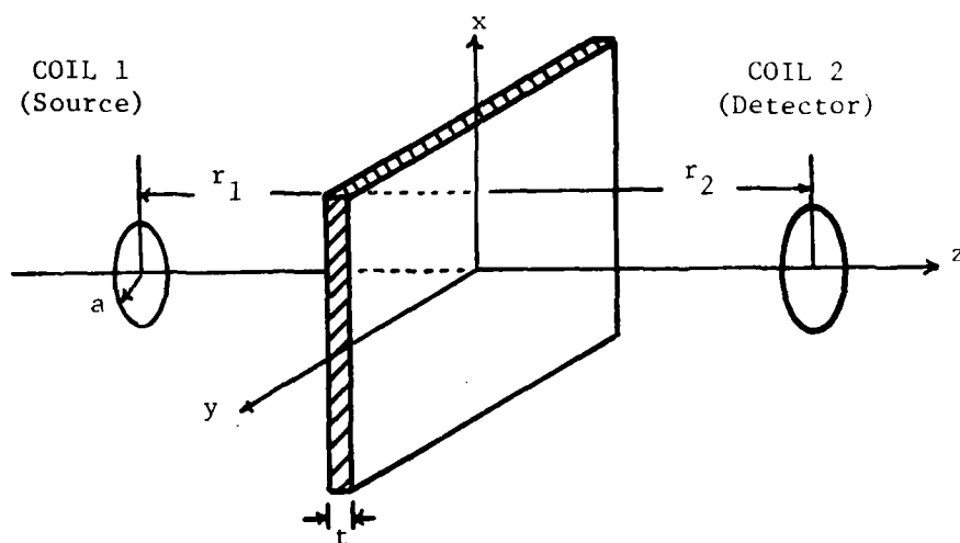
Figure 5. Two-loop/Infinite Flat Plate Configuration
