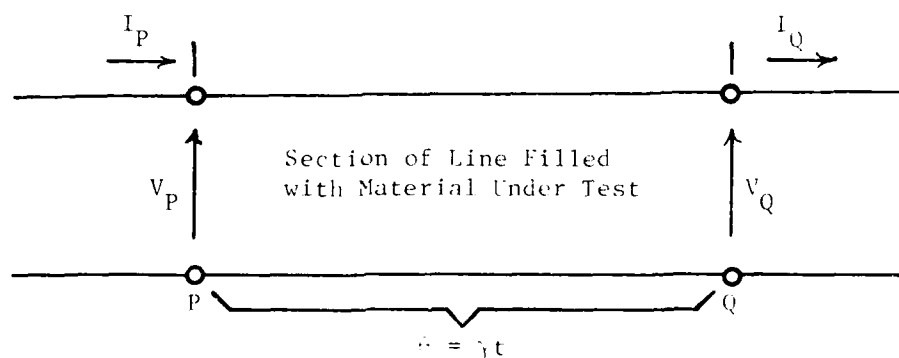
Figure 9. Generalized Transmission Line Model for Measurement Structure. Note: V_P = V_i + V_r , I_P = I_i - I_r .
