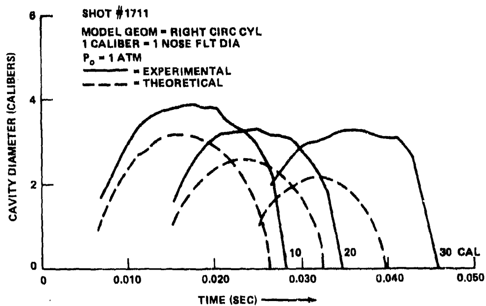
FIGURE 16 CAVITY DIAMETER AT VARIOUS DEPTHS VS TIME
