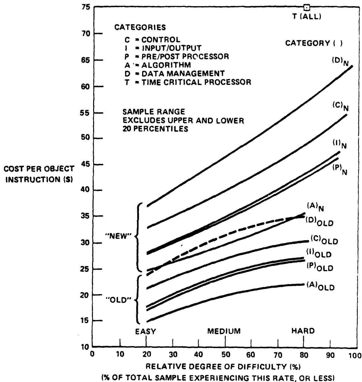
Figure A-7. Cost Per Object Instruction Versus Relative Degree of Difficulty
