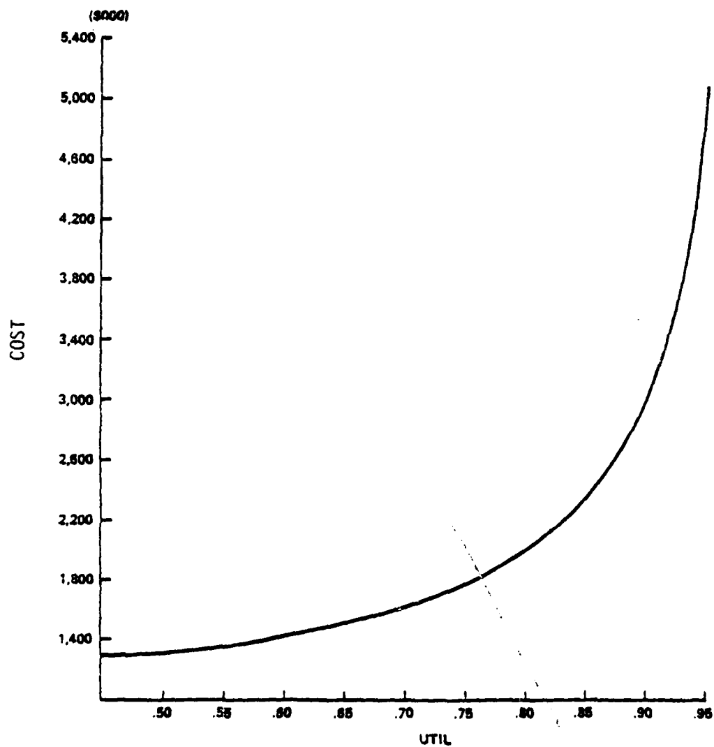
Figure A-6. Effect of UTIL on COST
