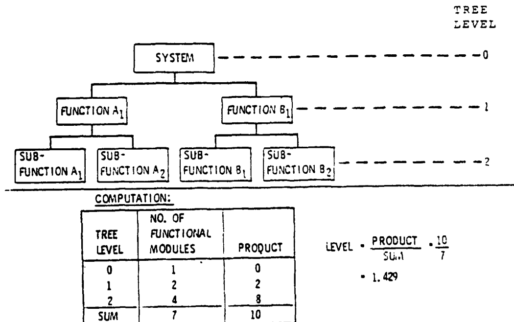
Figure A-5. Computation of LEVEL
