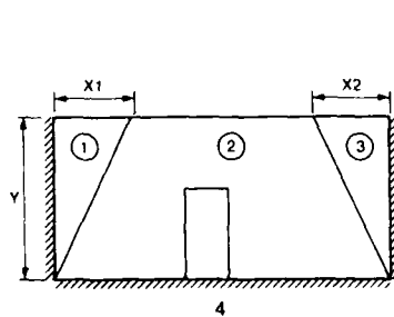
b. Three sides supported
