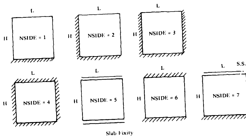
Figure 11a. Wall geometry
