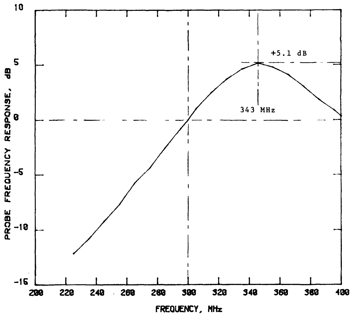
Fig. 24 Frequency Response of H-Field Probe
