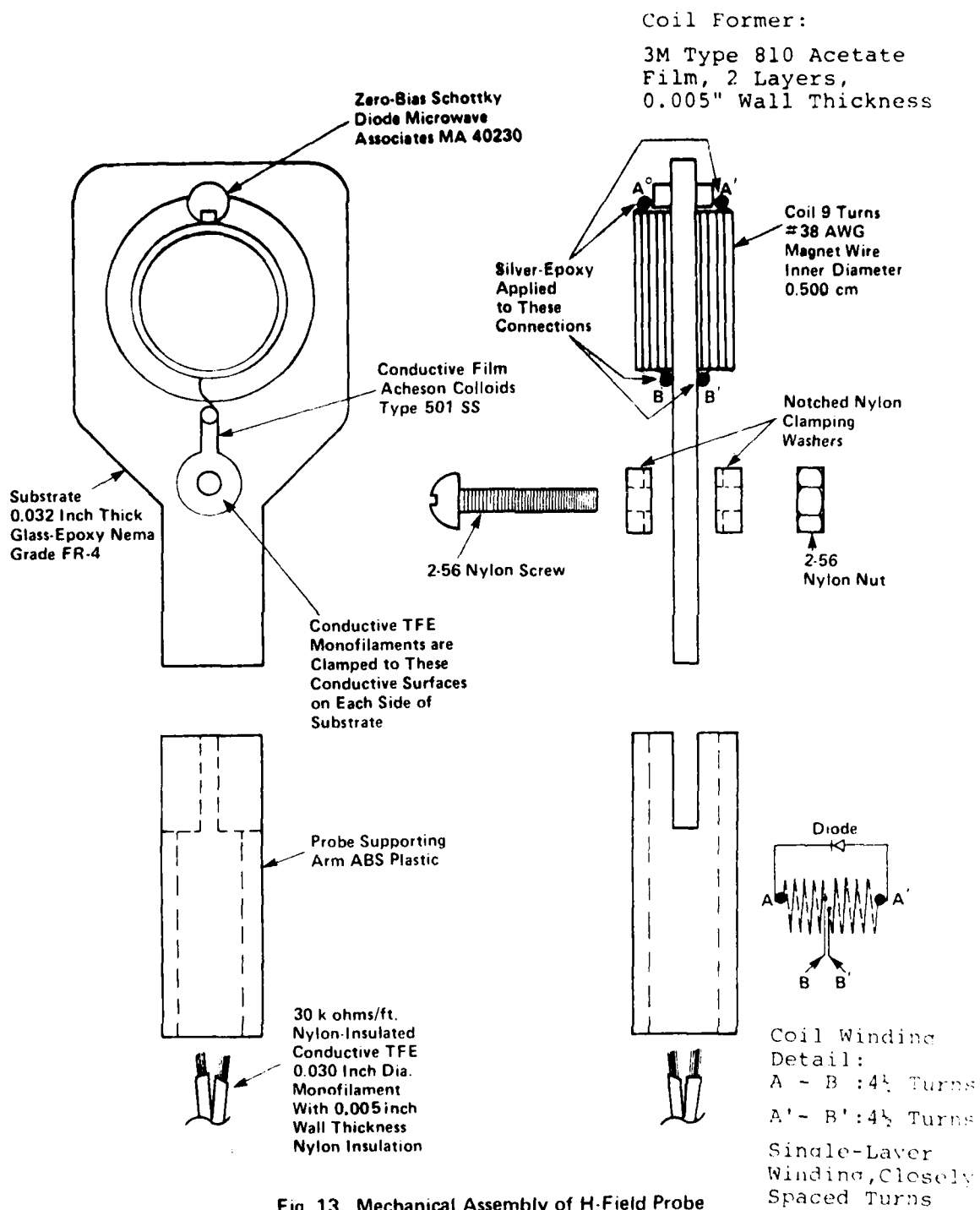
Fig. 13 Mechanical Assembly of H-Field Probe
