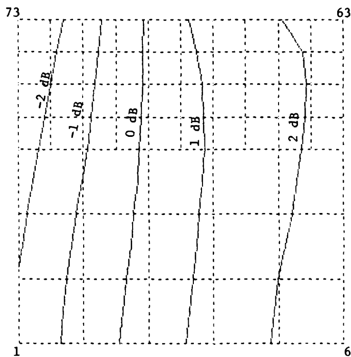
Figure B-11 CYLINDER MAP Hy
