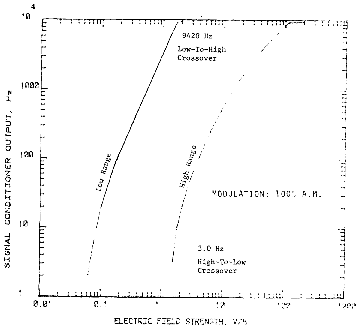
Fig. 19 Total Transfer Characteristic of Signal Conditioner and E-Field Probe
