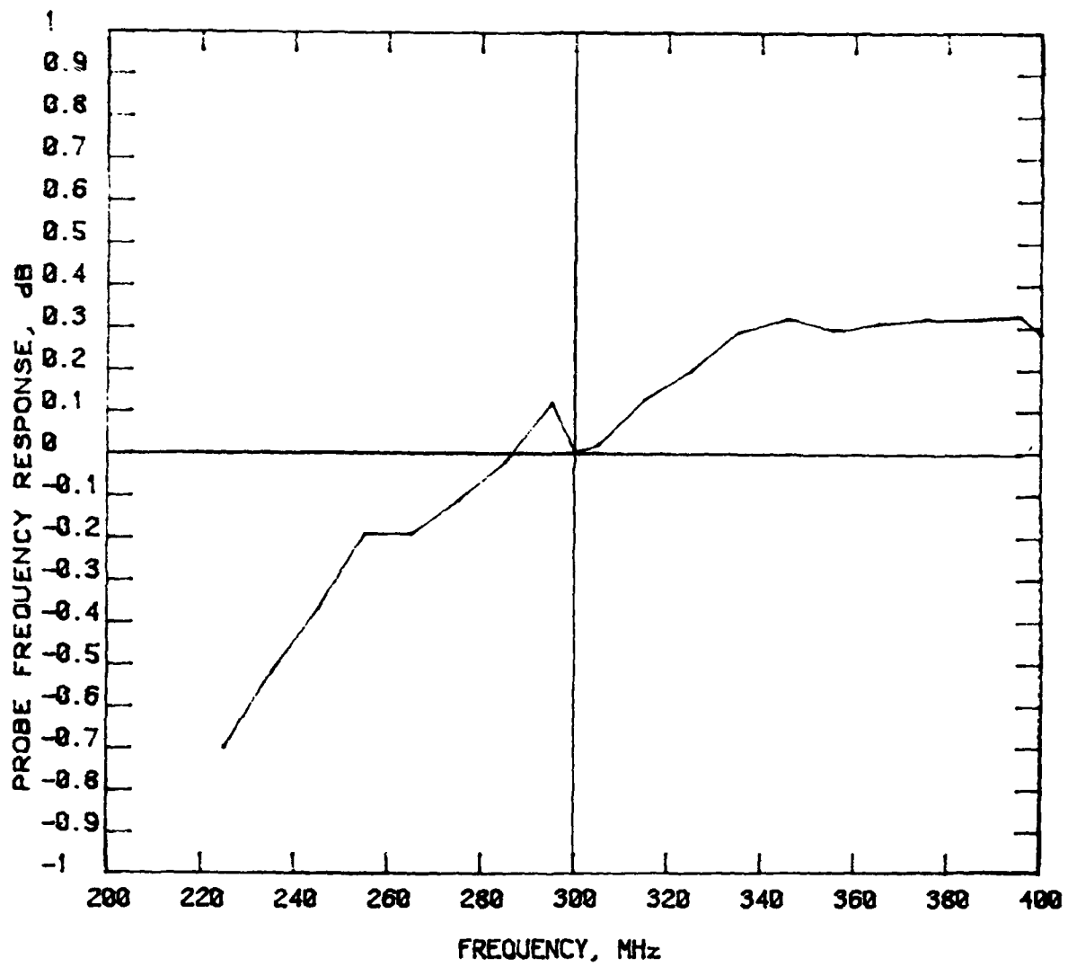
Fig. 22 Frequency Response of E-Field Probe
