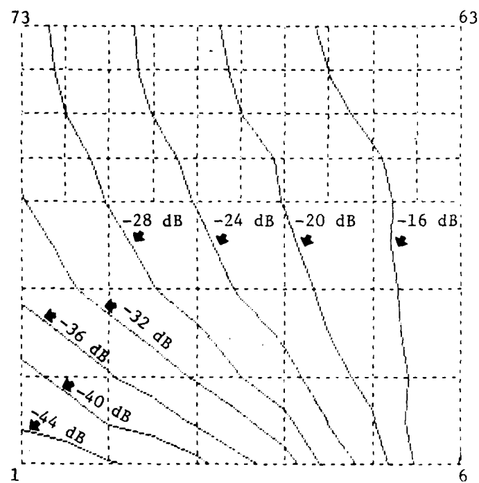
Figure B-28 NOSECONE MAP Hx
