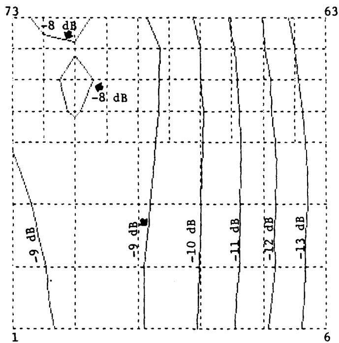
Figure B-23 NOSECONE MAP Hy
