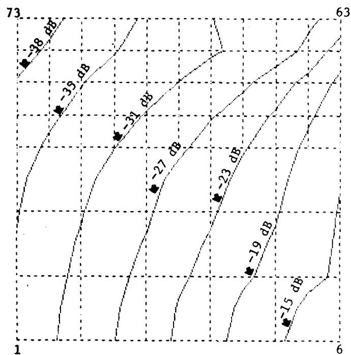
Figure B-31 NOSECONE MAP Ex
