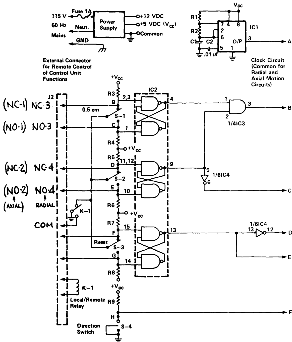
Fig. G-3 Sheet 1 of 4 Probe Position Control Unit
