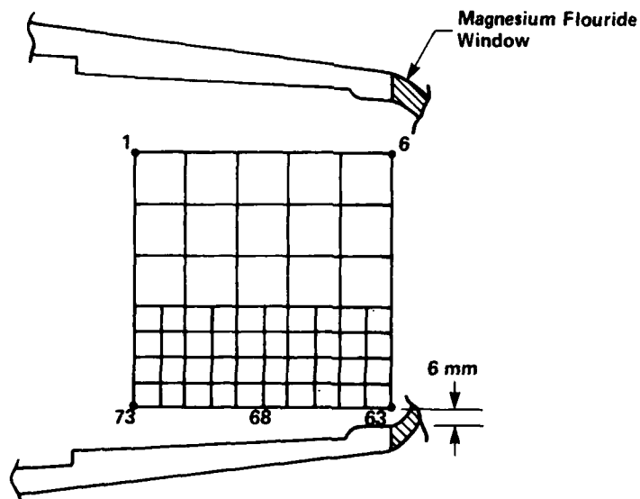
Fig. A-5 Scanning Grid Location Details for Missile Nosecone
