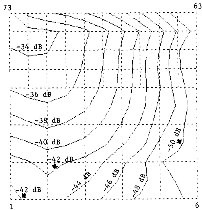
Figure B-20 NOSECONE MAP Ey
