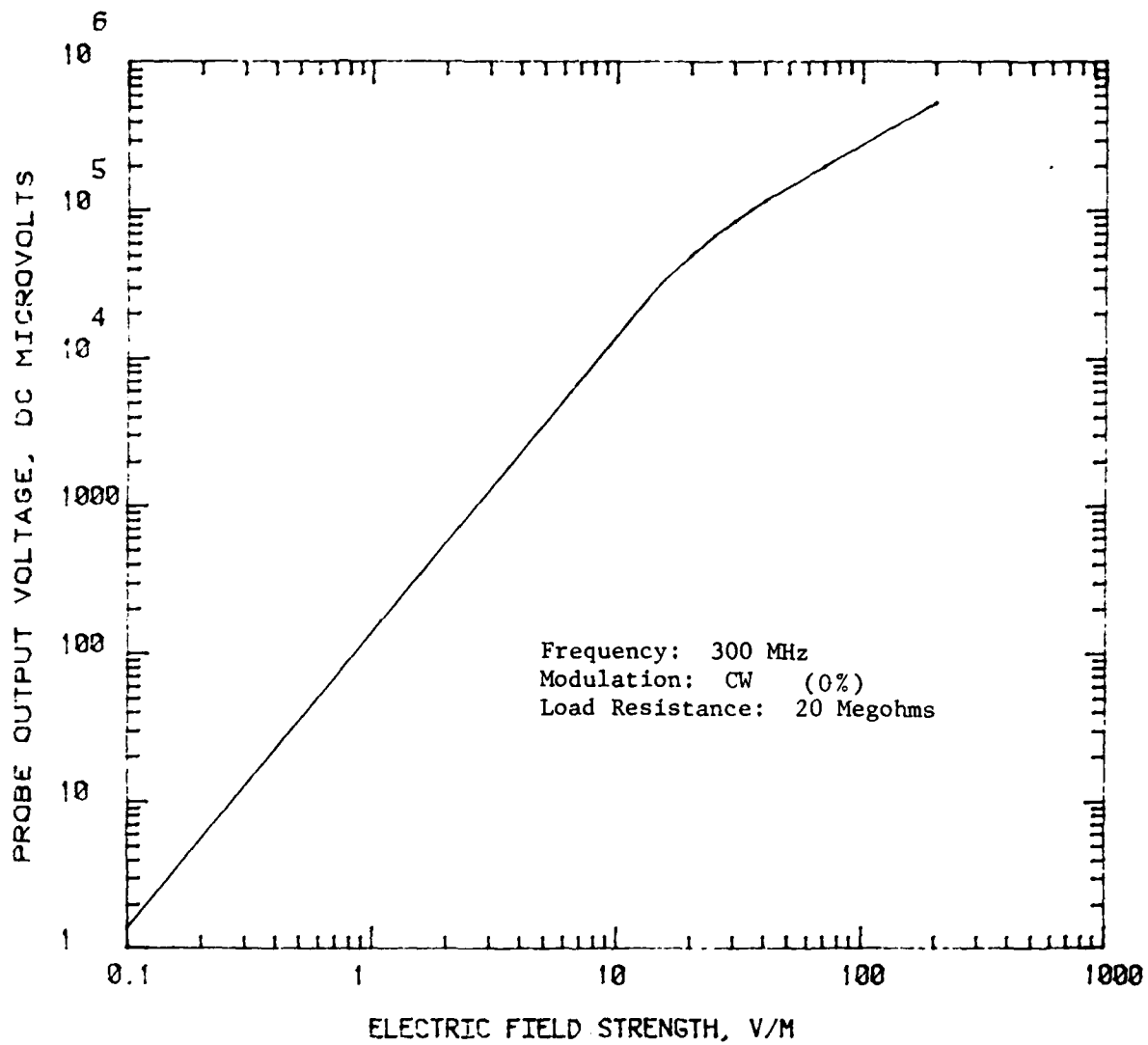
Fig. 10 DC Characteristics of E-Field Probe
