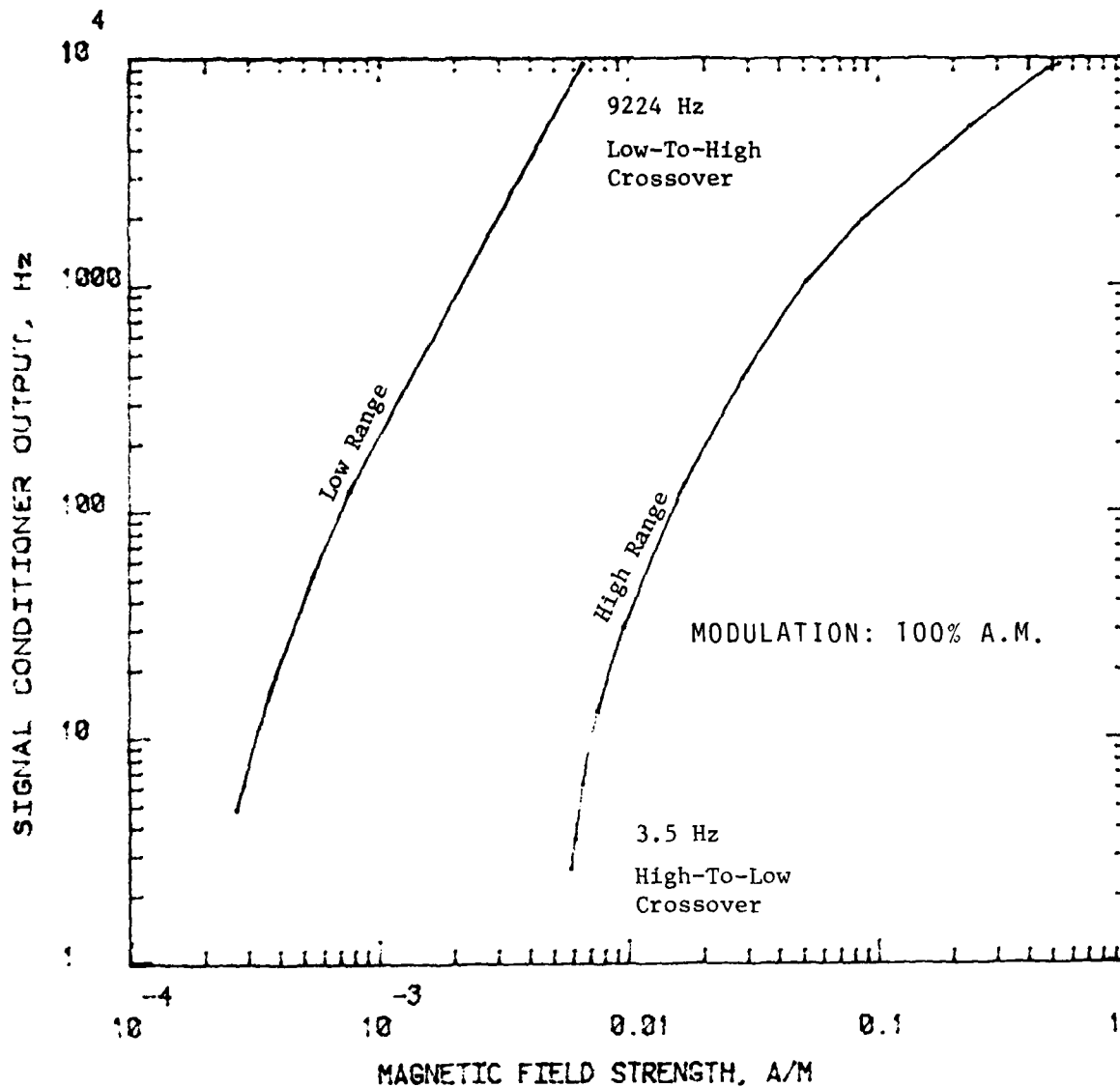
Fig. 20 Total Transfer Characteristic of Signal Conditioner and H-Field Probe
