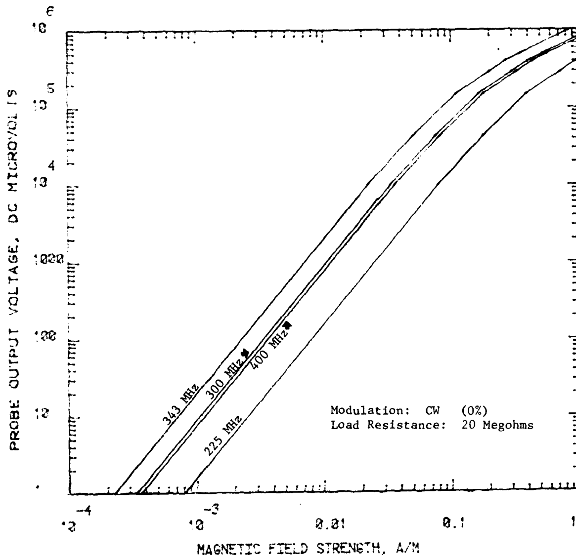
Fig. 14 DC Characteristic of H-Field Probe
