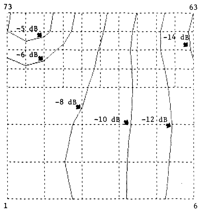
Figure B-17 NOSECONE MAP Hy
