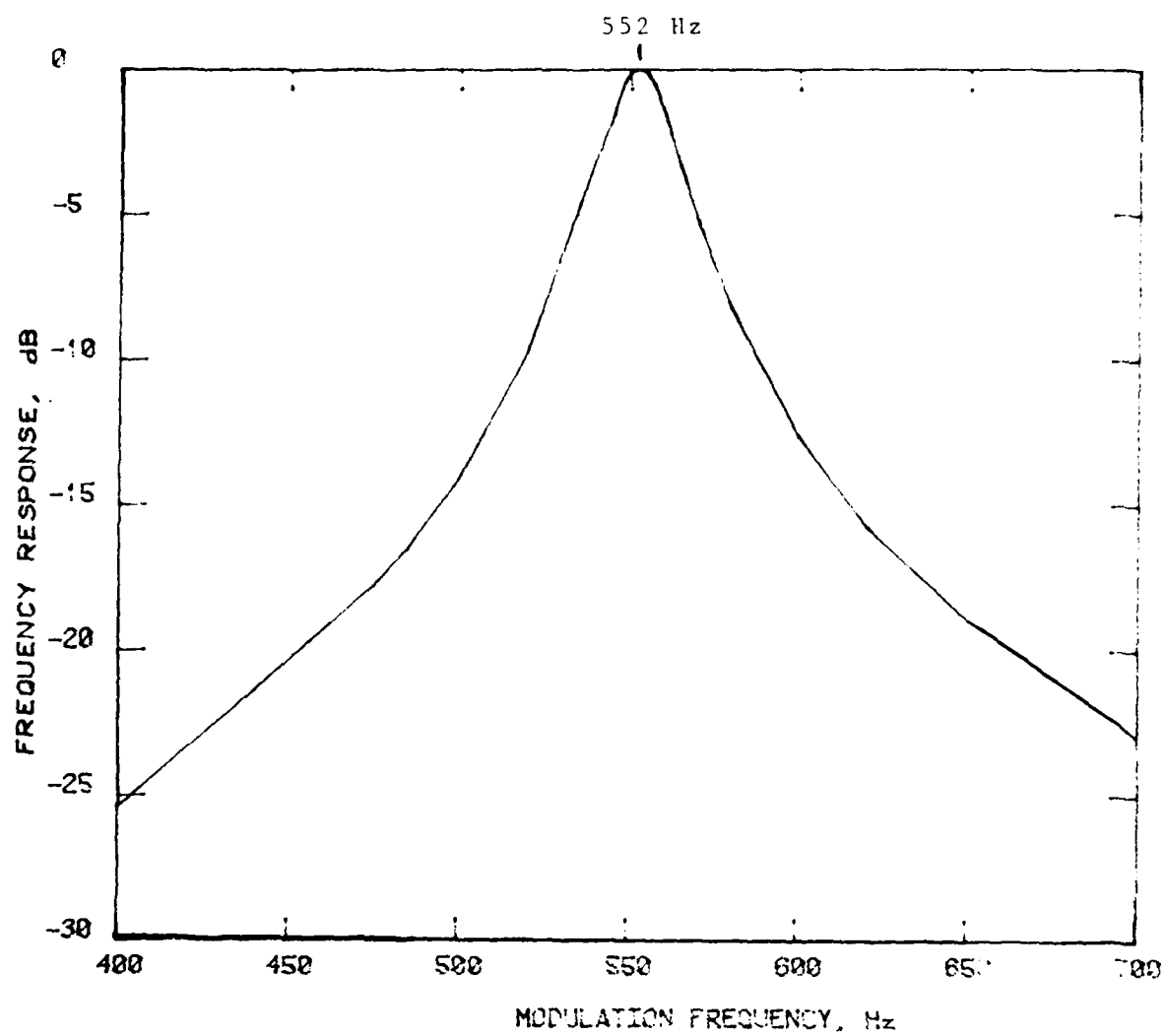
Fig 18 Frequency Response of Signal Conditioner
