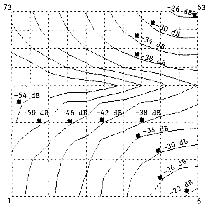
Figure B-26 NOSECONE MAP Ey
