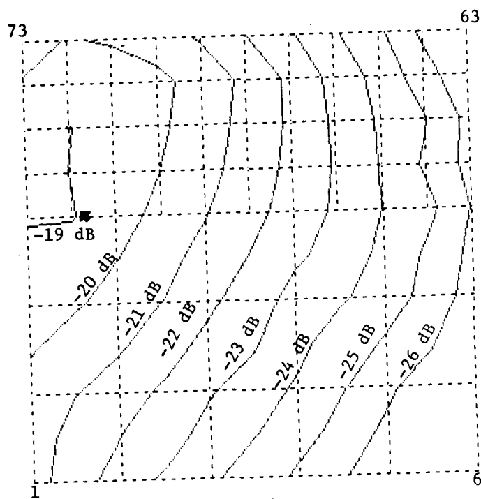
Figure B-22 NOSECONE MAP Hx
