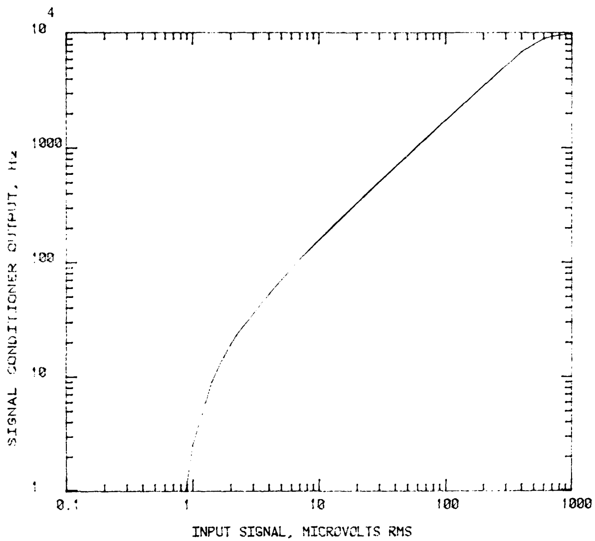
Fig. 17 Transfer Characteristic of Signal Conditioner
