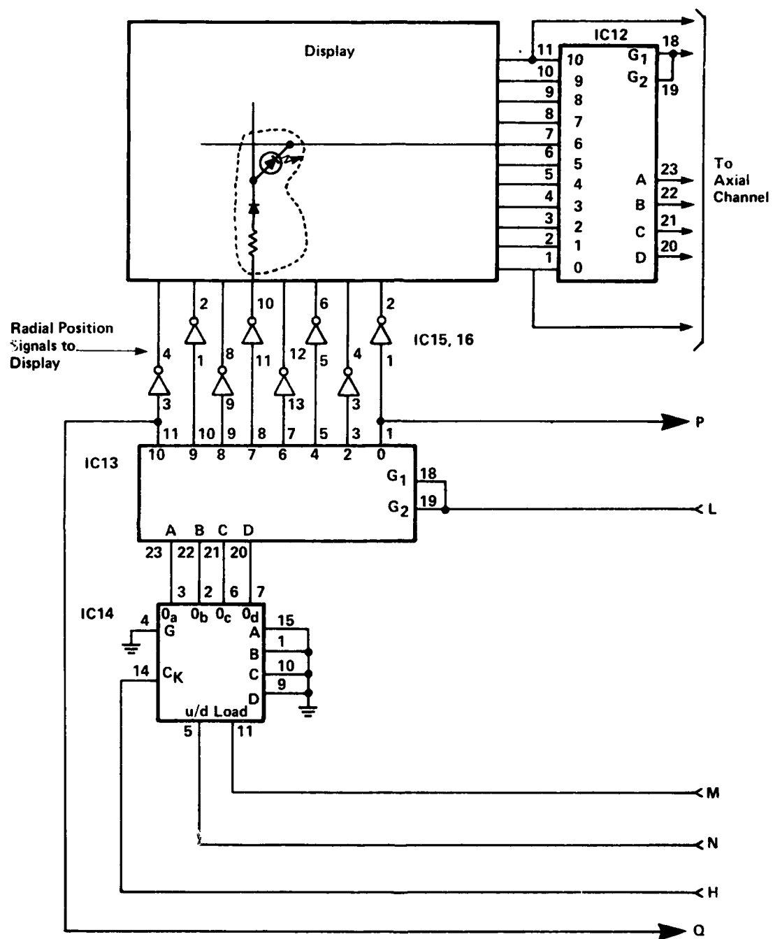
Fig. G-3 Sheet 3 of 4 Probe Position Control Unit
