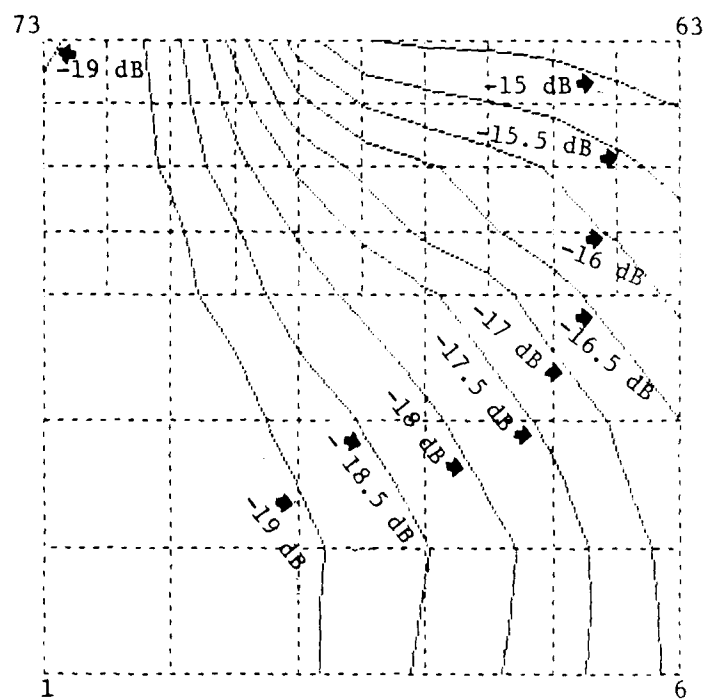
Figure B-4 CYLINDER MAP Hx
