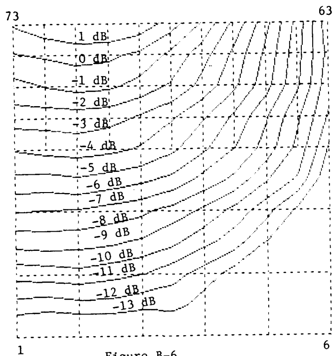
Figure B-6 CYLINDER MAP Hz
