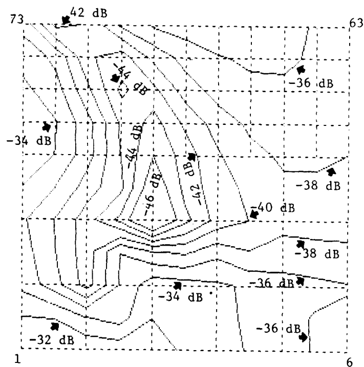
Figure B-16 NOSECONE MAP Hx
