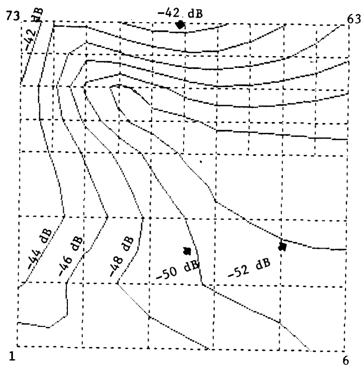
Figure B-14 NOSECONE MAP Ey
