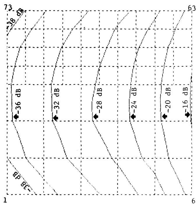
Figure B-25 NOSECONE MAP Ex
