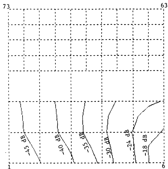
Figure B-33 NOSECONE MAP Ez
