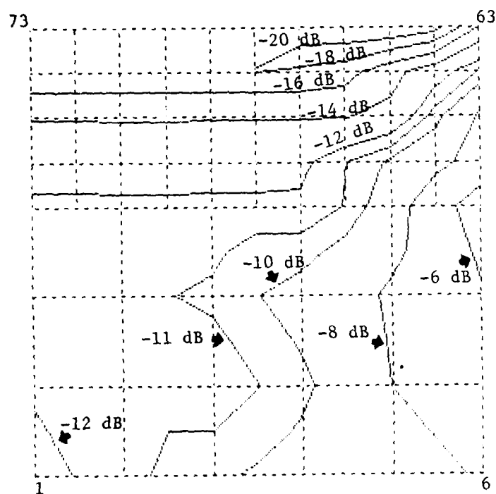
Figure B-9 CYLINDER MAP Ez
