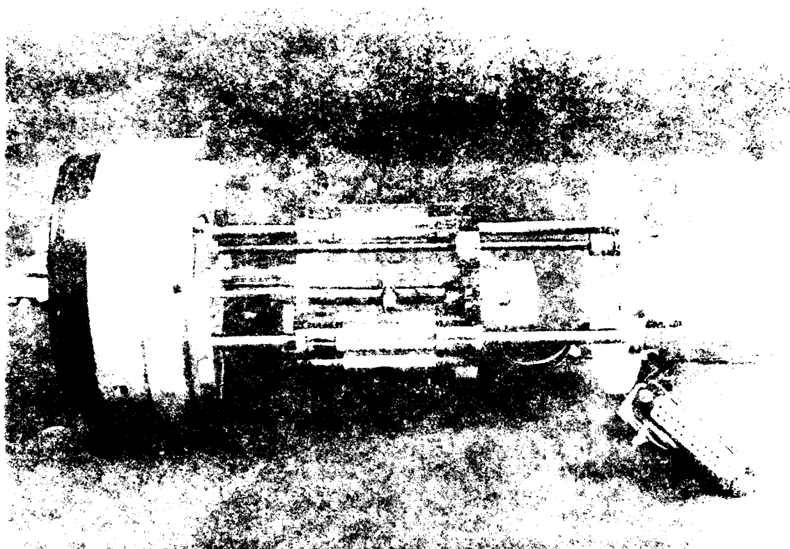
Fig. 3 View of Mechanical Positioning Unit, Assembled to Nosecone Bulkhead
