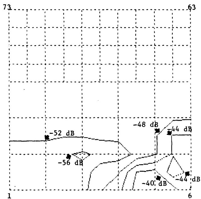
Figure B-27 NOSECONE MAP Ez
