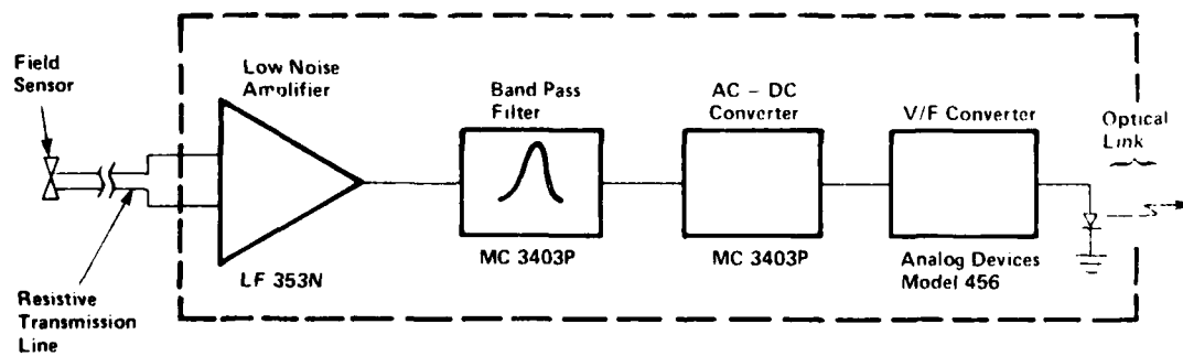
Fig. 16 Block Diagram of Signal Conditioner
