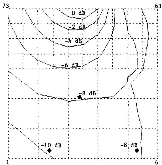
Figure B-7 CYLINDER MAP Ex
