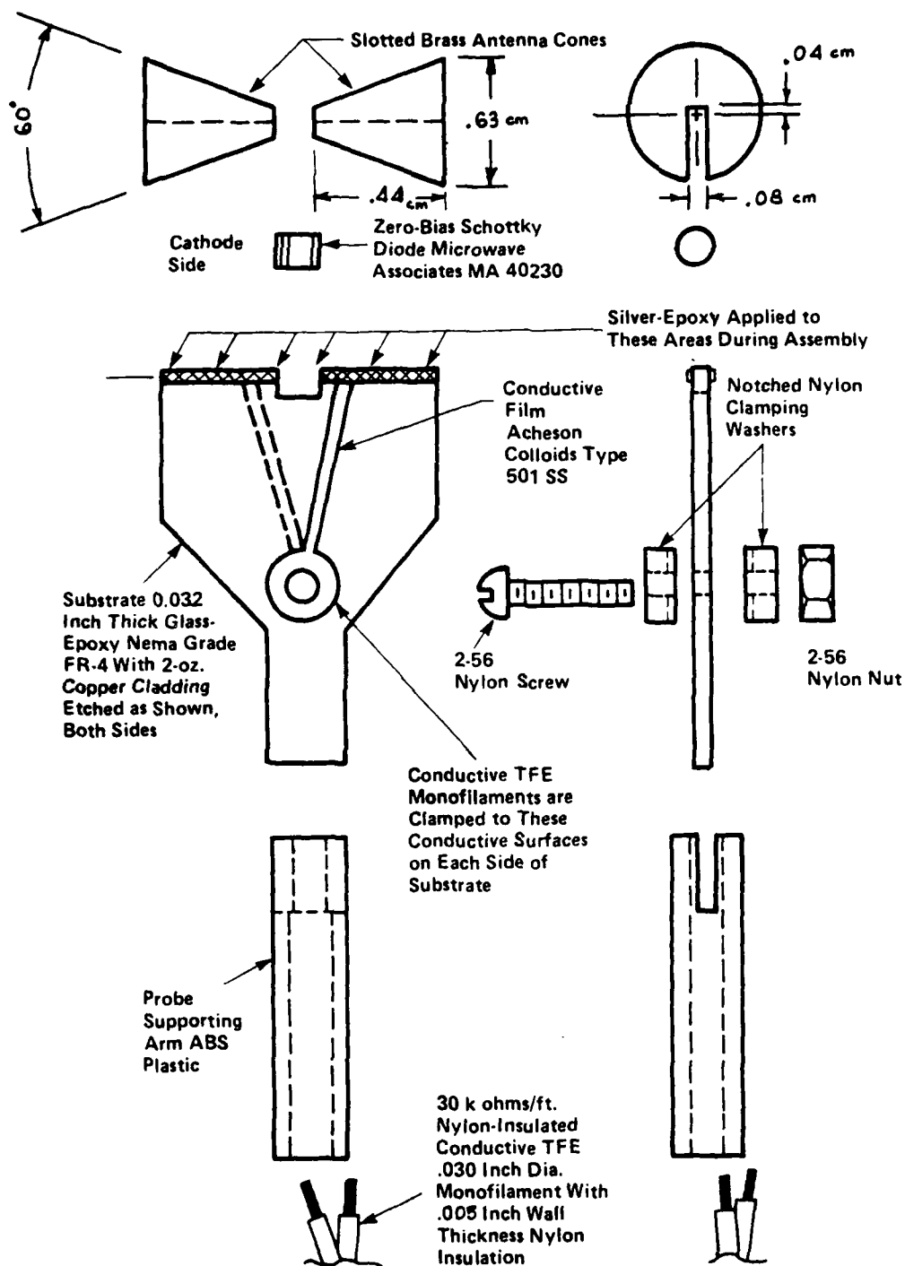
Fig. 9 Mechanical Assembly of E-Field Probe
