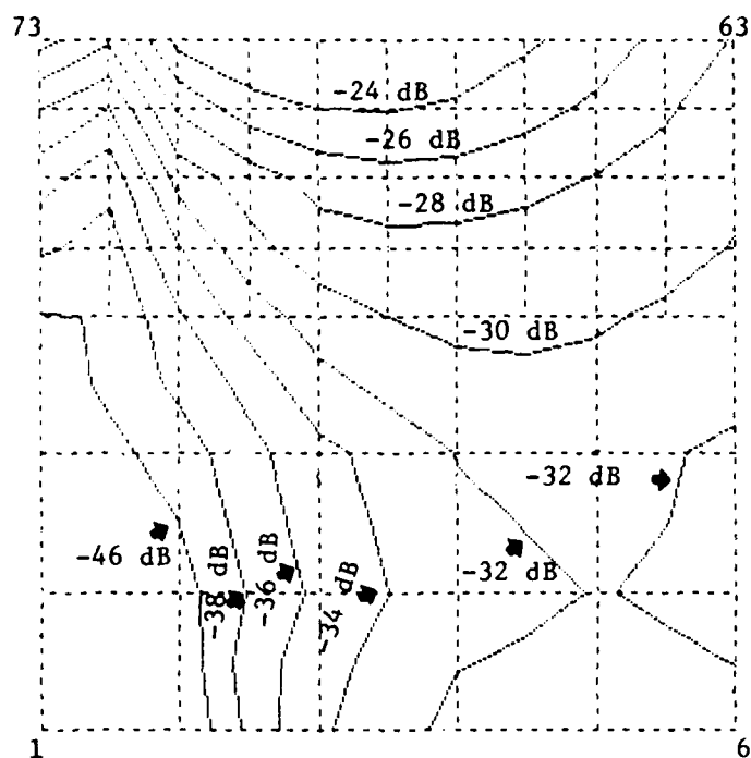
Figure B-19 NOSECONE MAP Ex
