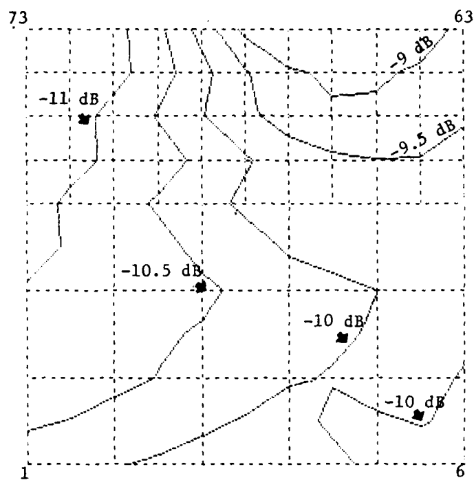
Figure B-3 CYLINDER MAP E_z
