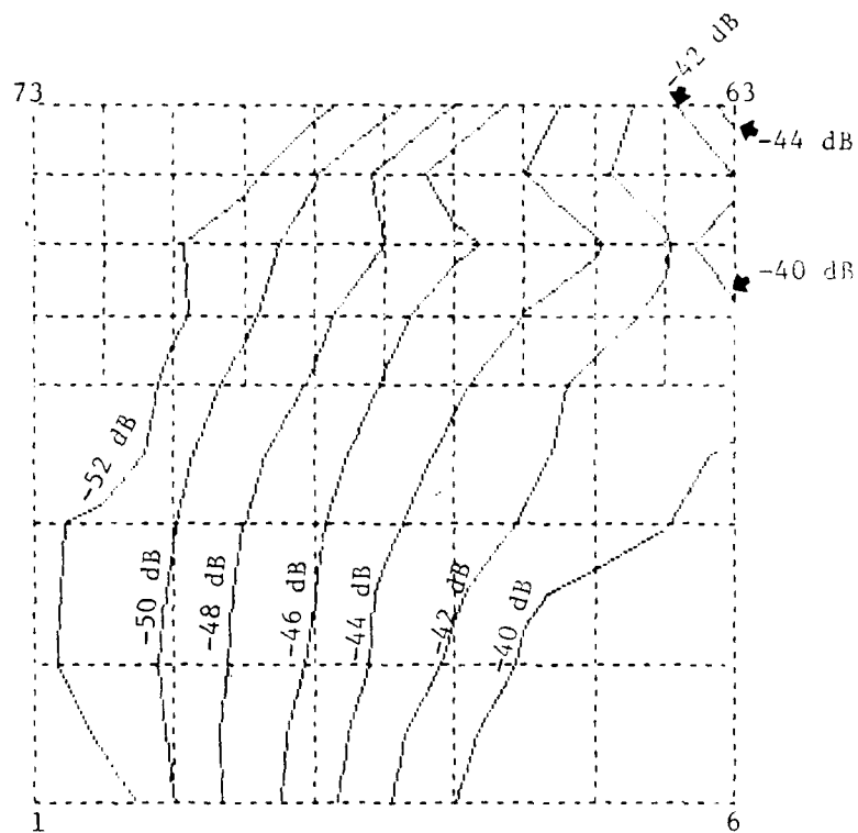
Figure B-32 NOSECONE MAP Ey
