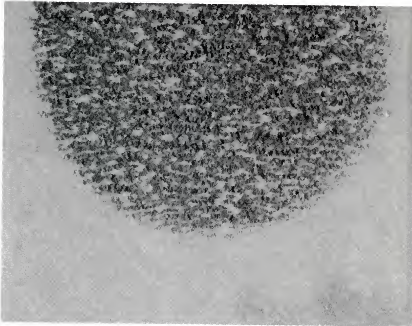
Figure 3. Lustrik, Low-Temperature Hardcoat, 2.6 mils — Porosity Test 9X: a. Not heated. b. Heated 56½ hours, 325° F.
