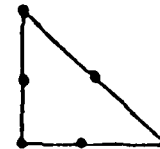
(ii) quadratic element
