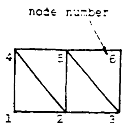
(i) Finite element solution graph
