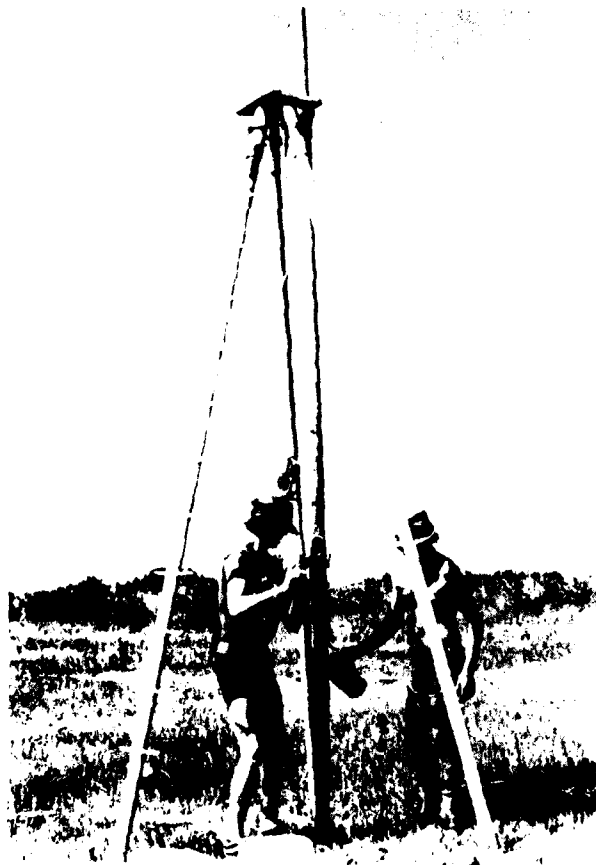
Figure 3. The 14-foot-high tripod with step supports welded to one leg. Extraction is accomplished with the use of two come-alongs attached to the headplate at the top of the tripod.
