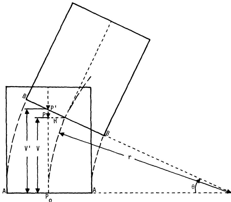
Figure C1. Illustration of effects on ground-motion displacement measurements due to rotational motion.
