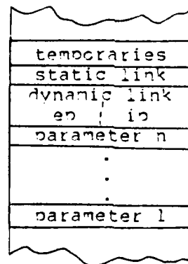
Figure 7. Activation Record Format
