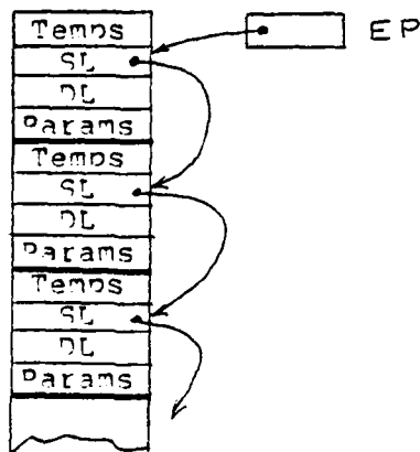
Figure 8. The Static Chain
