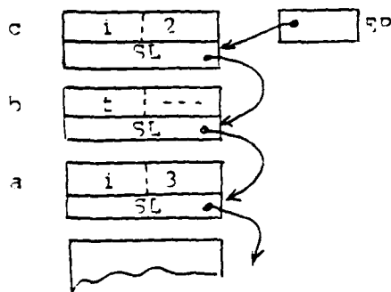
Figure 4. Before call to f
