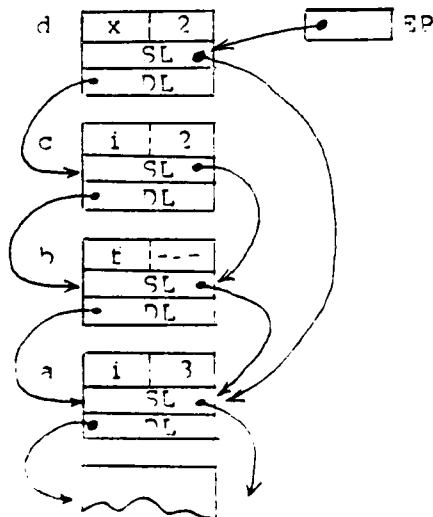
Figure 6. Inside f, with dynamic chain
