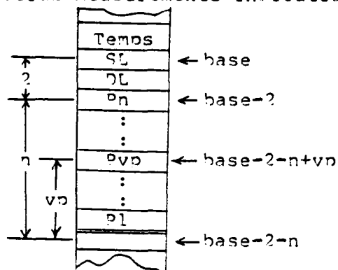
Figure 9. Activation Record Distances
