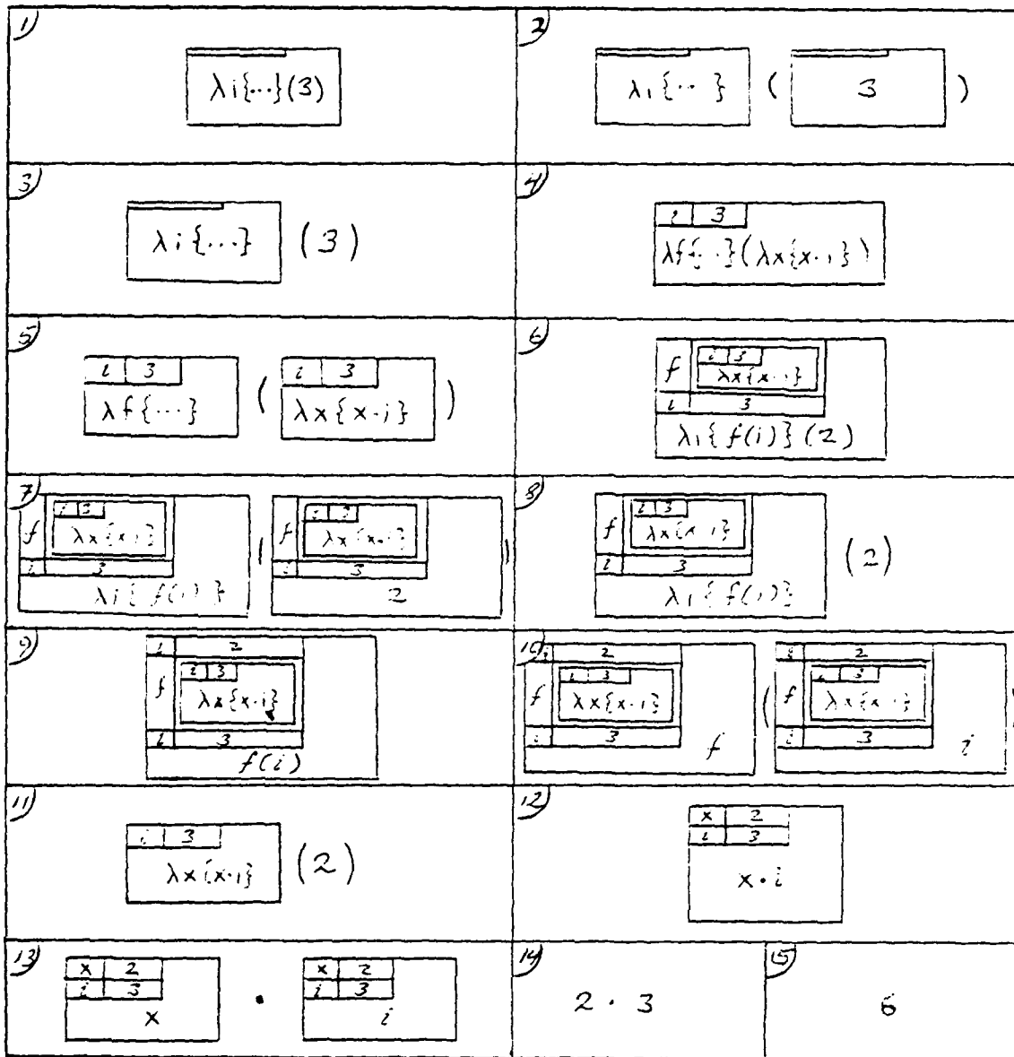
Figure 1. Example of Hand Evaluation
