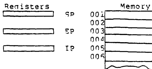
Figure 2. L-Machine Storage Architecture
