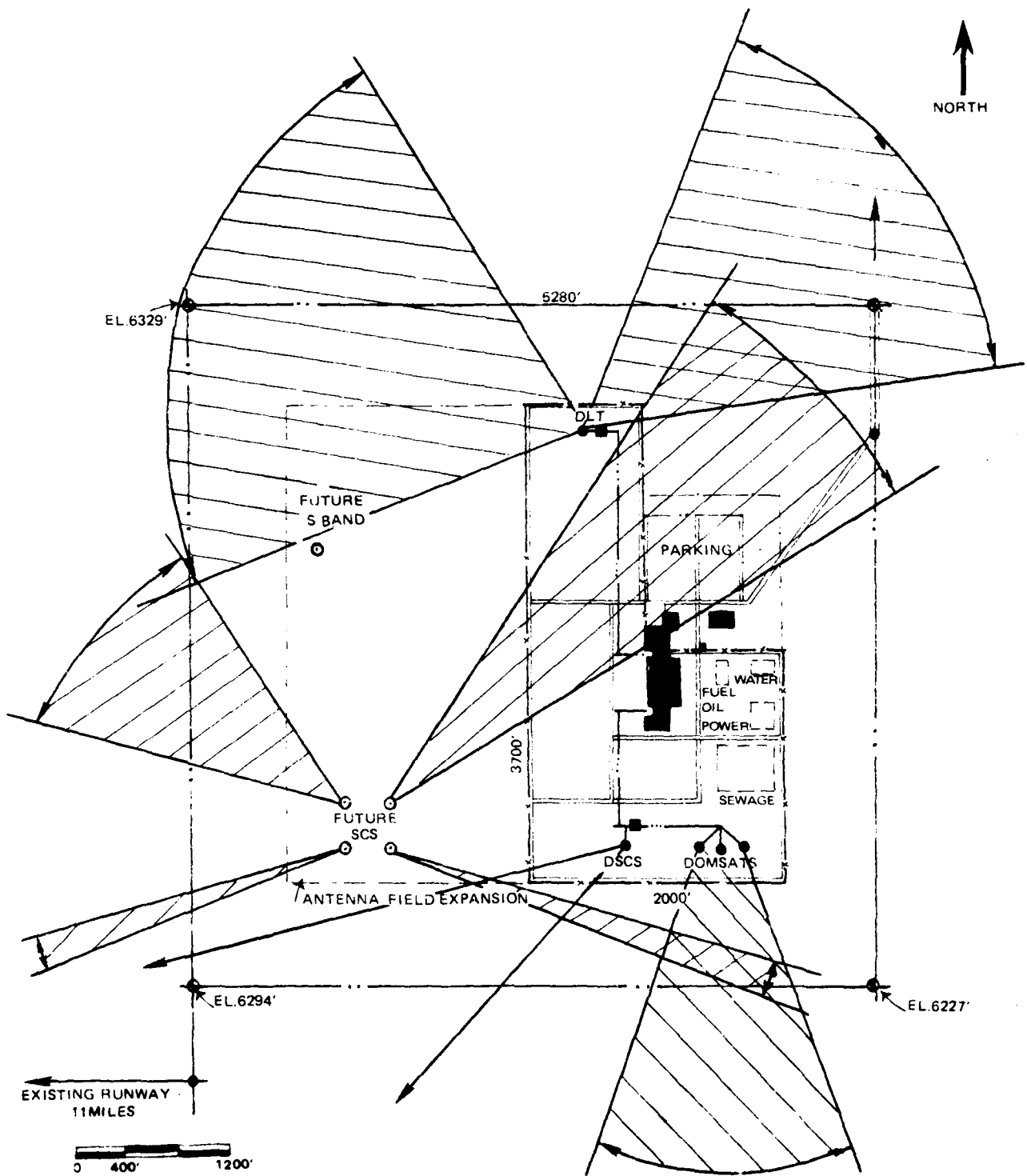
Figure 21 Antenna Layout on Section 24 at Peterson AFB/Colorado Springs Location
