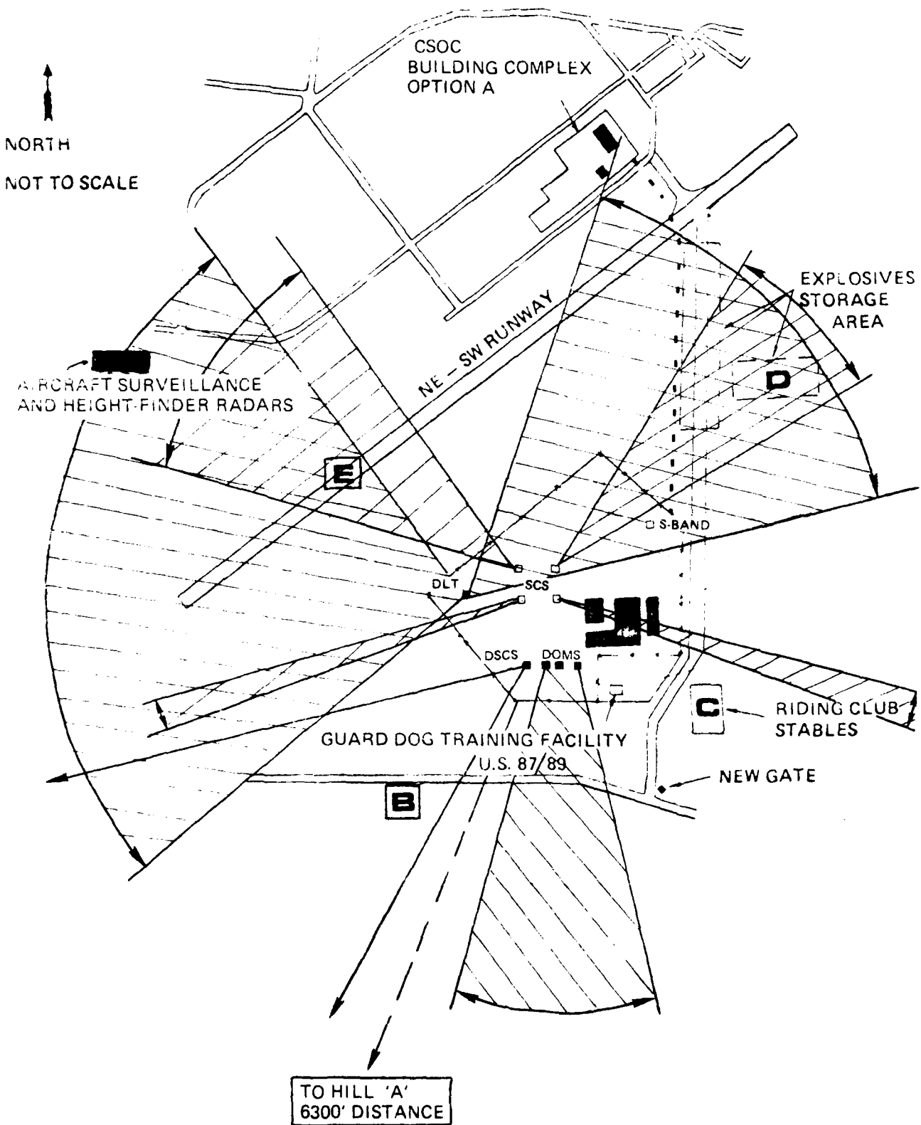
Figure 26 Antenna Layout at Malmstrom AFB IV-43
