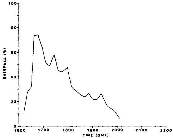
Figure 8. Contribution of Major Echo A to Total Estimated Rainfall
