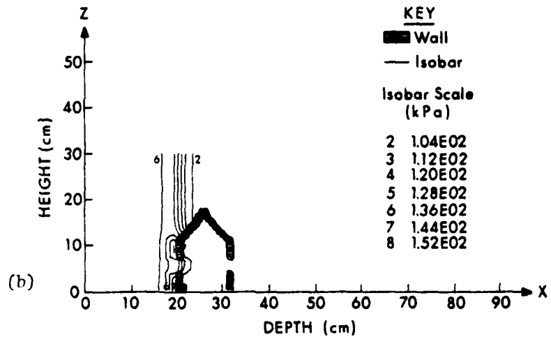
Figure 5. Isobars predicted at t = 0.23 ms; (a) Z = 5.3 cm, (b) Y = 29.8 cm.
