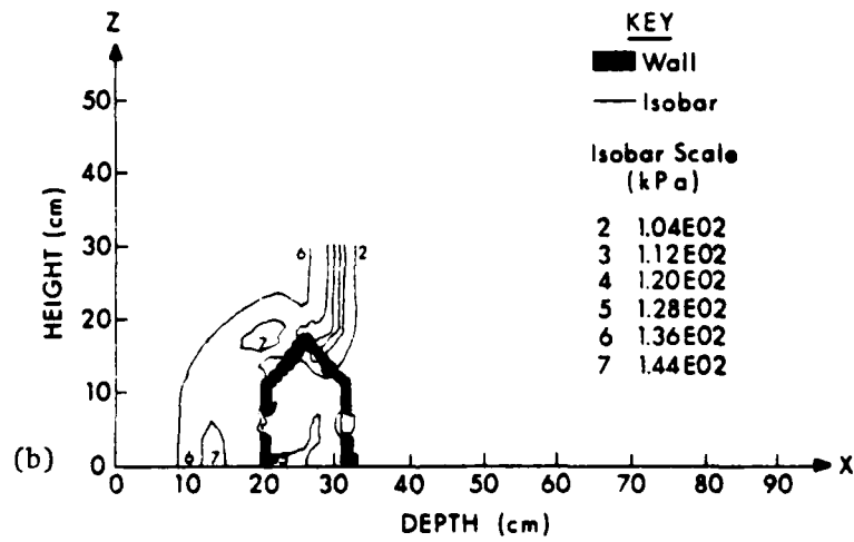
Figure 7. Isobars predicted at t = 0.38 ms; (a) Z = 5.3 cm, (b) Y = 29.8 cm.
