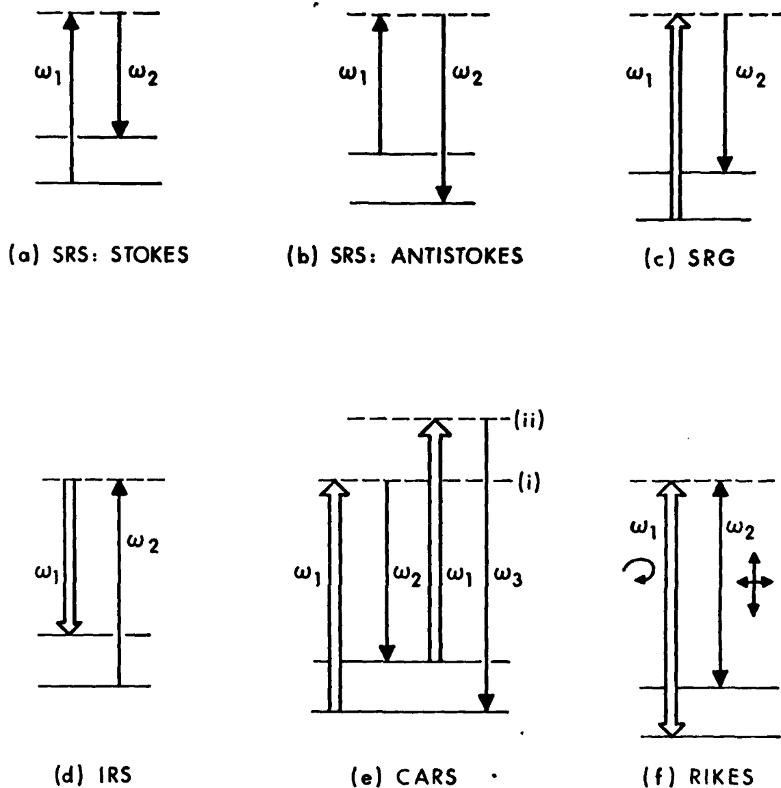
Figure 1. Transitions involved in different Raman processes. Solid lines indicate real levels, while dashed lines denote virtual states. (a) spontaneous Raman scattering in Stokes region; (b) spontaneous Raman scattering in anti-Stokes region; (c) stimulated Raman gain; (d) inverse Raman spectroscopy; (e) coherent anti-Stokes Raman spectroscopy; (f) Raman-induced Kerr effect spectroscopy. For the coherent Raman techniques (c) - (f), the stronger (pump) laser is designated by a broad, open arrow and the probe laser is shown as a thin arrow. In RIKES, (f), the pump laser is circularly polarized, and the probe laser is linearly polarized. Signal at \omega_2 , polarized perpendicularly to the incident beam, is detected.
