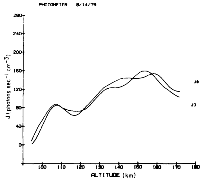
Figure 23. Volume Emission Rate for the N_2 Second Positive (0, 0 band) Emission. The results of the two in-band channels are shown separately
