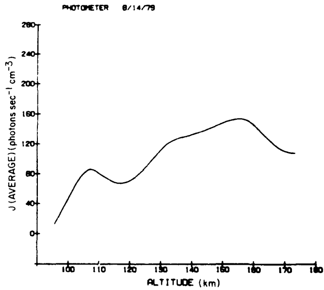
Figure 24. Volume Emission Rate of N_2 Second Positive (0, 0 band)
