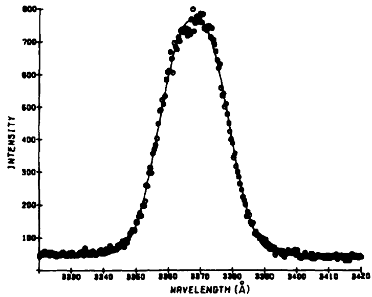
Figure 9. Relative Spectral Response of Channel 0. The solid line indicates the fit using the parameters given in Table 1
