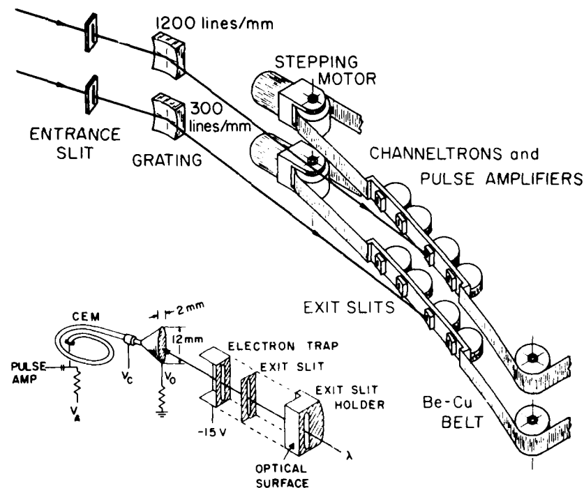
Figure 2. Schematic of the Solar EUV Spectrometer. The inset illustrates the assembly of each exit slit and its Galileo channel electron multiplier. The optical surfaces on each exit slit holder and on the entrance slit holders, not shown, are used to align the exit and entrance slits for parallelism
