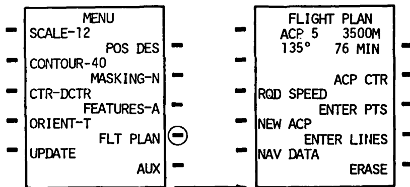
Figure 61. Calling the flight plan page on CDU.
