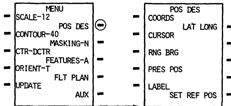
Figure 40. Calling the position designation page on CDU.
