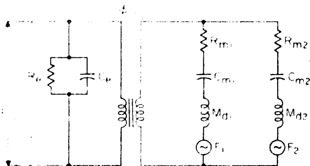
Fig. 4 — The H68B hydrophone sensor electroacoustic equivalent circuit
