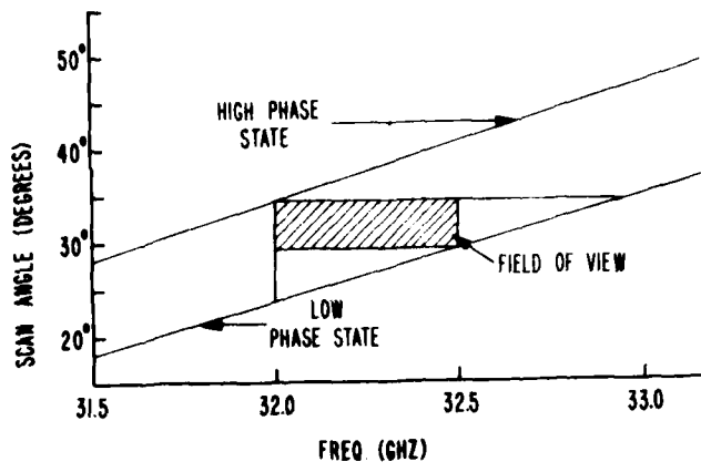
Figure 13. SFS Characteristics
