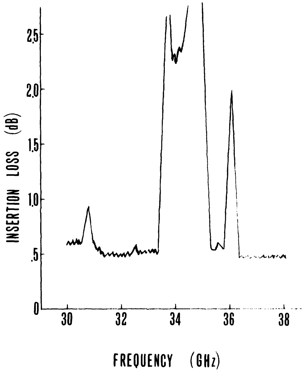
Figure 9. Insertion Loss vs. Frequency - GFS Array
