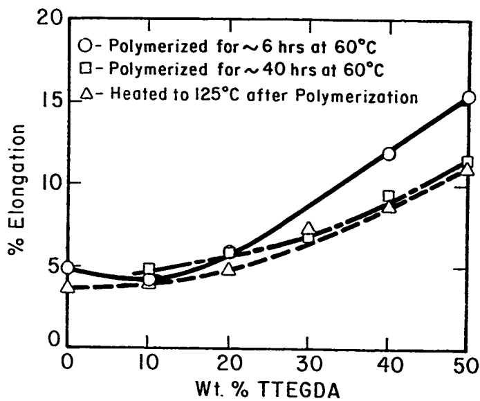
Fig. 9. Effect of TTEGDA on Polymer Ductility
