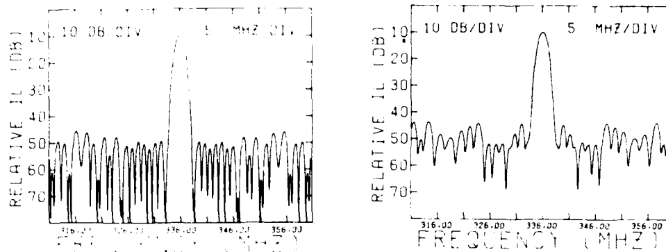
Figure 6. Theoretical Comparison of the Frequency Characteristics of a 40% Phase-Corrected, Source-Weighted Design (Left) With Those of a Combination-Weighted Device (Right)
