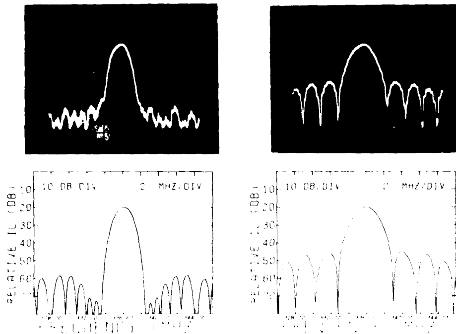
Figure 3. Relative Insertion Loss Versus Frequency Responses Comparing a Standard Withdrawal-Weighted Design (left) to an All 1's Design (right). Both are velocity corrected. Top: Experiment. Bottom: Theory
