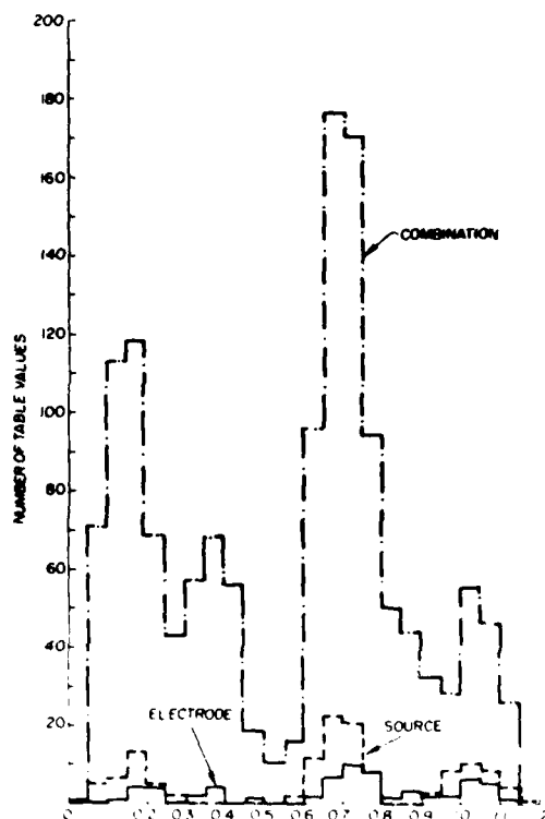
Figure 2. Distribution and Number of Individual Electrode Weights for Three Types of Constant-Finger-Overlap Weighting Schemes. Data shown is for double electrodes. Horizontal axis indicates table values ranging between 0 and 1.2
