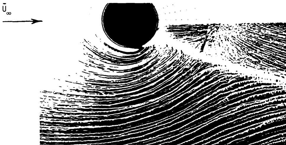
Figure 2 Oil Flow Streaklines For A Circular VSTOL Jet, From Margason And Fearn [9].
