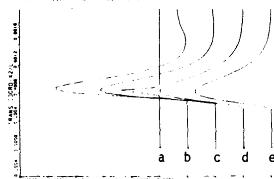
Figure 13. 2DPNS Computed Solution Field, Turbulent Rectangular Slot Jet Flow, U_j/U_j^- = 1.0/0.02 , x_1/D = \{0, .25, .5, .75, 1.0\} = \{a, b, c, d, e\} .
