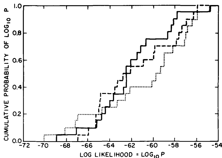
Fig. 5 — Smirnov test for three samples of size 20
