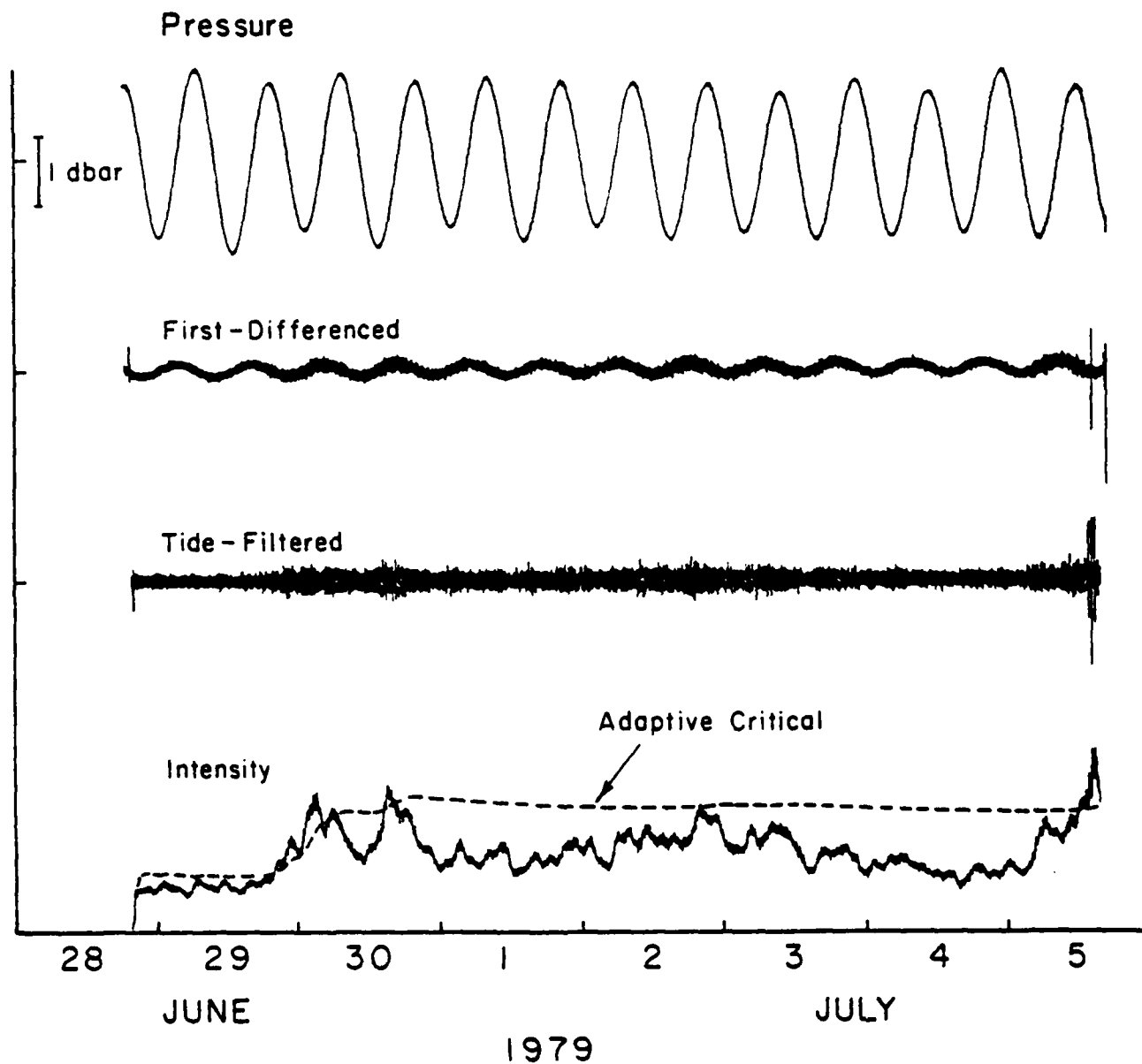
Figure 16. The conditional sampling process simulation on the computer. The pressure record shown in Figure 15 is at top, then the first difference record, tide-filtered record, and finally intensity at the bottom.
