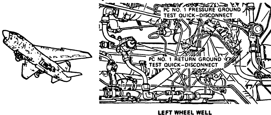
Figure 17. Connecting External Hydraulic Power
