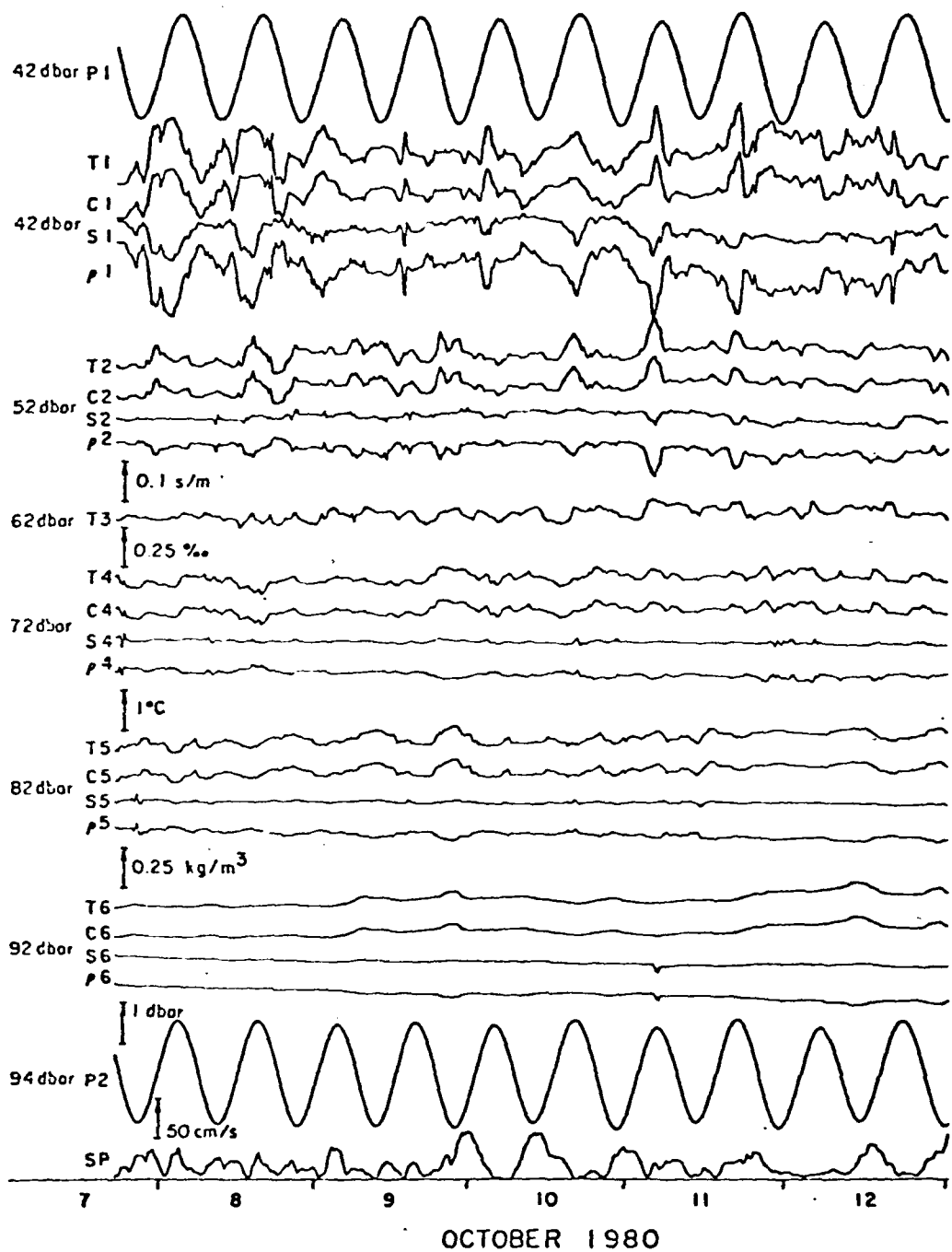
Measurements taken in Massachusetts Bay with a conditionally sampling density array. In addition to the 20 minute averages shown, the instrument recorded high frequency "conditionally sampled" data.
