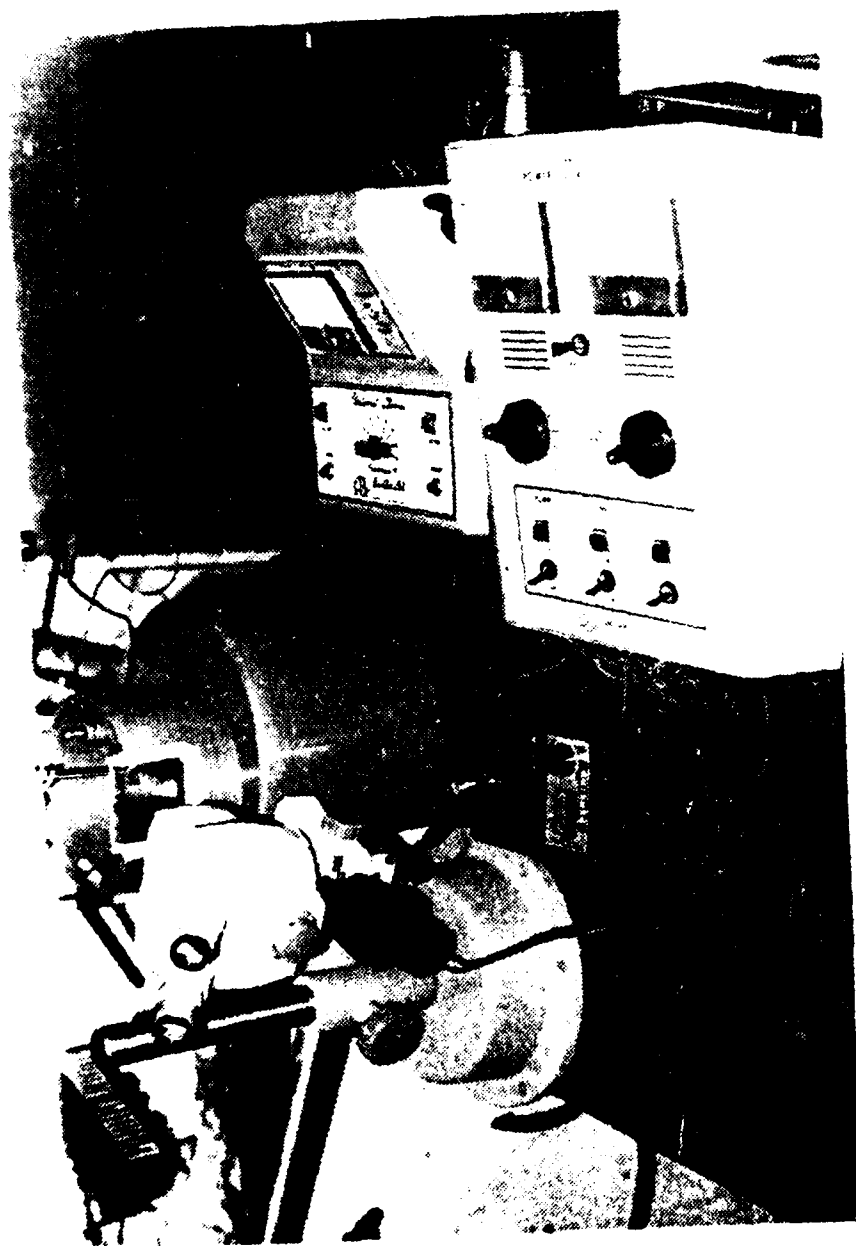
FIGURE 5. Electrolyte Thinning Apparatus Utilized for Thin Foil Preparation (power supplies included)
