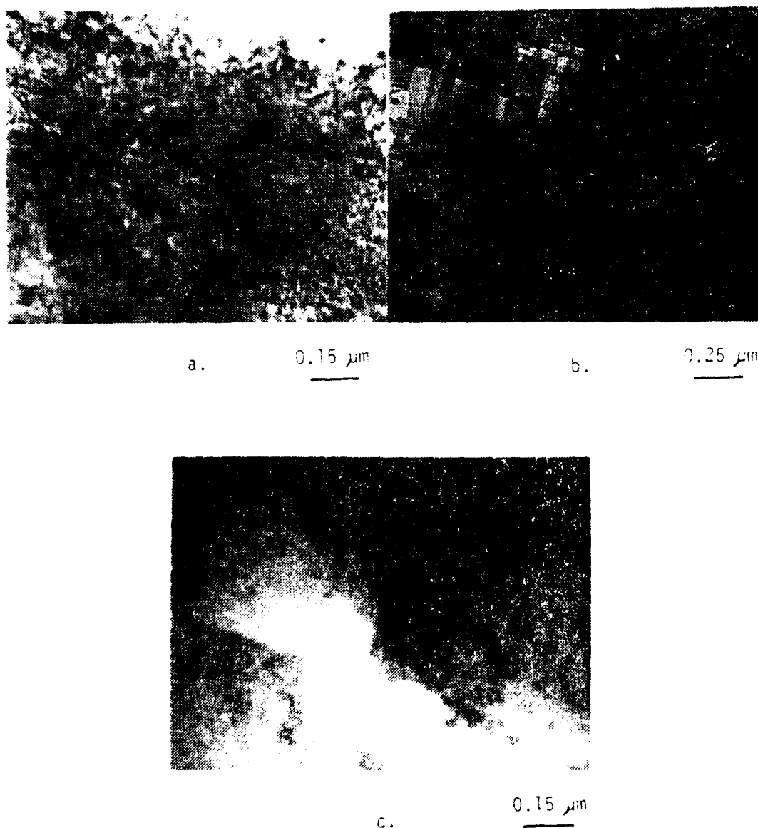
FIGURE 16. Regions of thin coils of Al-10.2 wt pct Mg, oil-quenched from homogenization, in the as-rolled condition indicating (a) heavily dislocated region similar to that expected of a cold worked material; (b) coarse precipitates which have sheared during subsequent rolling passes, and the diffuse cellular substructure; (c) light regions outlining original locations of precipitates and heavily dislocated structure
