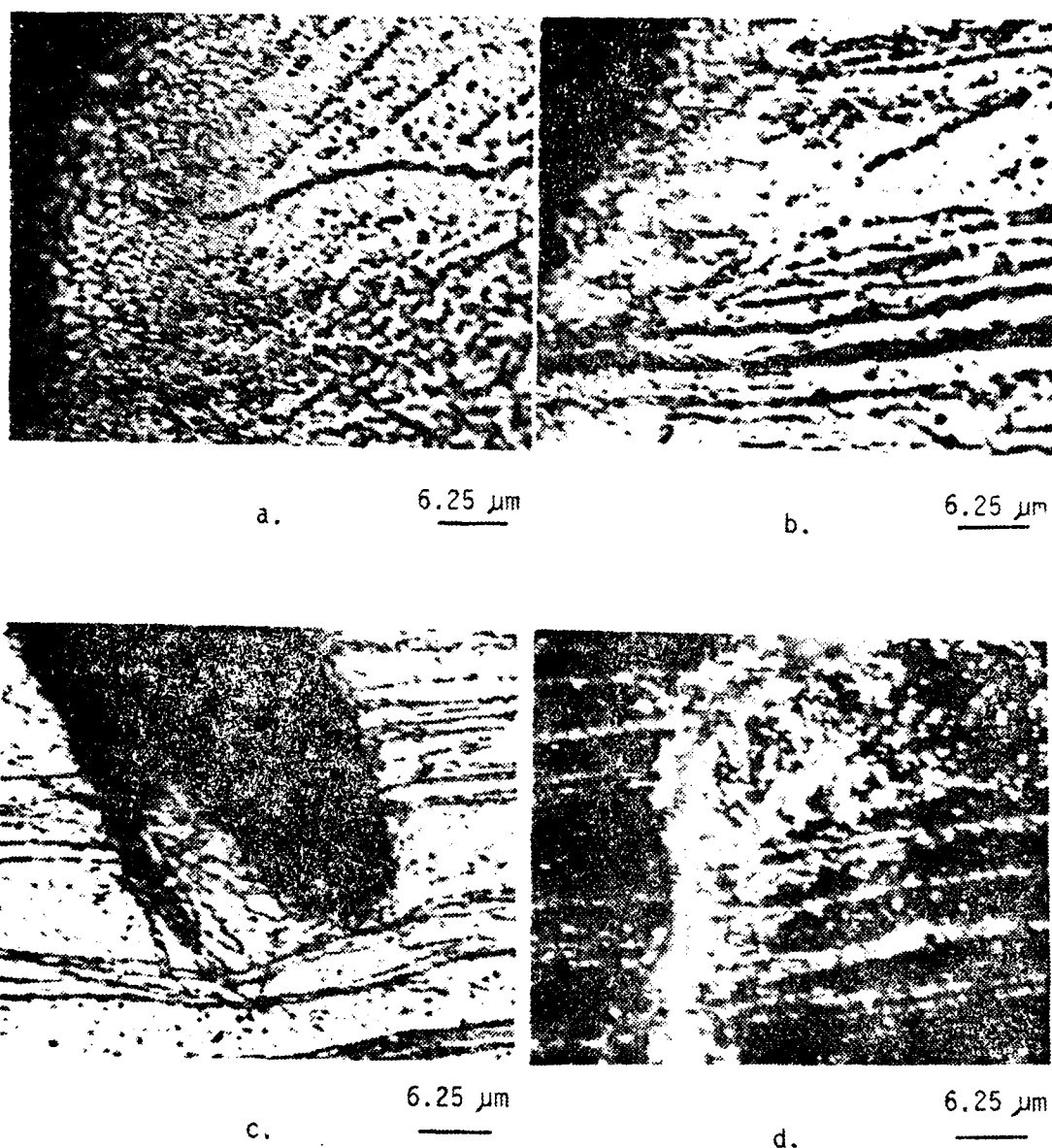
FIGURE 45. Optical micrographs of a low cycle fatigued specimen of Al-3.14 wt pct Mg-0.40 wt pct Cu, solution treated, water-quenched and warm-rolled at 300°C: (a) region adjacent to the main fracture surface; (b) region adjacent to the main fracture surface; (c) region adjacent to a blunt tipped secondary crack; and (d) region adjacent to and in front of a crack tip (dark field image)
