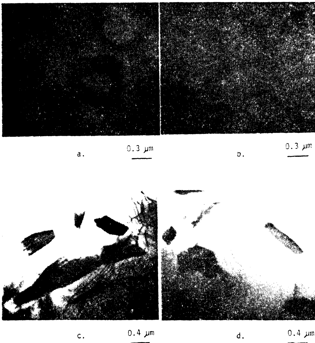
FIGURE 19. Thin foils of Al-10.2 wt pct Mg artificially aged (a) oil-quenched from homogenization showing sites originally occupied by second phase particles; (b) oil-quenched from homogenization, relatively free of precipitates with small dislocation density; (c) and (d) water-quenched from homogenization showing precipitate growth during aging at 500^{\circ}\text{C} with dislocations believed generated through increments volume occupied by second phase particles
