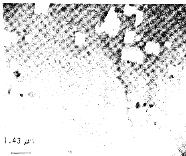
FIGURE 34. Thin foil TEM micrograph of Al-10.2 wt pct Mg solution treated, water-quenched and warm-rolled at 300°C after being tested under low cycle fatigue conditions; (a) some indication of larger precipitates (b) region where volume fraction of precipitates is increased over the as-rolled condition (dark blotches in (b) are artifact from electrolyte thinning)
