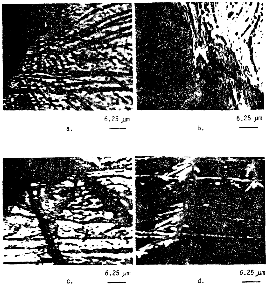
FIGURE 40. Optical micrographs of a low cycle fatigued specimen of Al-8.14 wt pct Mg-0.40 wt pct Cu, solution treated, oil-quenched and warm-rolled at 300°C: (a) adjacent to the main fracture surface; (b) adjacent to the main fracture surface; (c) secondary cracks originating at the main fracture surface; and (d) secondary cracks (dark image)
