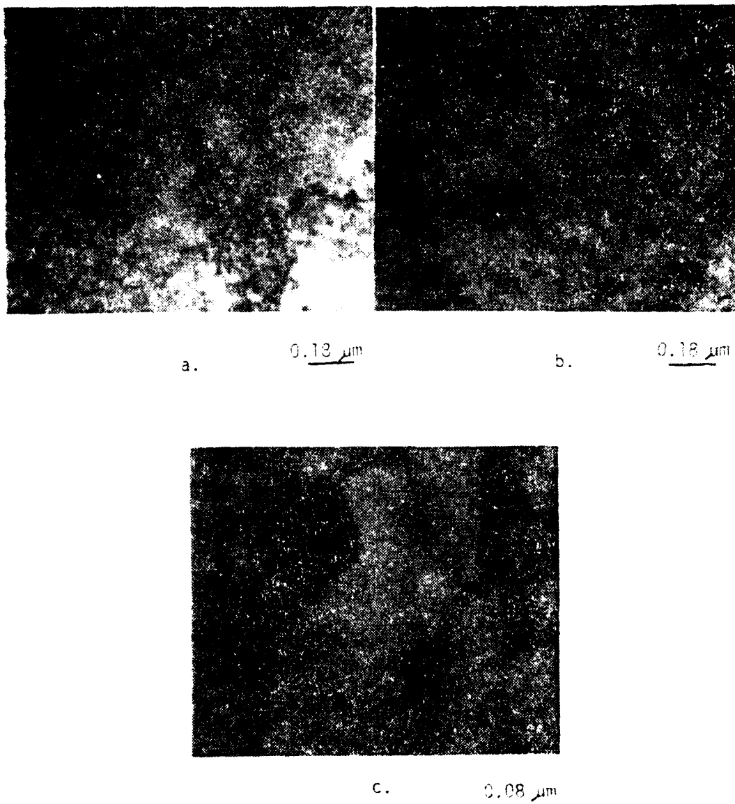
FIGURE 17. Regions of thin foils of Al-10.2 wt pct Mg, water quenched from homogenization, in the as-rolled condition indicating (a) heavily dislocated and diffuse cellular substructure; (b) same region as (a), but tilted; (c) cellular nature of substructure more clearly defined at higher magnification
