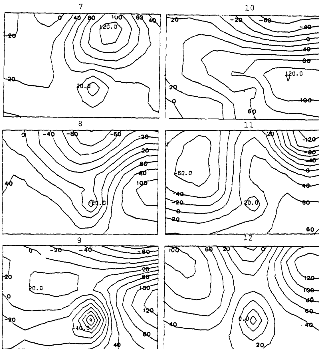
Fig. C1. cont. 850 mb map types 7-12.
