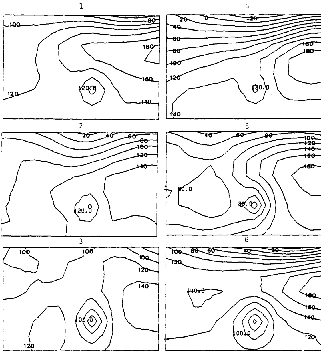
Figure C2. 700 mb map types 1-6. Isopleths are D-values (m).
