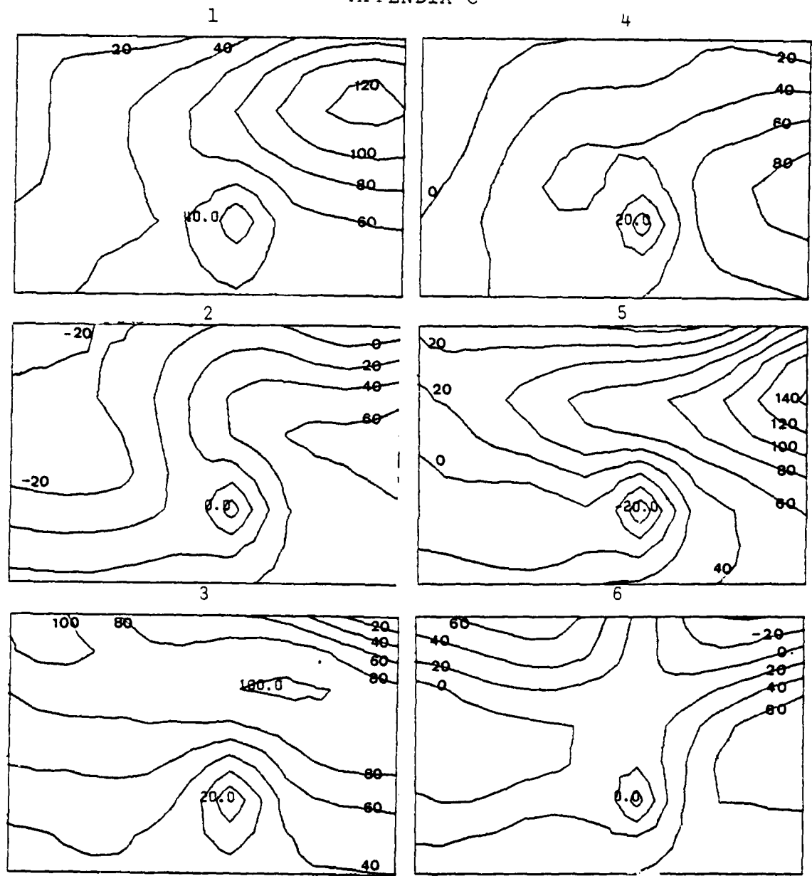
Figure C1. 850 mb map types 1-6. Isopleths are D-values (m).
