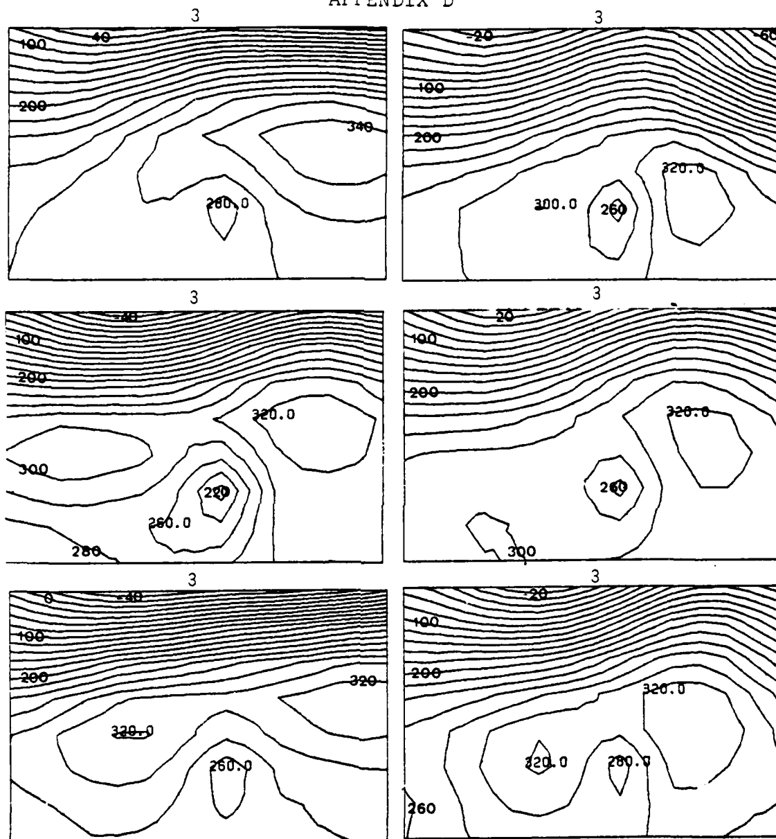
Figure D1. Examples of 500 mb maps. Isopleths are D-values (m) and the classification by map type is indicated by the number above the map.
