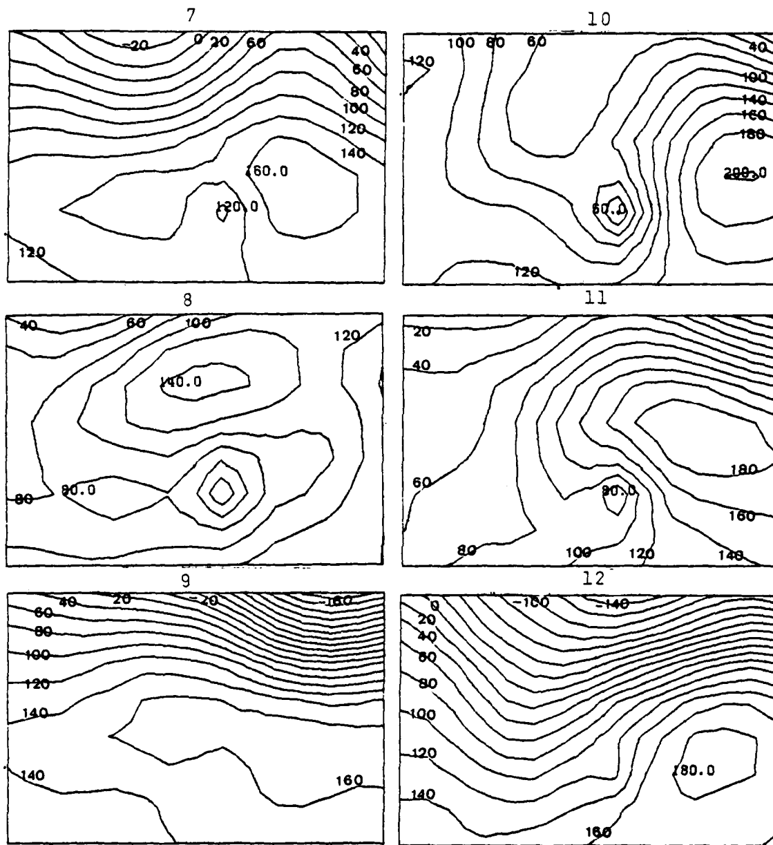
Fig. C2. cont. 700 mb map types 7-12.
