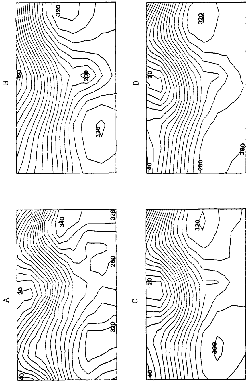
Figure 5. Similar to Fig. 4 except for 12 GMT 25 Aug 1967.
