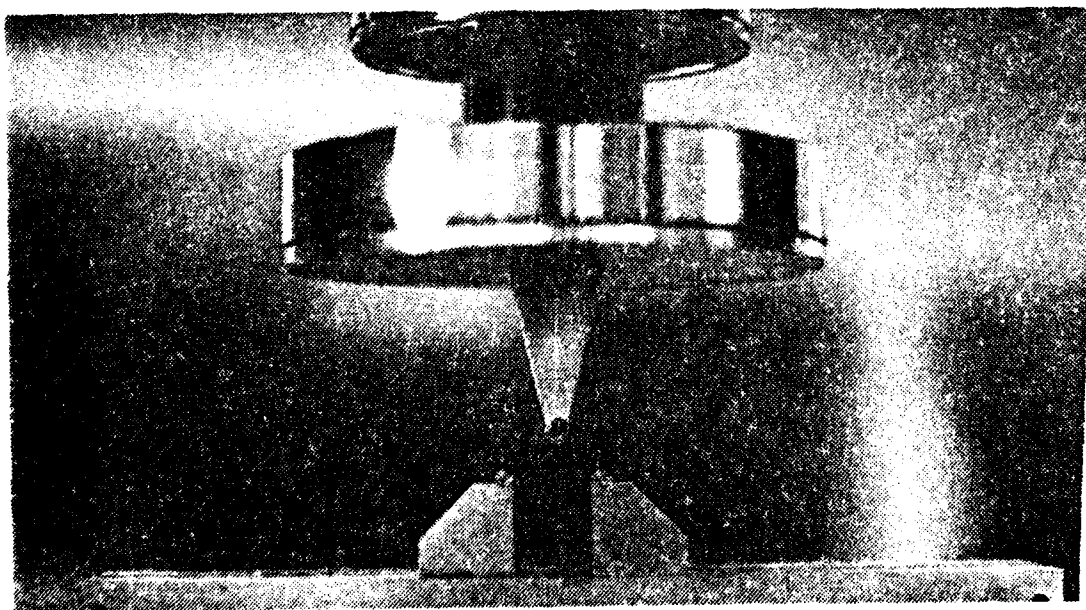
FIGURE 16: TEST RIG SETUP FOR TESTING 1/4 INCH SAMPLES
