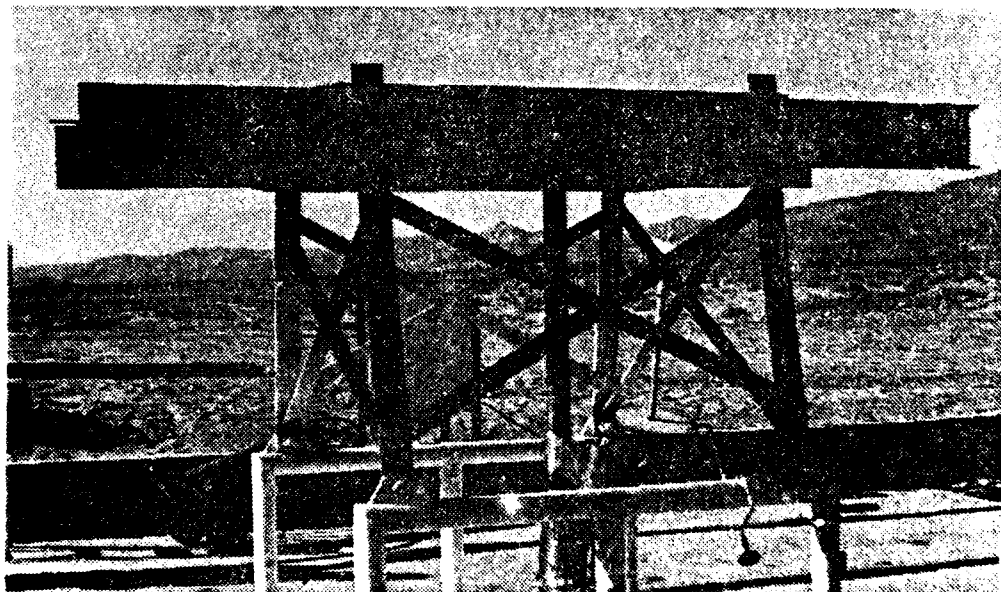
FIGURE 23: WINGBOX AT CONCLUSION OF TESTING. NOTE SOOT BUILD- UP ON WINGBOX
