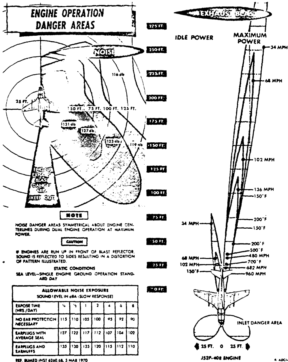
Figure 1-24. Engine Operation Danger Areas
