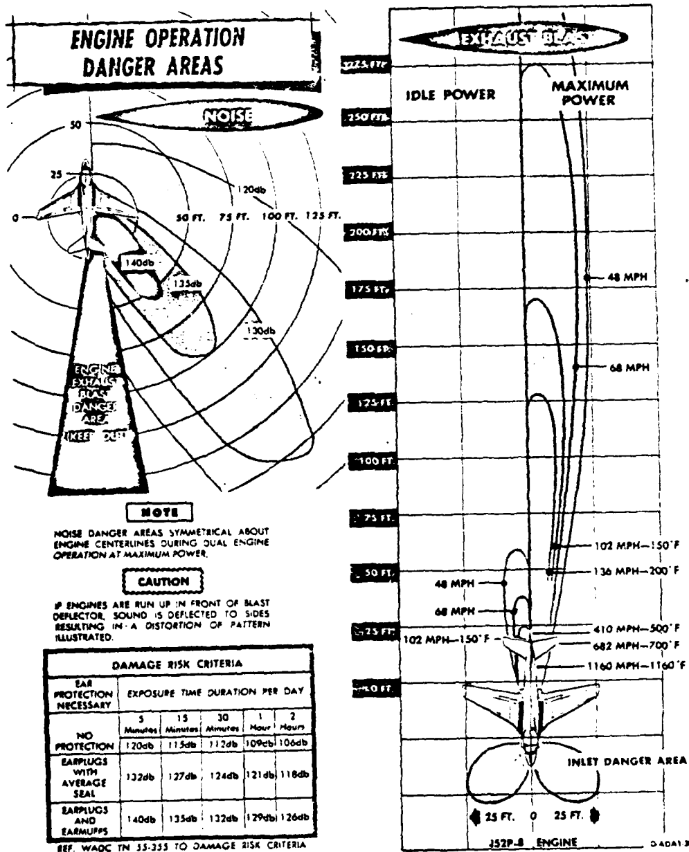
Figure 1-38. Engine Operation Danger Areas A-16E/A-16
