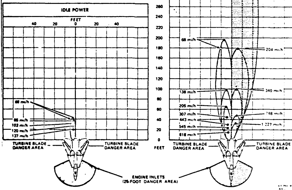
Figure 1-90. Runup Danger Areas (Sheet 2 of 2)
