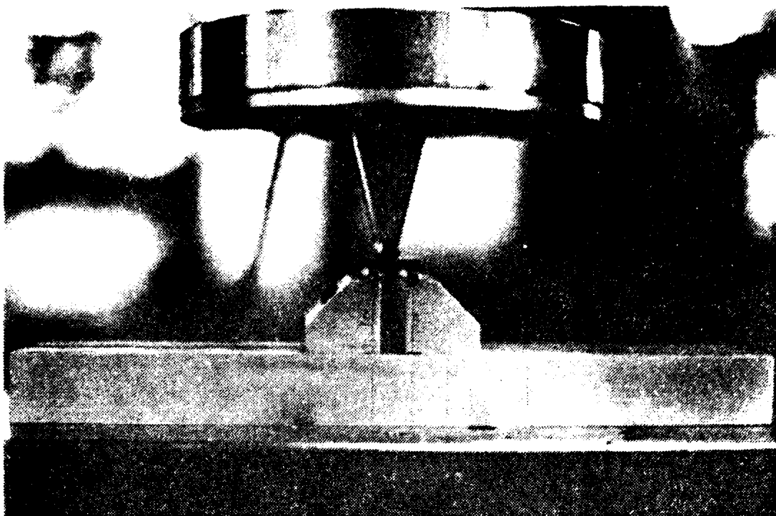
FIGURE 15: TEST RIG SETUP FOR TESTING 1/8 INCH SAMPLES
