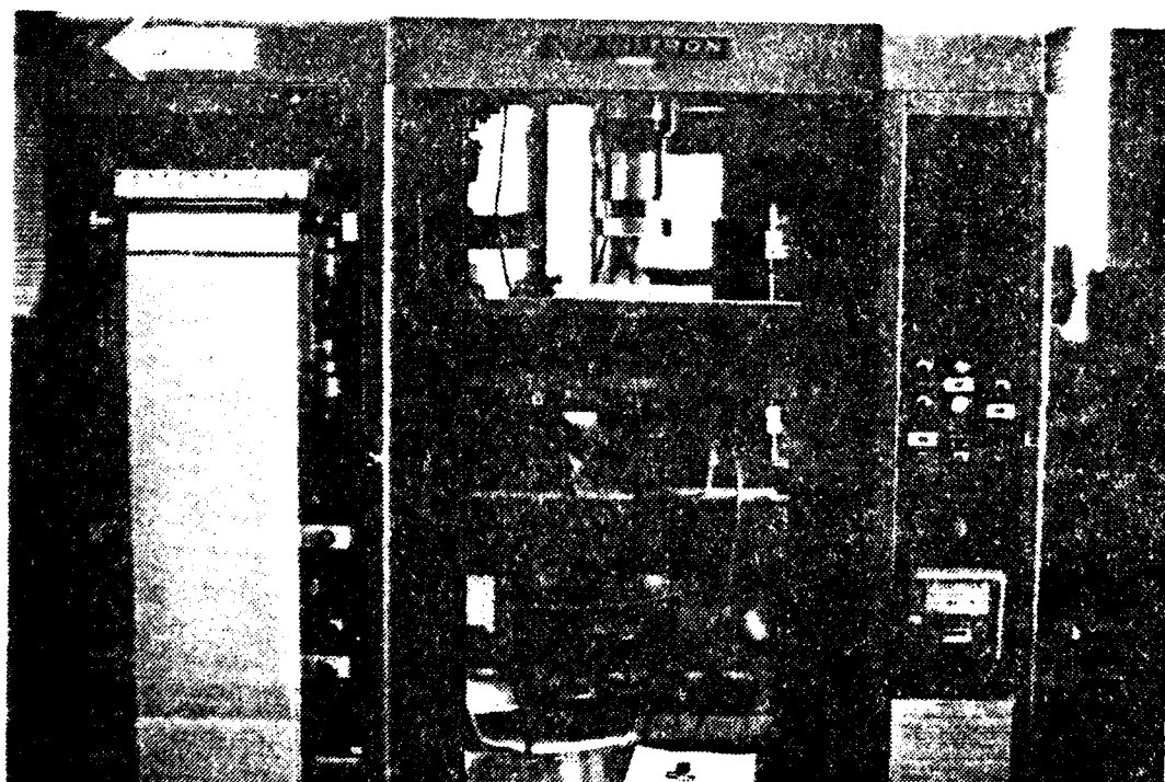
FIGURE 18: INSTRON SETUP FOR SHORT BEAM SHEAR TEST
