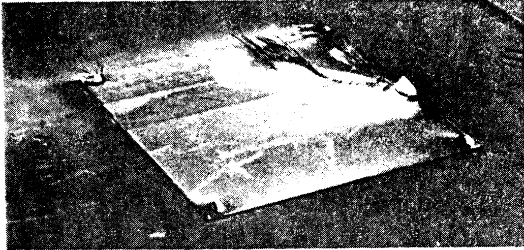
FIGURE 19: 1/2 COMPOSITE AFTER TESTING. NOTE DELAMINATION TEST NUMBER 6
