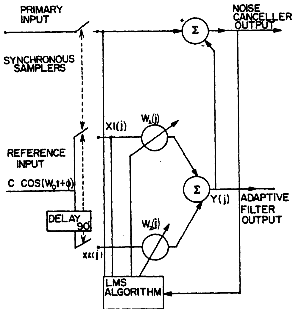
Fig. 2.11. Single Frequency Adaptive Noise Canceller
