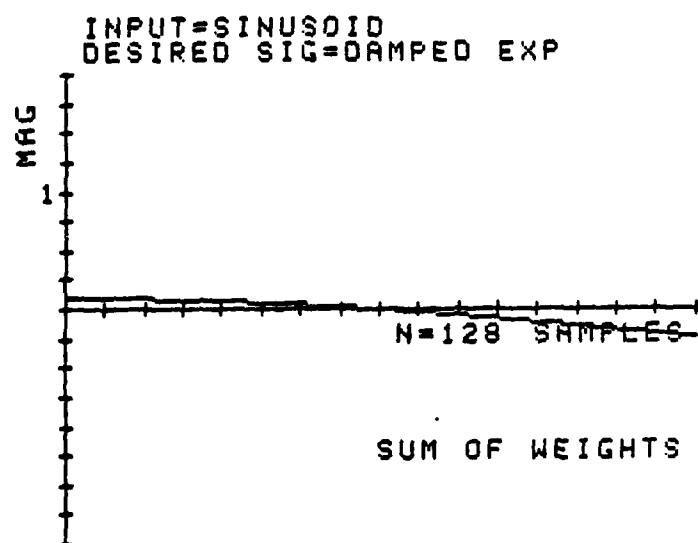
Fig. 4.36. Sum of Weights Plotted Through N = 128 Samples. Linear Constraint K = -.2
