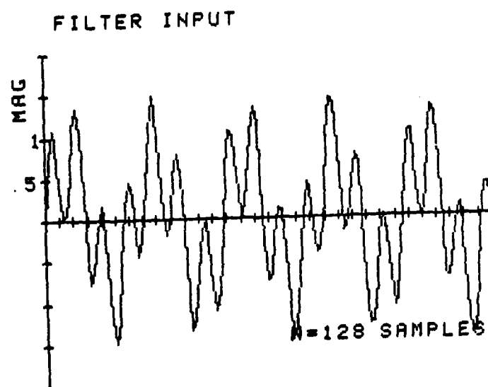
Fig. 4.25. System Input - Four Adaptive Weights
