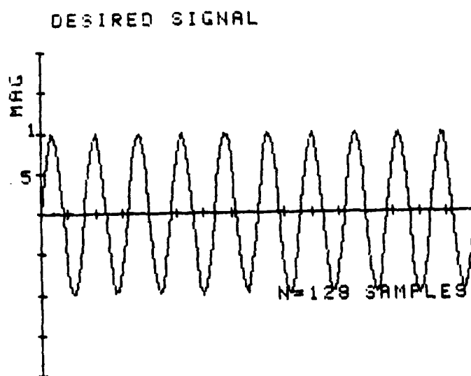
Fig. 4.2. System Reference Signal Sampling Frequency F_s = 128 Hz
