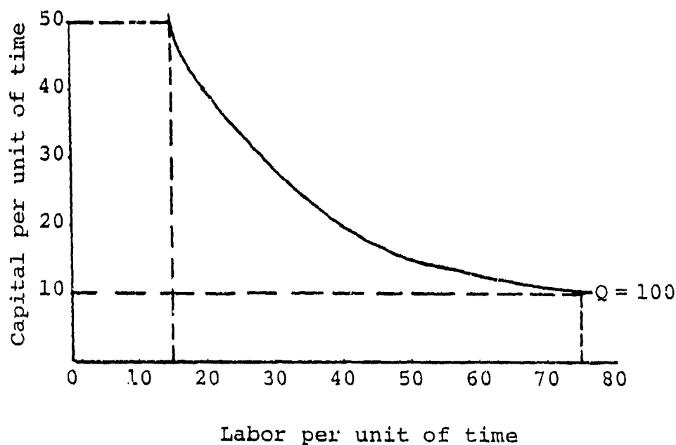
FIGURE V-1 PRODUCTION ISOQUANT
