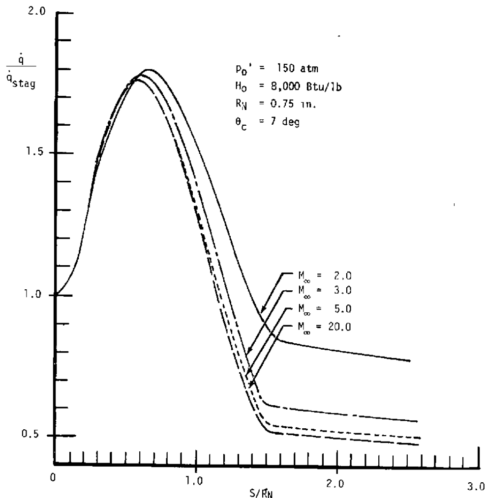
Figure 5. Influence of free-stream Mach number on turbulent heat flux on a sphere-cone.
