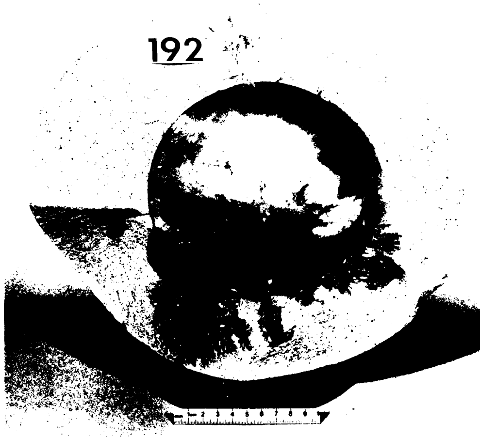
FIGURE 3.34 HYDROFRACTURE FROM UNVENTED EXPLODED CAVITY TEST 192 NEARBY VERTICAL FAULT
