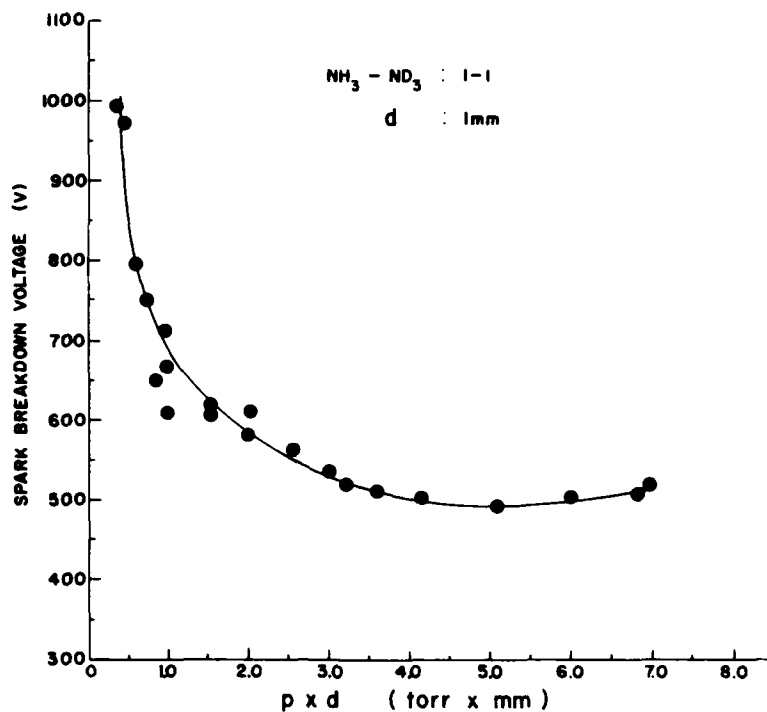
FIGURE 6 - Paschen curve for the Stark cell. The electrode spacing was about 1 mm.
