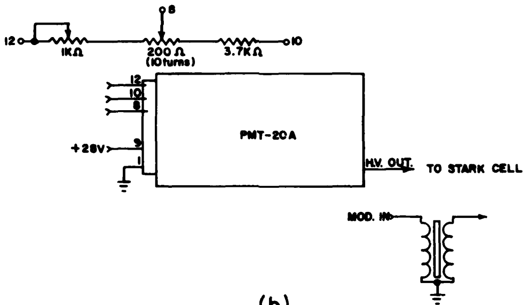
FIGURE 4 - Schematic circuit diagram of the accompanying electronic: (a) detector and preamplifier, (b) biasing circuit
