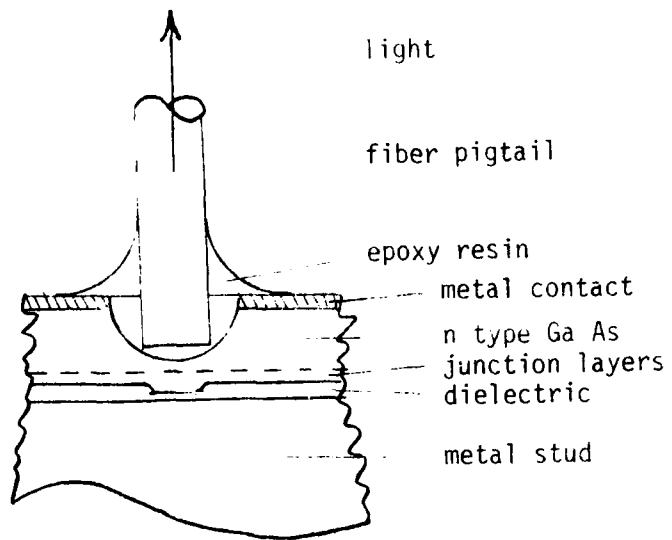
Figure 3. Surface Emitter
