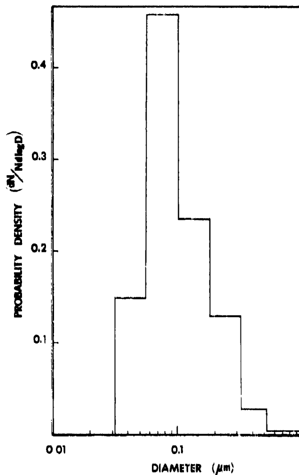
Figure 6. 0.007 - 1 μm particle size distribution probability density function measured by EAA for trial 18, white phosphorus.
