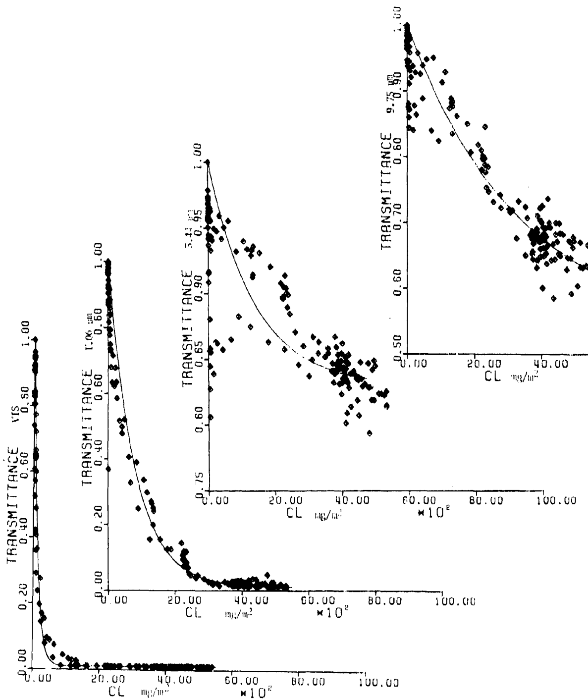
FIGURE 4. CURVE FIT FOR SP11A-T-3 HC SMOKE.
