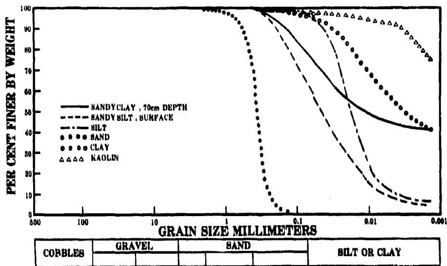
FIGURE 5. SOIL TYPES ENCOUNTERED OR TAILORED DURING THE UH1-III PROJECT: (1) Natural surface, dark brown sandy silt; (2) natural soil, 70 cm deep, reddish sandy clay; (3) kaolin, tailored soil test; (4) sand tailored soil test; (5) clay, tailored soil test; (6) silt, tailored soil test.
