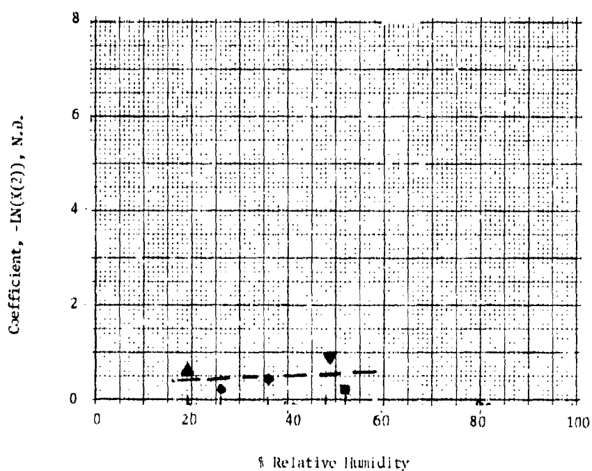
FIGURE 16. CORRELATION COEFFICIENTS VS RELATIVE HUMIDITY FOR HC SMOKE AT 9.75 \mu m .
