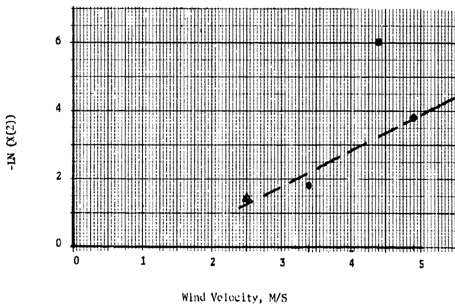
FIGURE 8. CORRELATION COEFFICIENTS VERSUS WIND VELOCITY FOR WP SSMKE AT 3.44 \mu\text{m} .
