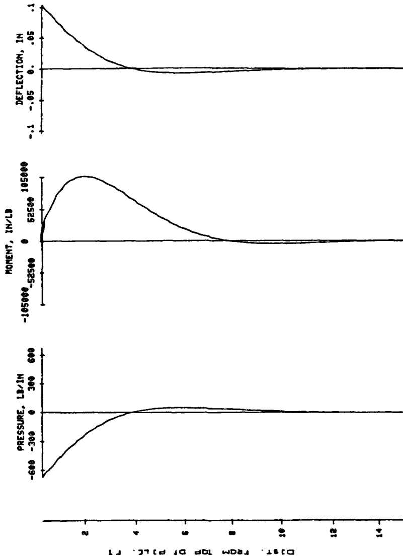
Figure 50. Pressure, moment, and deflection in the most critically loaded pile for normal operation plus ice
