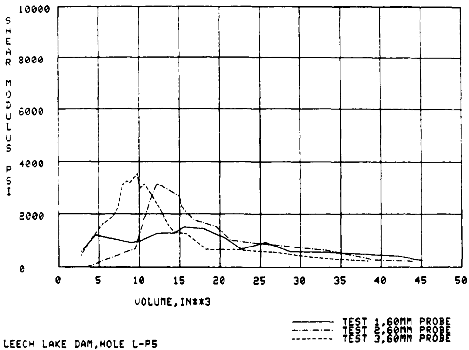
Figure 24. Shear modulus, L-P5
