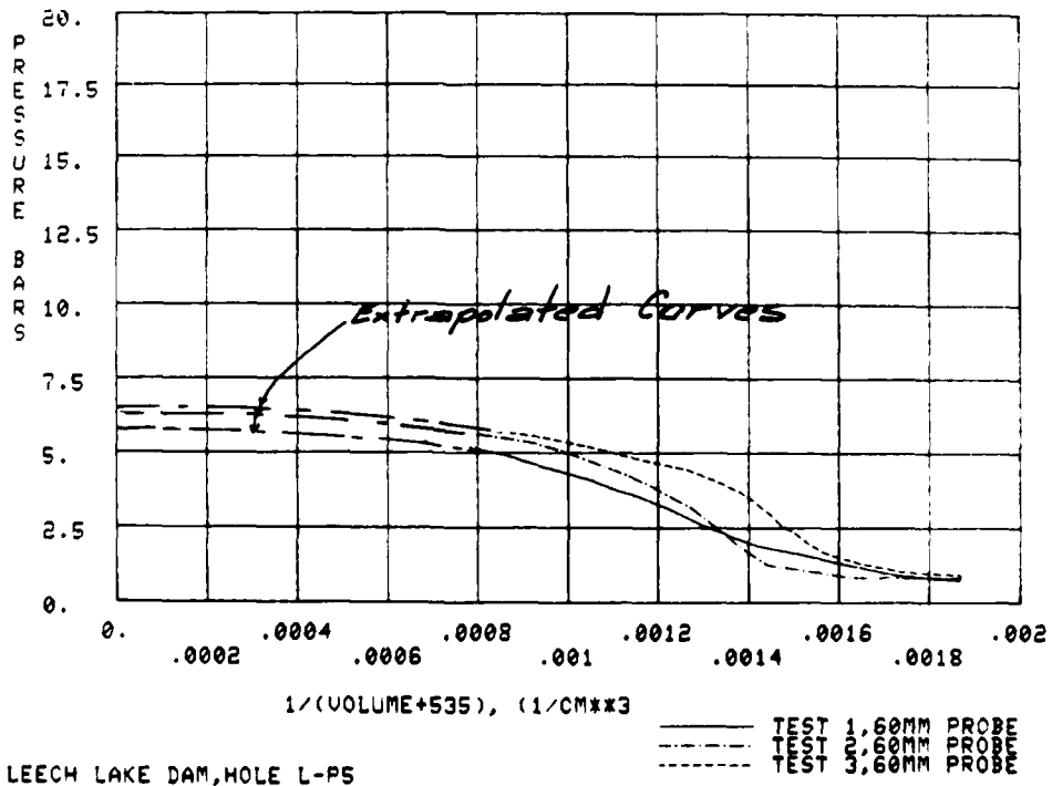
Figure 22. Limit pressure determination, L-P5
