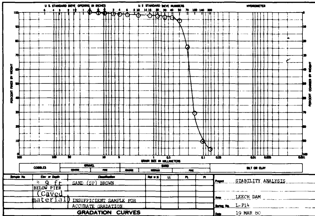
Figure 16. Foundation soil sieve analysis and classification, L-P14, ≈ 9 ft
