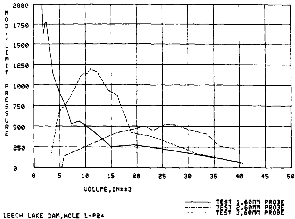
Figure 40. Ménérd modulus divided by limit pressure, L-P24
