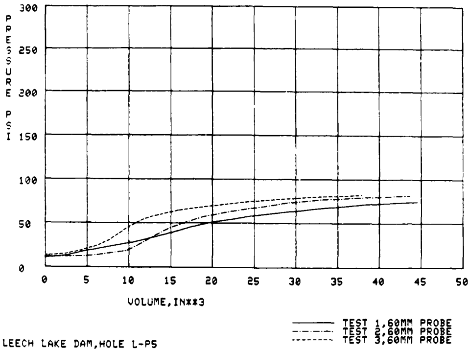
Figure 23. Pressure versus volume, L-P5
