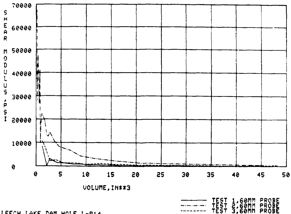
Figure 31. Shear modulus, L-P14
