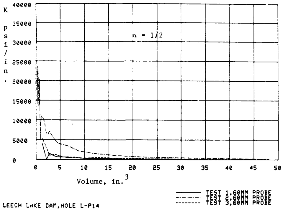
Figure 34. Modulus of subgrade reaction, L-P14
