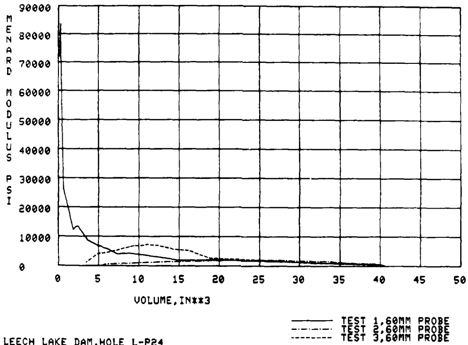
Figure 39. Ménérd modulus, L-P24
