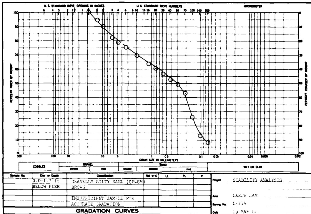
Figure 15. Foundation soil sieve analysis and classification, L-P14, 0.0-1.7 ft
