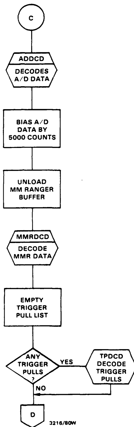
Figure V-1. EXEC Flowchart (Continued)
