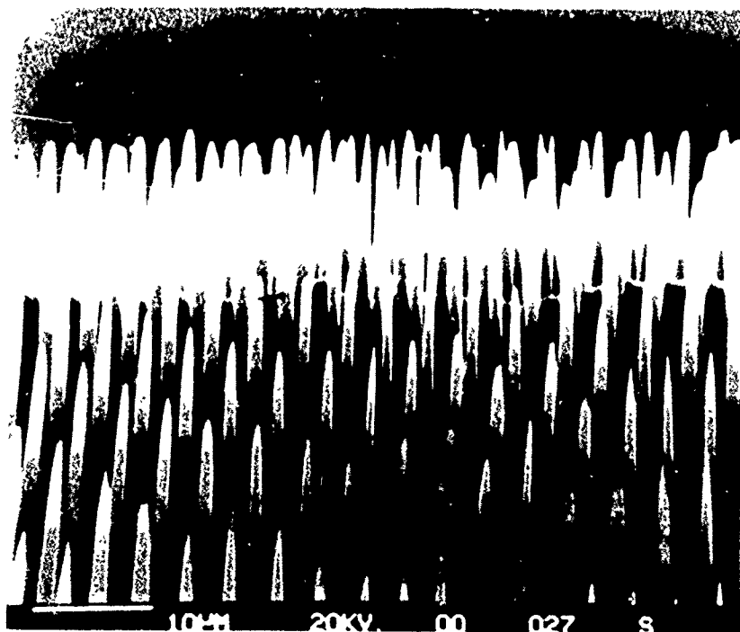
Figure 20. Side view of top edge of "Chisel" shaped VC cathode before testing. x 2K C6403
