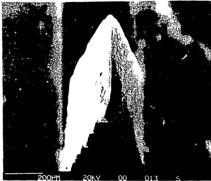
Figure 18. General View of "Chisel" shaped VC cathode before testing. x 150 C6389
