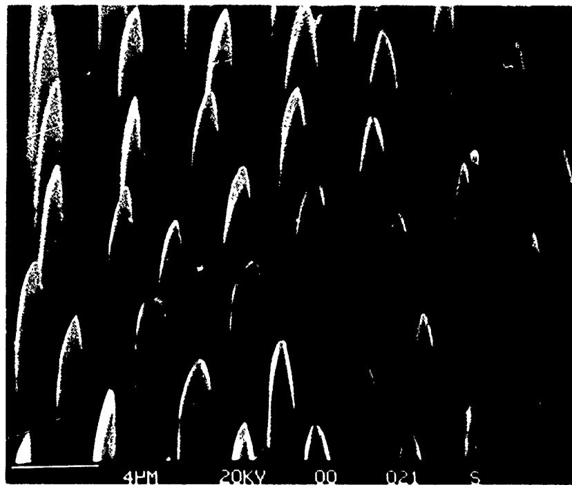
Figure 19. View along the top edge of "Chisel" shaped VC cathode before testing. x 5K C6397
