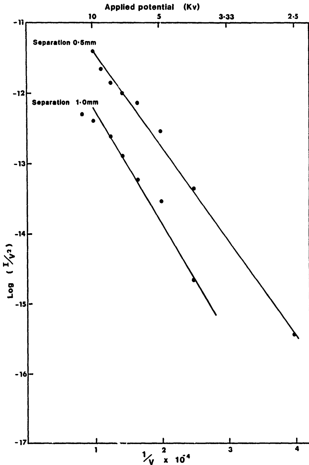
Figure 41. Fowler - Nordheim plots for material A77-205 cathode at the anode to cathode separation shown
