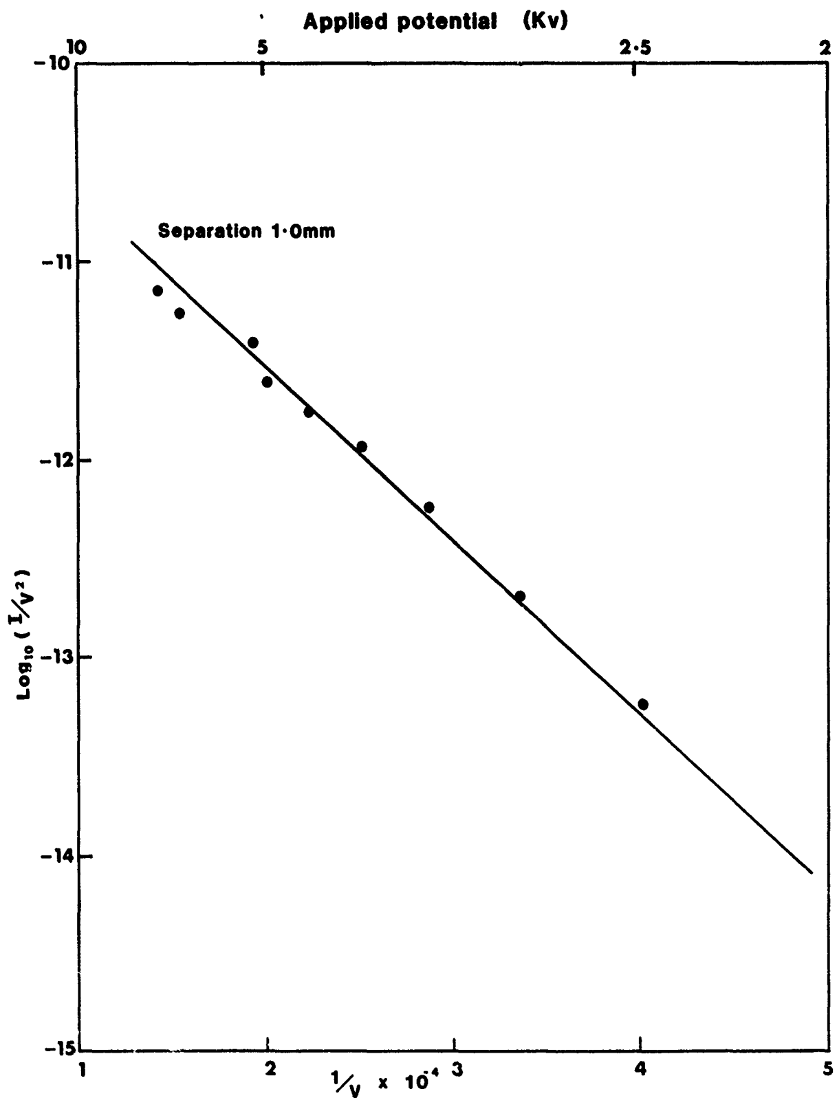
Figure 33. Fowler - Nordheim plot for NbC cathode at the anode to cathode separation shown
