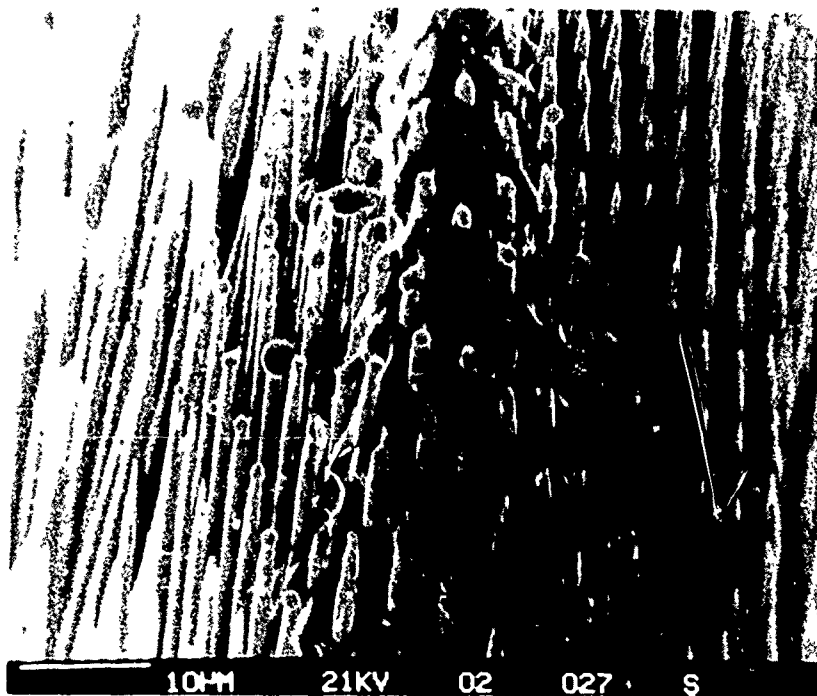
Figure 45. End View of Corner B of "Chisel" shaped VC cathode after testing. x 2K
