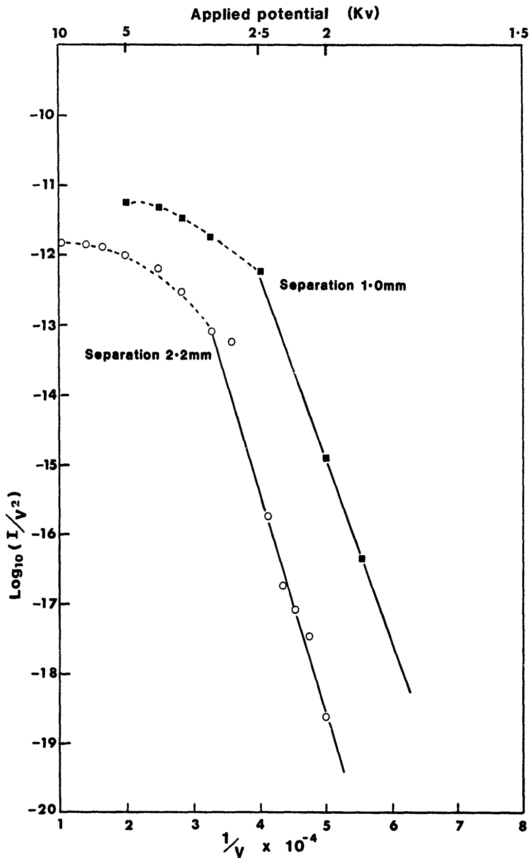
Figure 26. Fowler - Nordheim plots for TaC cathode at the anode to cathode separation shown
