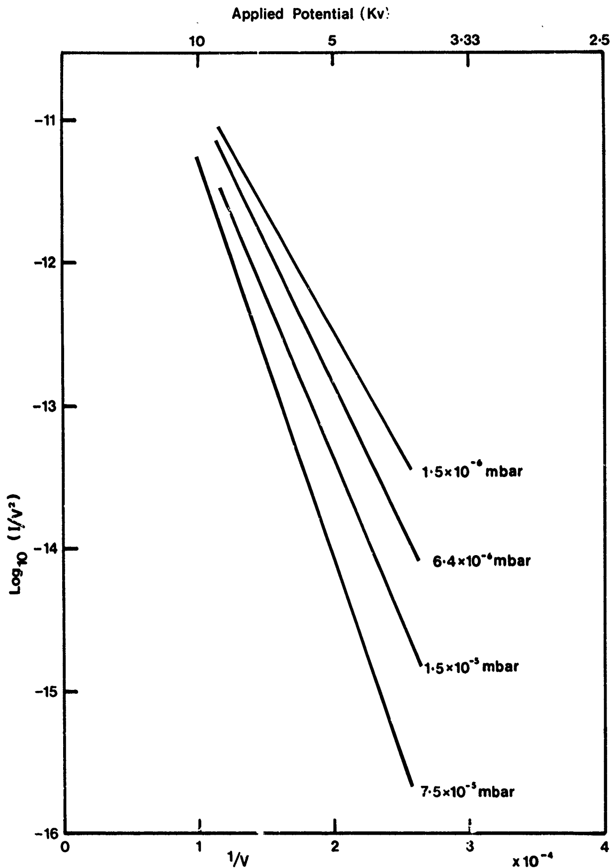
Figure 36. Fowler-Nordheim plots for NbC at the chamber pressures shown (after 1000 hour life test)
