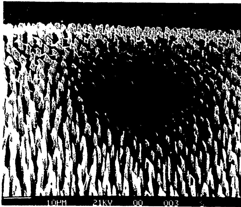
Figure 44. Dark Area on 300μ x 400μ VC Cathode C6524 x 2K after testing.
