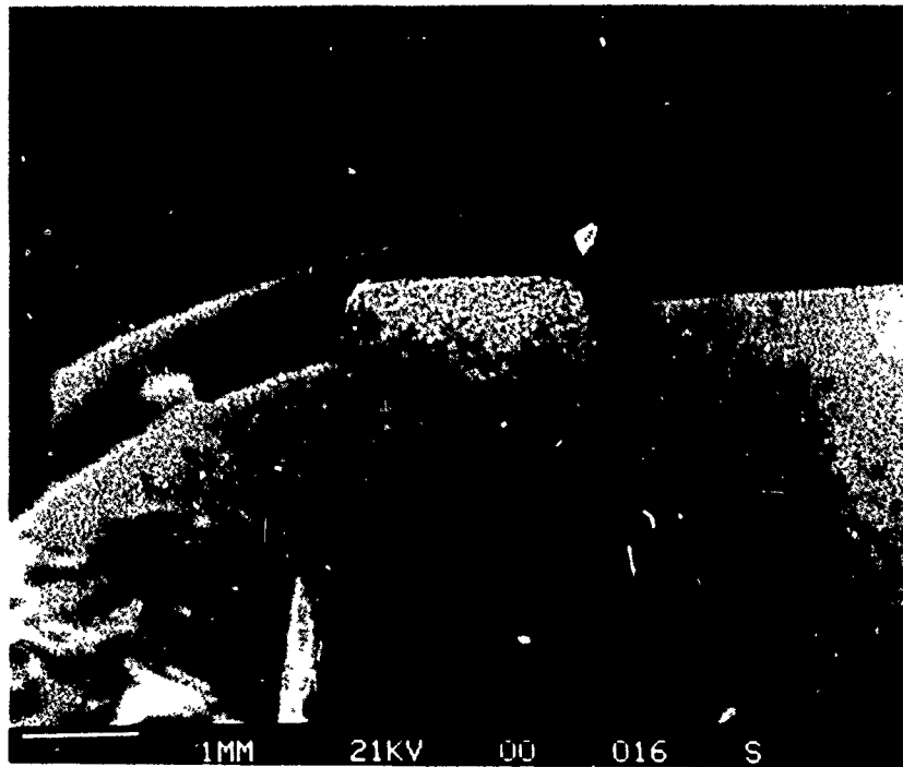
Figure 6. General View of small fibre M5C cathode before 1000 hour life test. x 20 C6561
