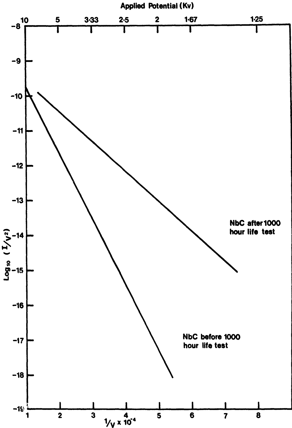
Figure 35. Fowler-Nordheim plots for small fibre NbC eutectic before and after 1000 hour life test
