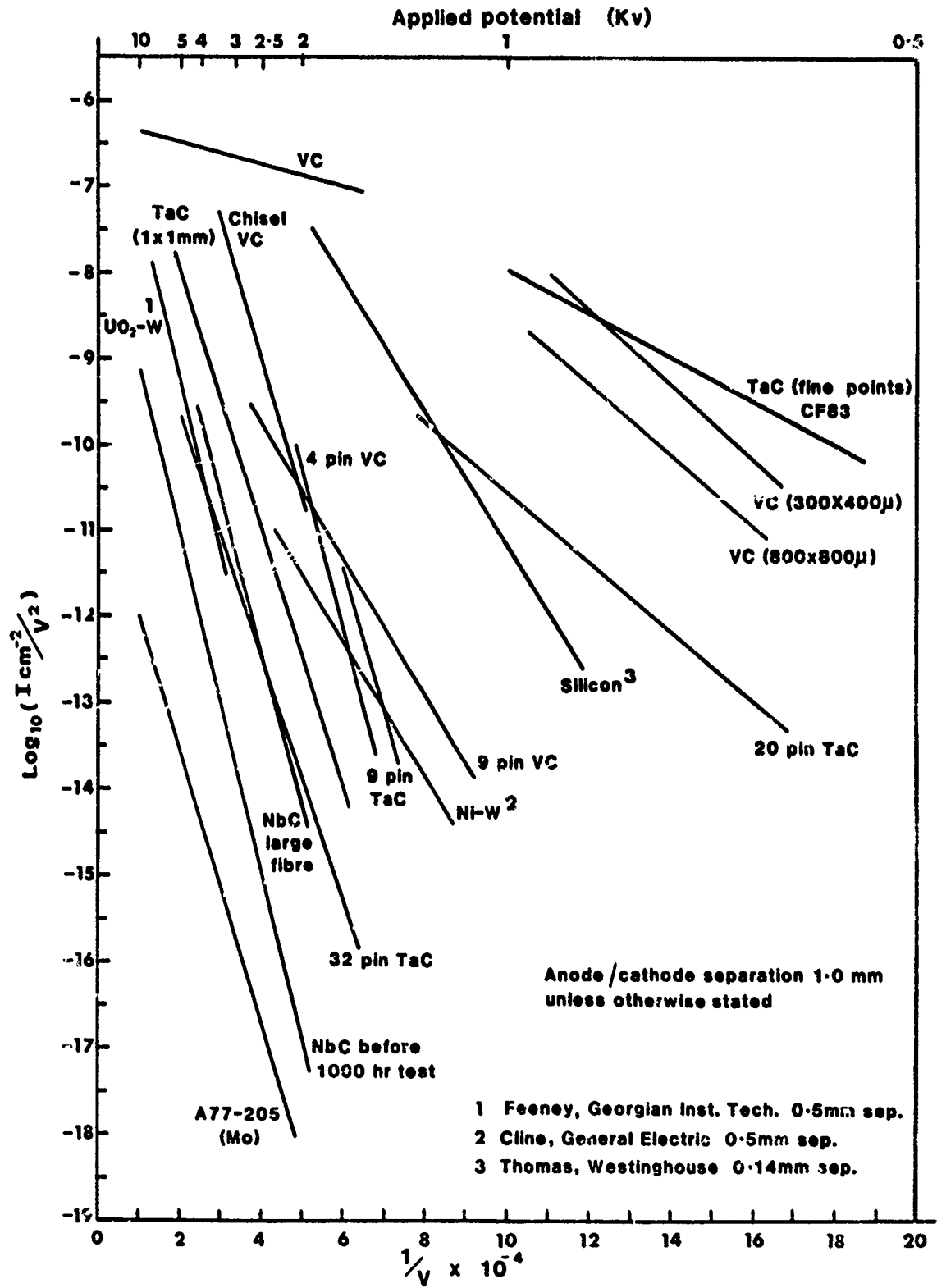
Figure 57. Set of F-N plots obtained at FRI and by Feeny et Al.
