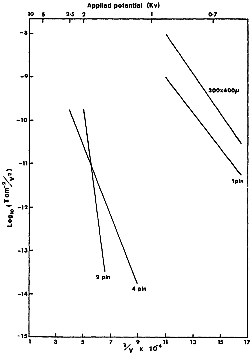
Figure 42. Fowler - Nordheim plots for Vanadium Carbide cathodes
