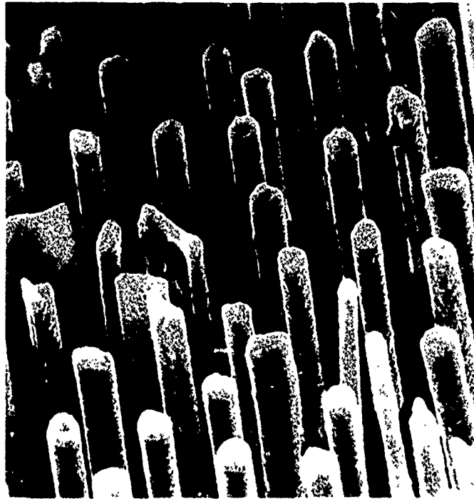
Figure 5. Typical area of M5C cathode before 1000 hour life test. x 2.9K C5577
