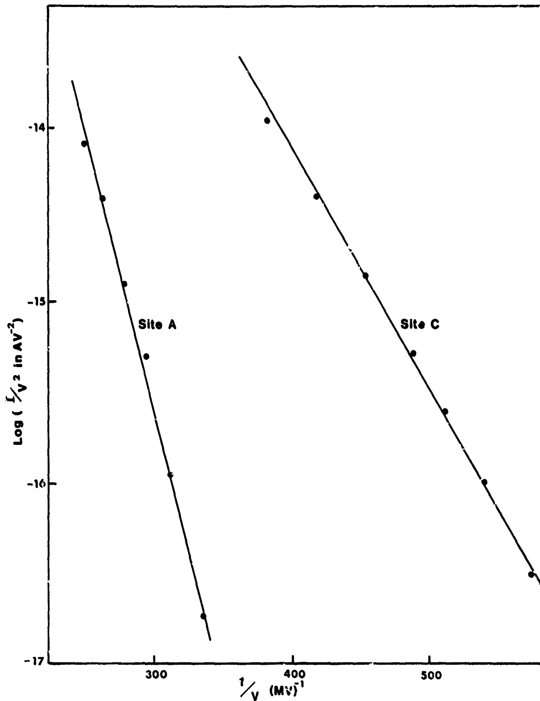
Figure 56. F-N plots for two different TaC emission sites
