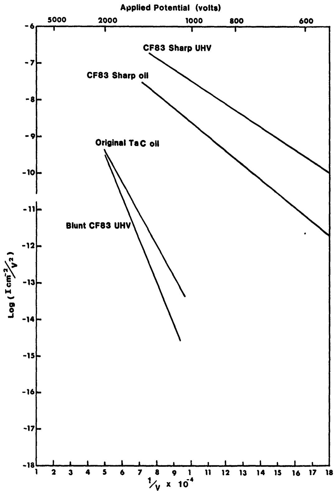
Figure 50. F-N Plots Comparing Sharp CF83 (oil and UHV), blunt CF83 and original TaC
