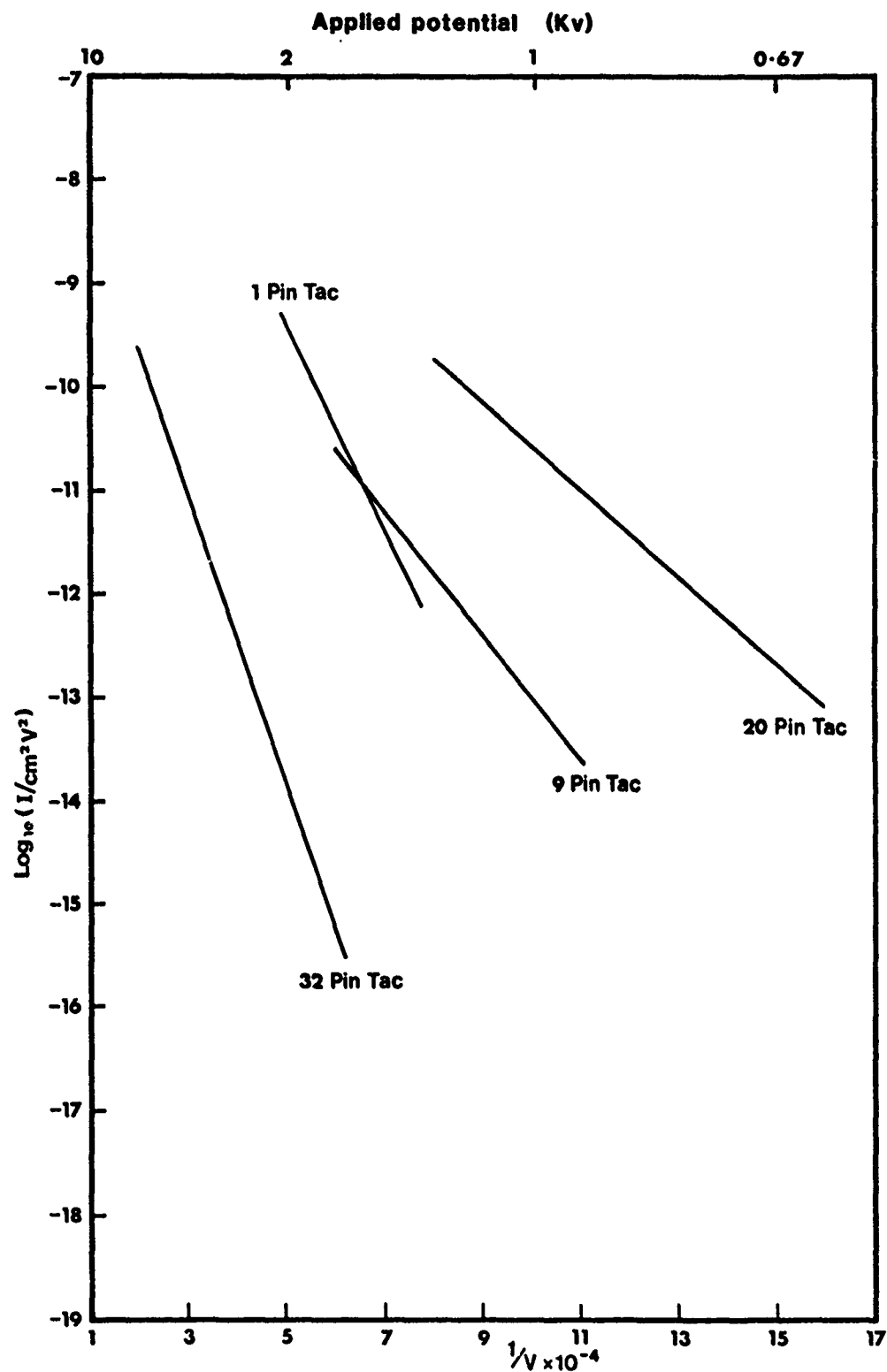
Figure 28. Comparison of Fowler-Nordheim plots for Tantalum Carbide cathodes
