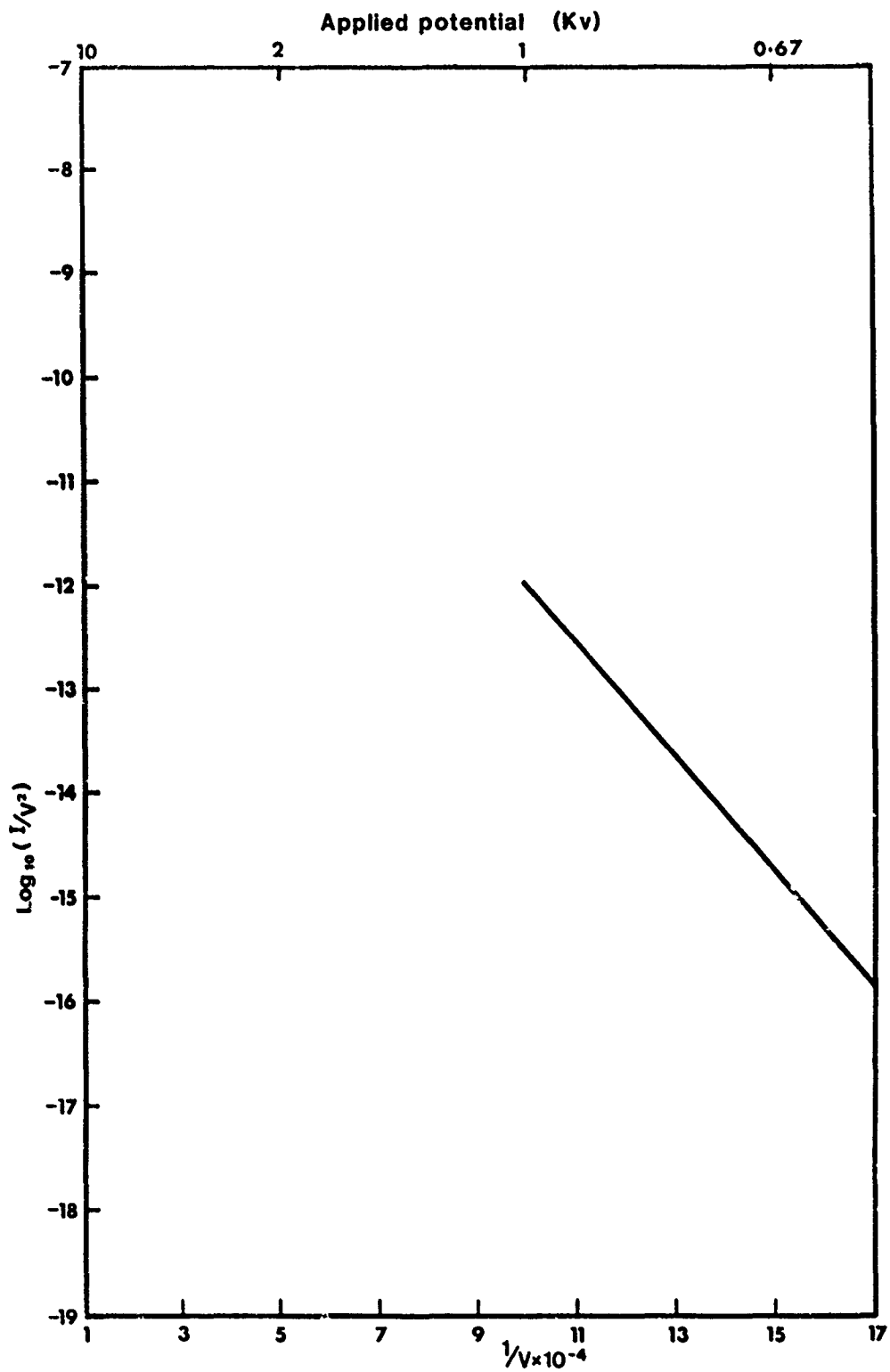
Figure 37. Fowler - Nordheim plot for single fibres of Niobium Carbide
