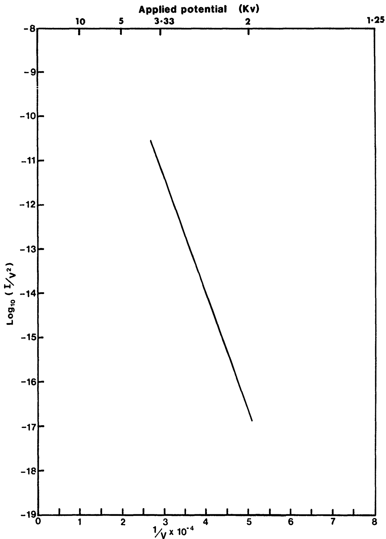
Figure 47. Fowler - Nordheim plot for "chisel" shaped Vanadium Carbide
