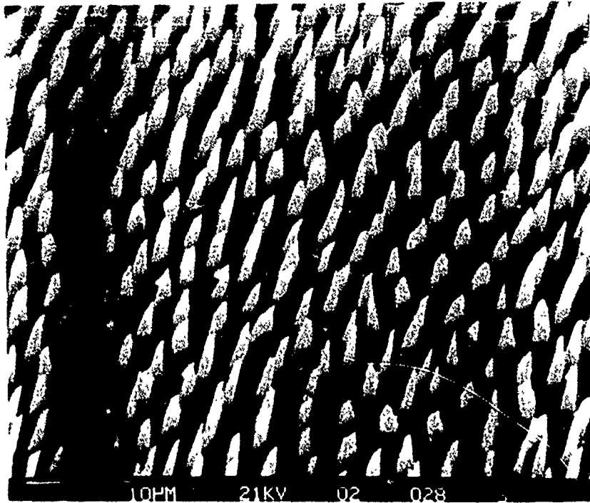
Figure 17. Typical Central area of 300 \mu x 400 \mu VC cathode before testing. x 2K C6487
