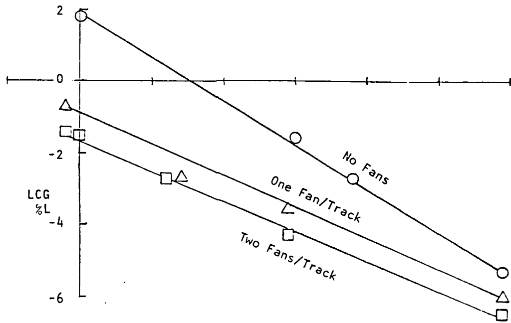
FIGURE 9 VARIATION OF DRAG WITH TRIM AT 8 MPH
