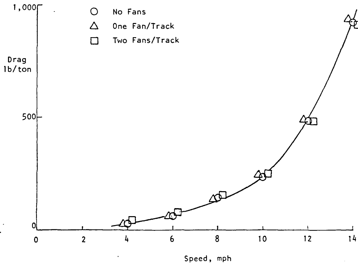
FIGURE 7 EFFECT OF TRACK BLOWING ON WATER DRAG
