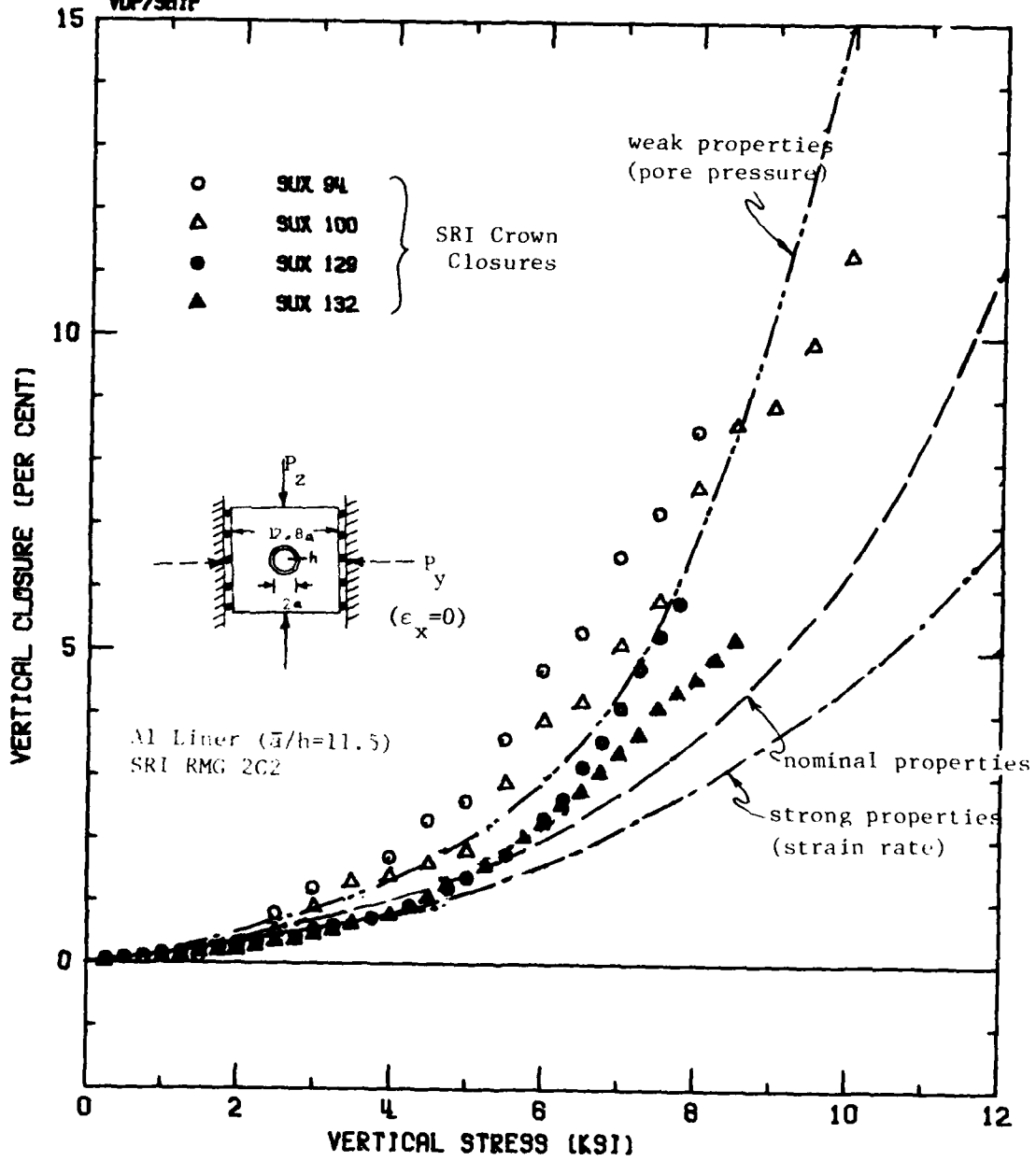
Figure 6.4. Effects of Material Property Variations on Tunnel Crown Closures.
