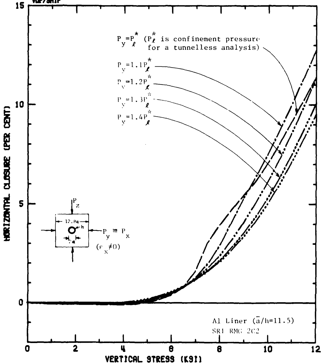
Fig. 3. Sensitivity Effect of Lateral Confinement Pressures on Tunnel Springline Closures.
