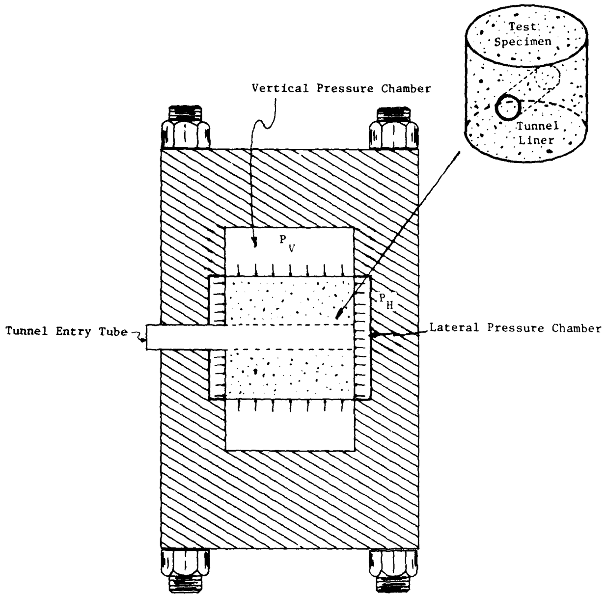
Figure 1.1. Schematic of SRI Triaxial Test Apparatus.
