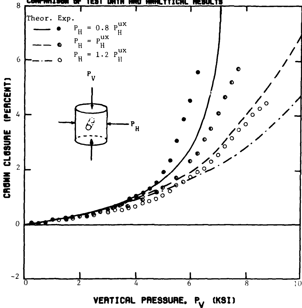
Figure 7.6. Comparison of Experimental and Theoretical Crown Closure in SRI RMG 2C2 for Uniaxial Strain, Overconfined and Underconfined Loadings. (Aluminum liner, \bar{a}/h = 11.5 . P_H^{ux} is lateral pressure required to maintain uniaxial strain as defined by SRI.)
