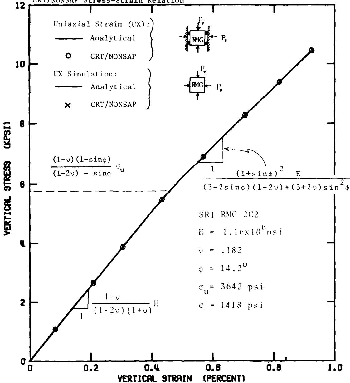
Figure 2.2. Preliminary Analysis Comparison of Analytical and Numerical Results for the Drucker-Prager Model.
