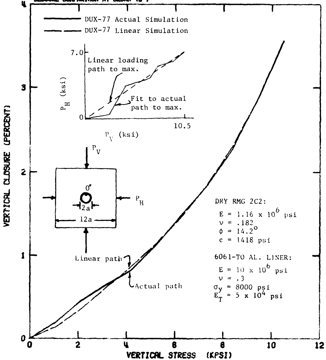
Figure 4.5. Numerical Simulation of Dynamic Test DUX-77, using Simple Linear Loading Path and Actual Fit to Measured Path.
