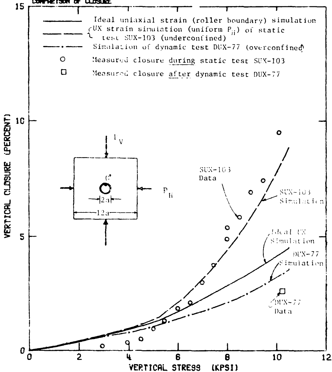
Figure S-2. Preliminary Analysis Comparison of Experimental and Theoretical Crown Closure in SRI RMG 2C2.
