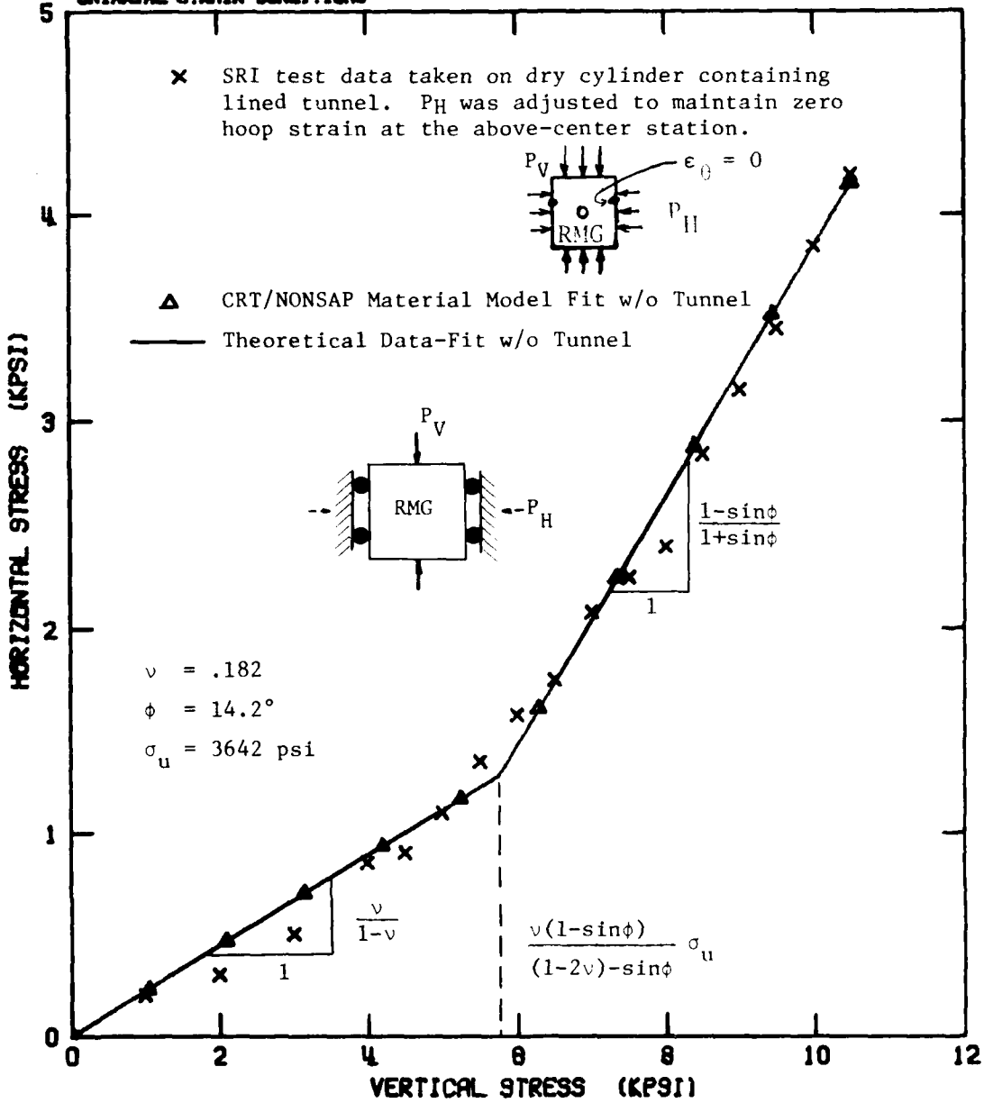
Figure 4.2. CRT/NONSAP Material Model Fit to SRI Test Data on Dry Sample (SUX-103).
