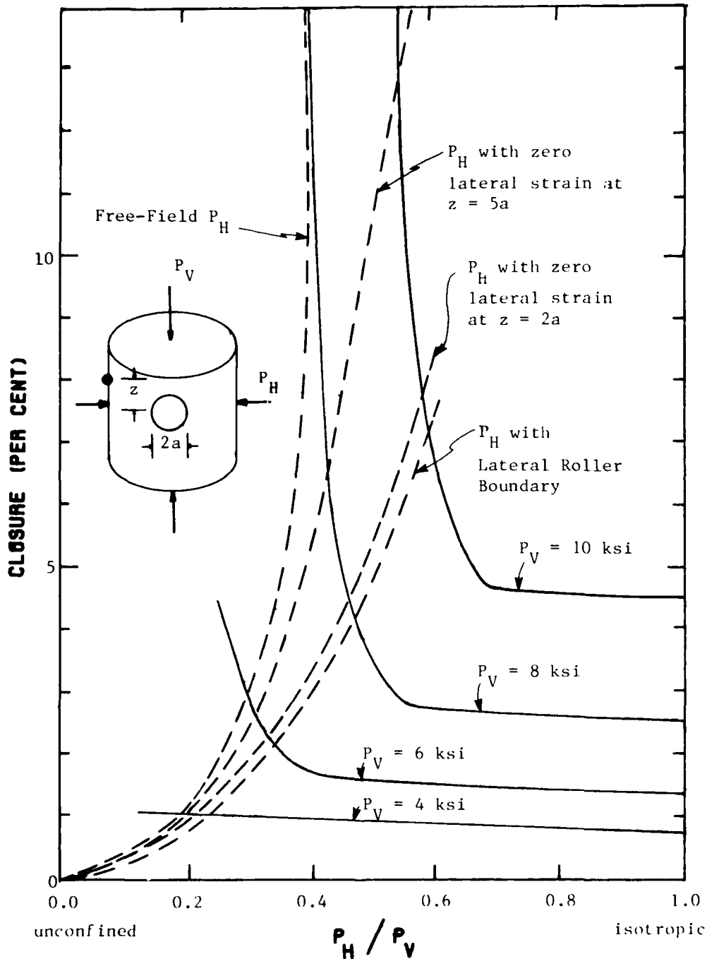
Figure 7.5. Sensitivity of Tunnel Crown Closure to Lateral Confinement Pressure for SRI RMG 2C2 Specimen with Aluminum Liner, \bar{a}/h = 11.5 .
