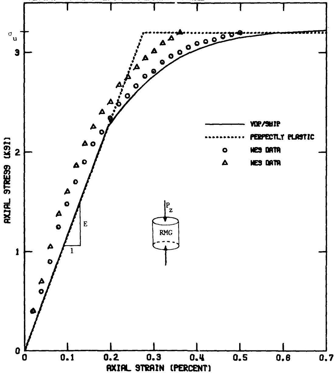
Figure A-2. Comparison of Unconfined Compression Stress-Strain Characteristics for the Combined Variable Friction Angle and Strain Hardening Versus Perfectly-Plastic Drucker-Prager Models of SRI RMG 2C2. ( E = 1.16 \times 10^6 psi, \sigma_u = 3200 psi.)
