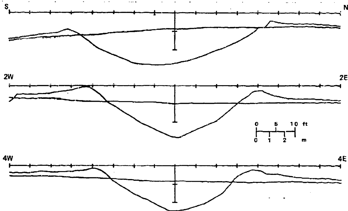
Figure 16. Slurry Row Crater—Cross-Sectional Profile.
