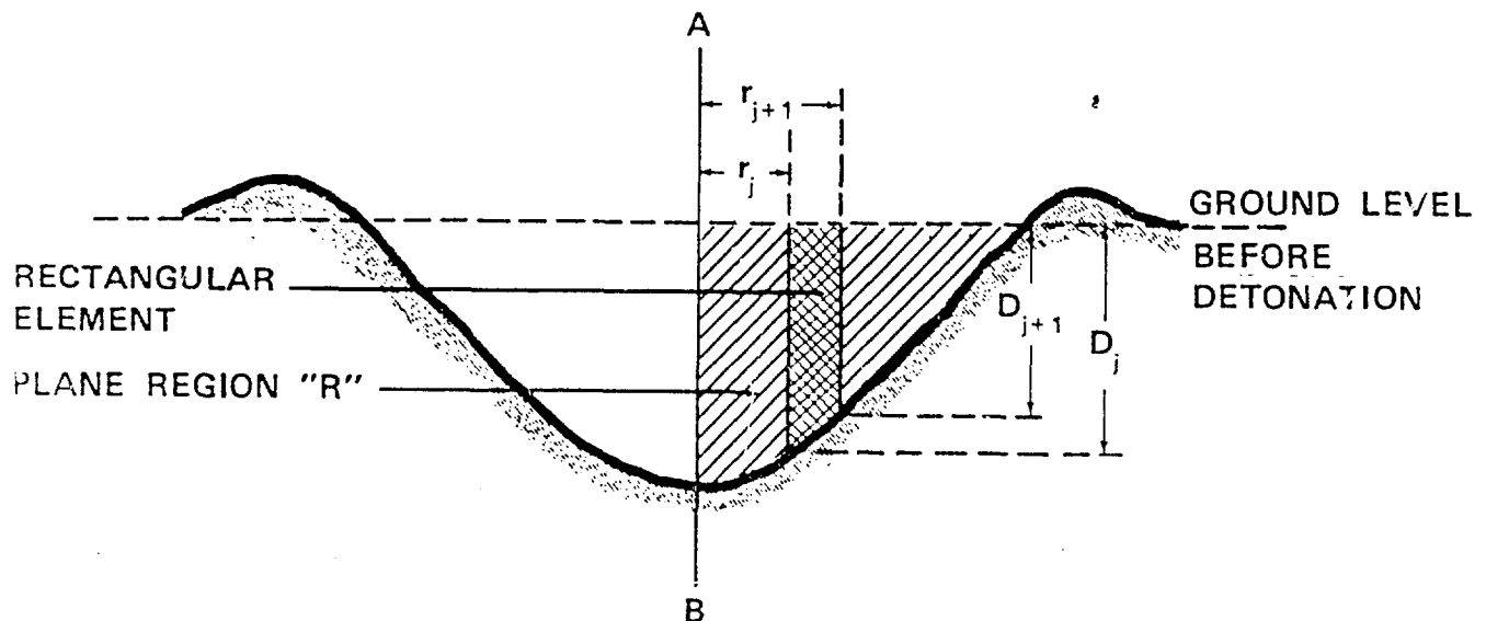
Figure C-3: Cross-sectional View of Typical Crater.
