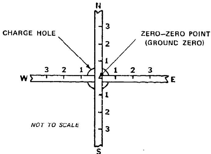
Figure 1. Measurement Orientation.
