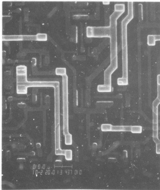
Fig. 4.4-7 A SEM photograph of a portion of a planar IC showing excellent lithography and high density. Note the second level interconnects running parallel above first level interconnects.
