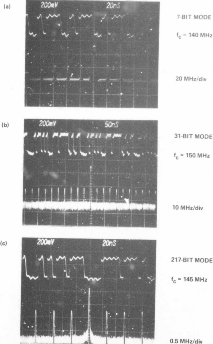
Fig. 6.3-13 Output waveforms for the 8-stage shift register operating in the pseudo-noise generation mode. The upper traces represent the output for each of the three codes while the lower traces represent the corresponding frequency spectra.
