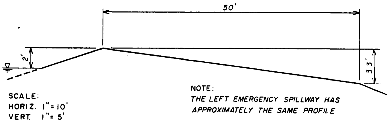
SECTION A-A (RIGHT EMERGENCY SPILLWAY PROFILE)
