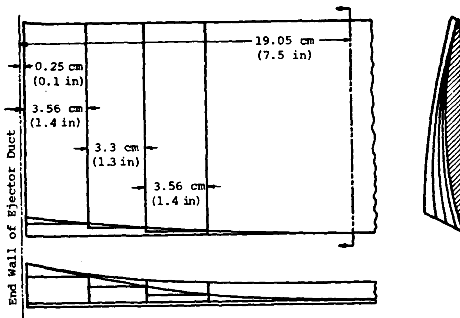
(a) Expanded Configuration
