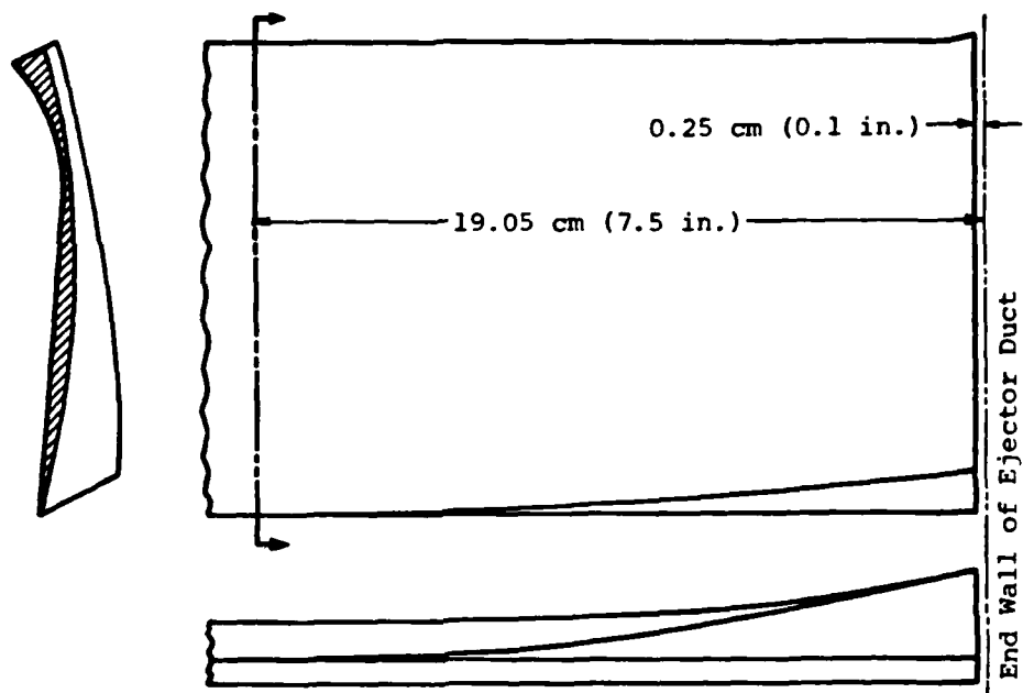
Figure B-3. Diffuser Inboard Panel
