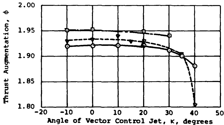
Figure 8. Performance of the Thrust Vector Control System
