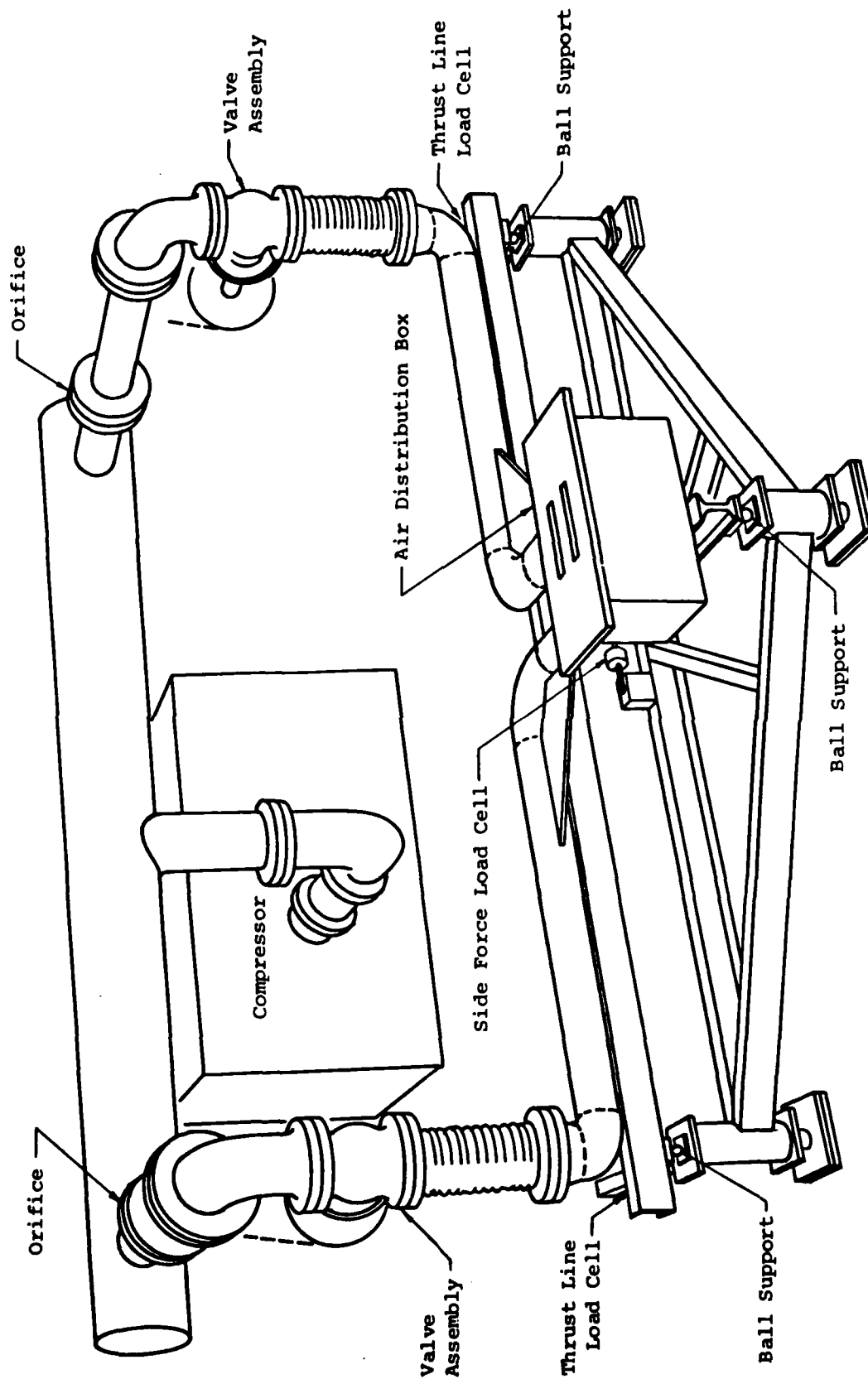
Figure A-1. FDR Static Ejector Test Rig
