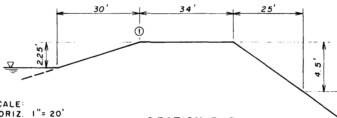
SECTION B-B EMERGENCY SPILLWAY PROFILE
