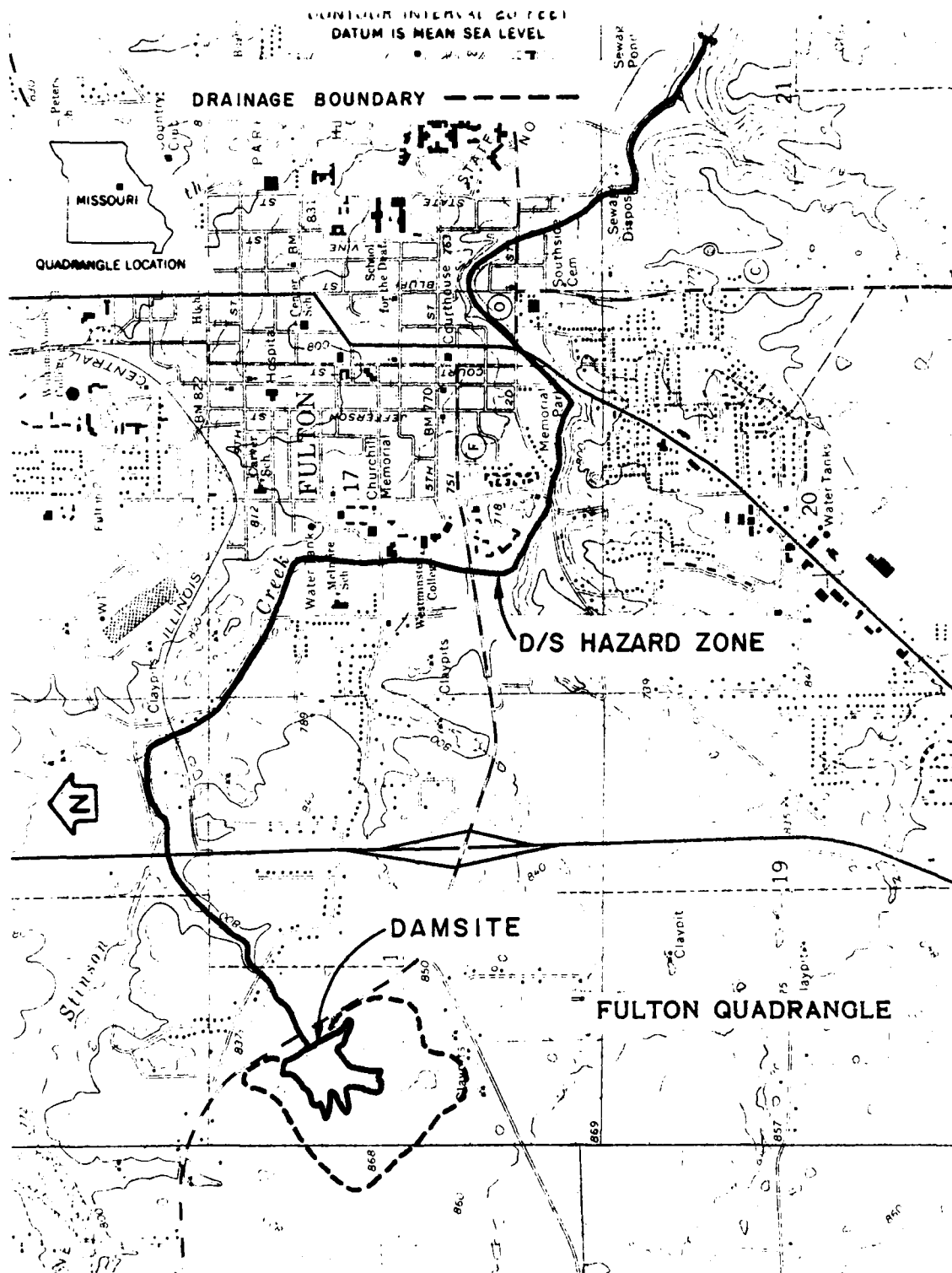
HAUCK LAKE DAM (MO. 10989) DRAINAGE BASIN AND DOWNSTREAM HAZARD ZONE
