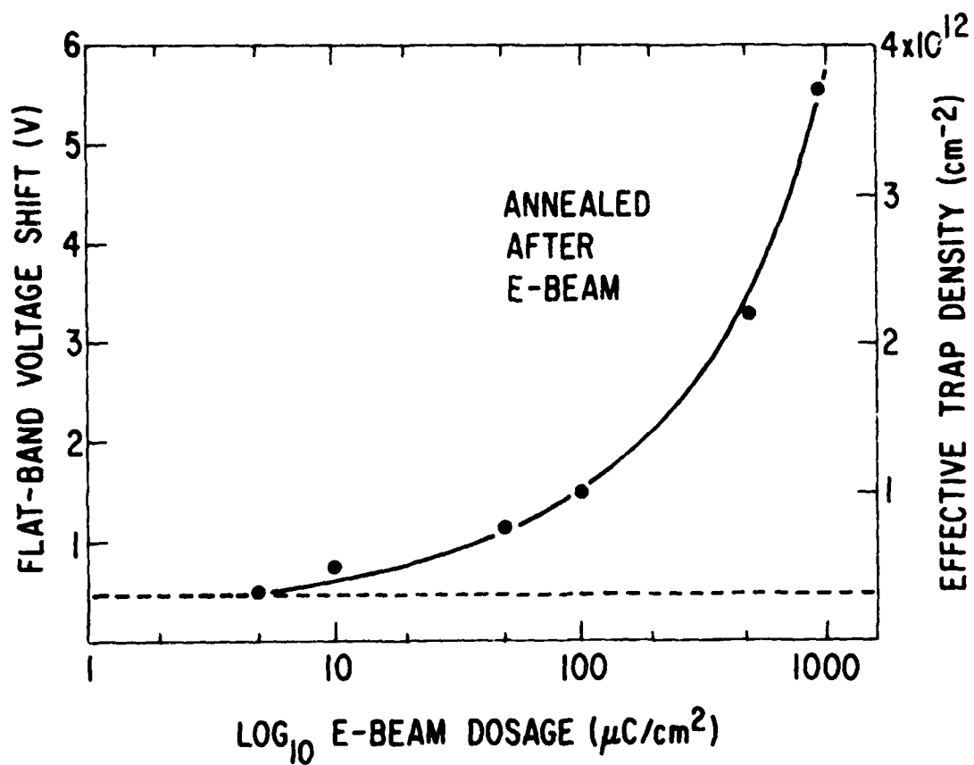
Fig. 2. The flat-band voltage shift (effective trap density) observed after 1 \times 10^{14} holes/cm 2 have been injected through the capacitors. The flat dotted line indicates the level of traps observed in the as-grown oxide.
