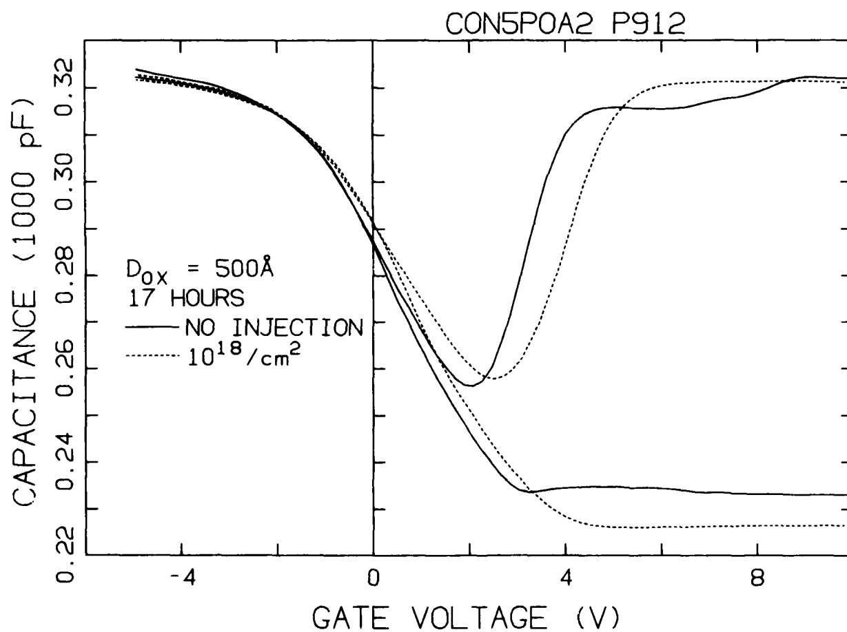
Fig. IV High frequency and quasistatic capacitance before and after injection of 10^{18} / \text{cm}^2 electrons for an oxide that was annealed in nitrogen for 17 hours.
