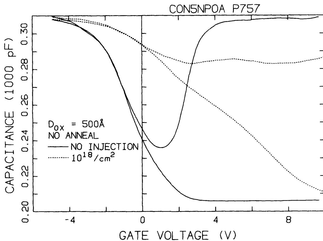
Fig. II High frequency and quasistatic capacitance before and after injection of 10^{18}/\text{cm}^2 electrons for an oxide that has not been annealed in nitrogen.
