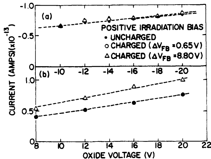
Fig5. The photoemission characteristics of an MOS capacitor with a semitransparent aluminum gate are shown before and after irradiation under positive bias. These samples had 50 nm oxides which were subjected 25KV X-rays. The capacitor was irradiated and measured twice as shown in the figure. In this case the charge is located at the Si/SiO 2 interface.
