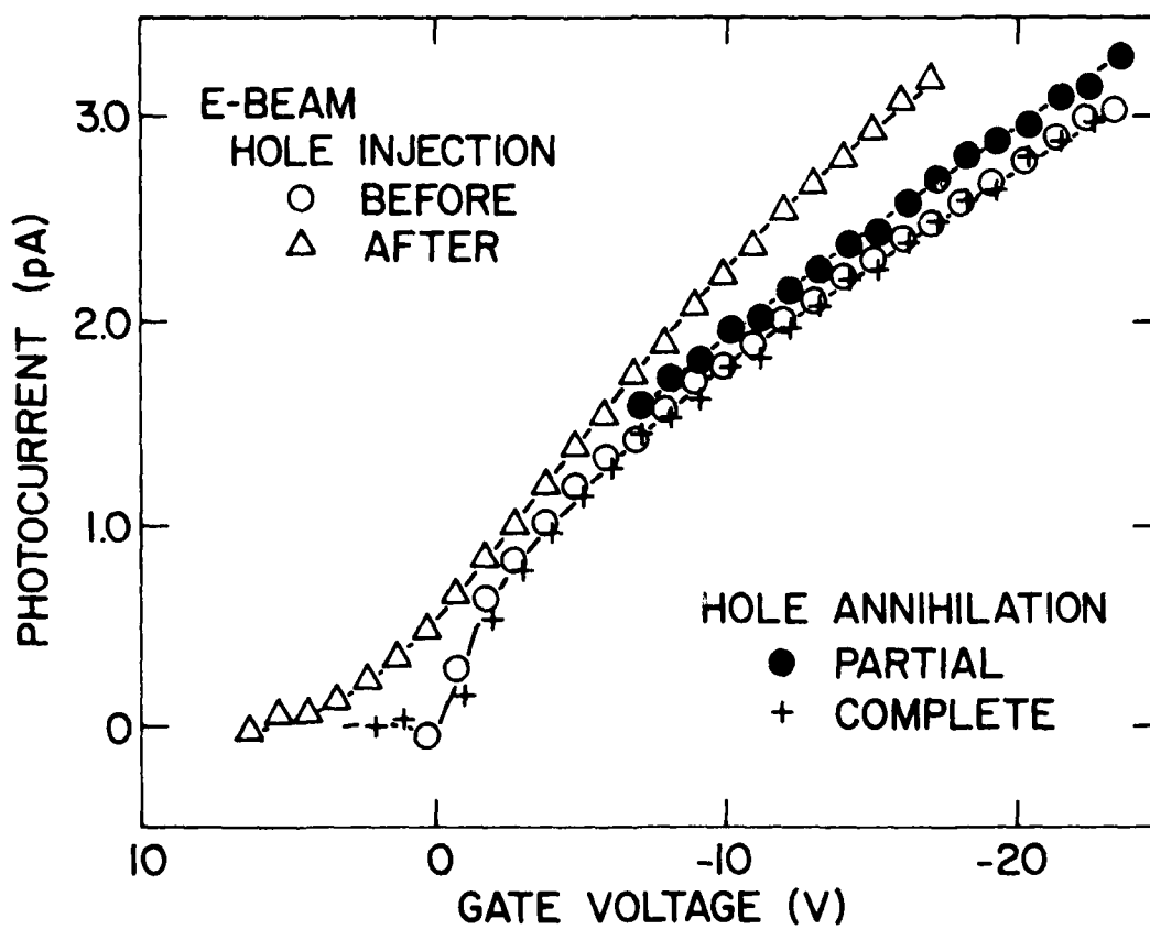
Fig. 3. Photoemission current versus gate voltage for sample measured before and after holes were injected into the oxide and after these holes have been annihilated by photo-injected electrons. The oxide was 80.0 \mu\text{m} thick. Samples was annealed after exposure to 50 KV electrons.
