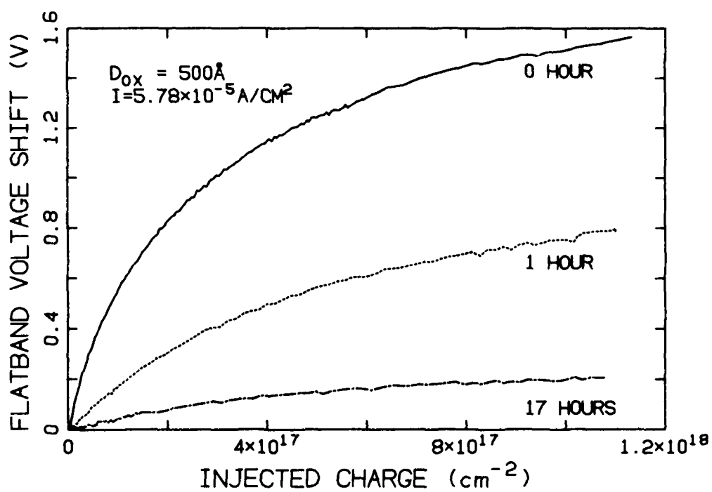
Fig. 1 Flatband voltage shift as a function of injected charge for 500 Å oxides that are annealed in nitrogen for 0 hour, 1 hour and 17 hours, respectively. Injection was carried out at 100°C.
