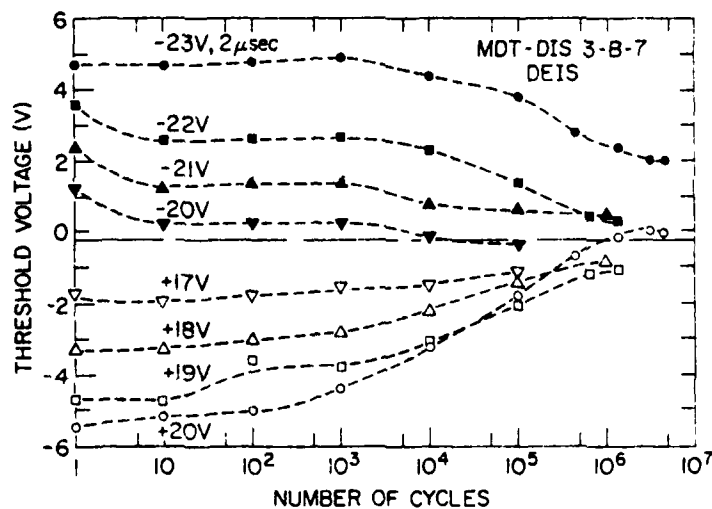
Figure 3. Threshold voltage after writing and erasing as a function of the number of cycles for various write/erase voltage conditions on DEIS FETs from wafer MDT-DIS 3-B. Solid and open symbols correspond to the threshold voltage after writing and erasing for 2 \mu sec, respectively. The horizontal dashed line indicates the initial threshold voltage of the as-fabricated FETs before cycling.
