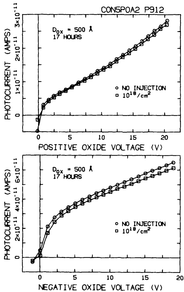
Fig. VIII Photo I-V curves for before and after injection of 10^{18}/\text{cm}^2 electrons for an oxide that was annealed in nitrogen for 17 hours.
