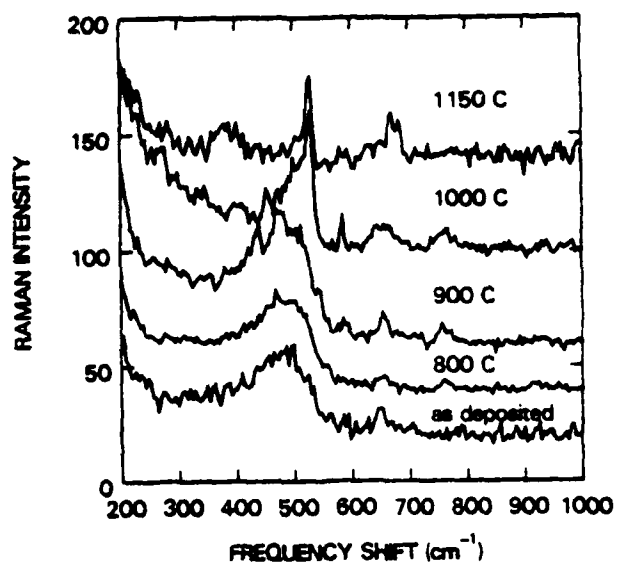
Figure 1 shows the Raman scattering spectra for Si rich \text{SiO}_2 films as-deposited and annealed at various temperatures.
