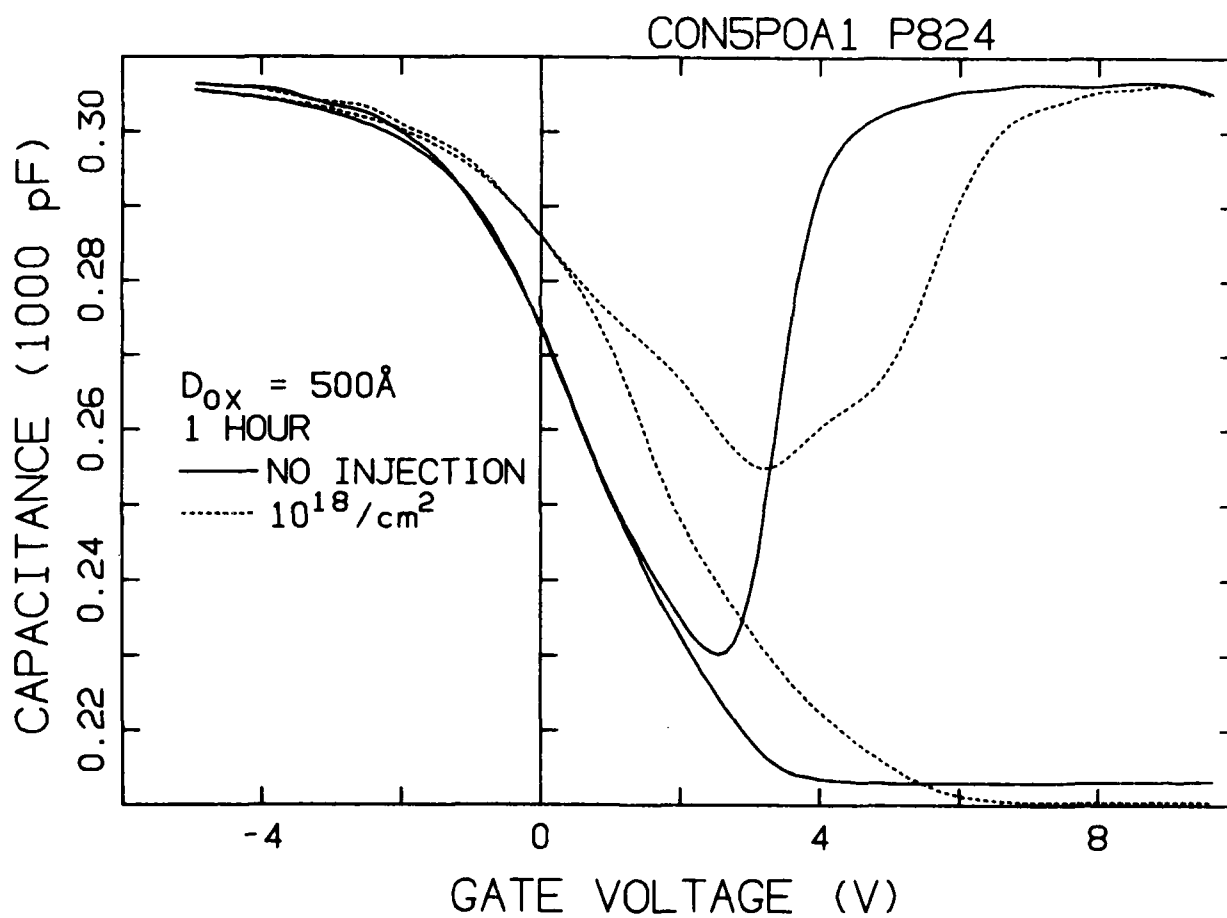
Fig. III High frequency and quasistatic capacitance before and after injection of 10^{18}/\text{cm}^2 electrons for an oxide that was annealed in nitrogen for 1 hour.
