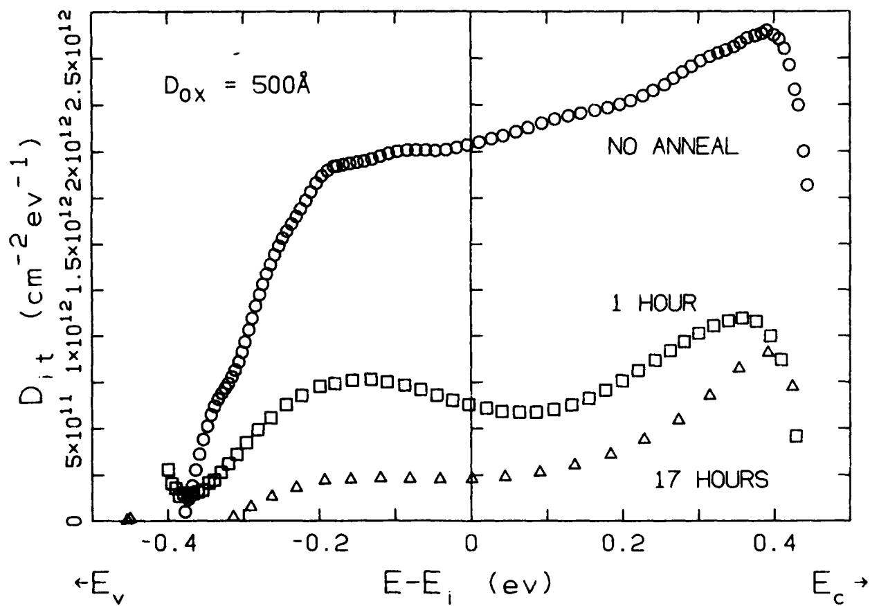
Fig. V Interface state densities after injection of 10^{18}/\text{cm}^2 electrons for 500 Å oxides that are annealed in nitrogen for 0 hour, 1 hour and 17 hours, respectively. Any lateral nonuniformity effect has been ignored in the analysis and if the effect is large, these represent apparent interface state densities.
