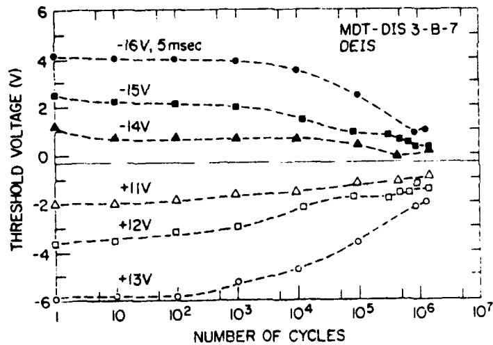
Figure 2. Threshold voltage after writing and erasing as a function of the number of cycles for various write/erase voltage conditions on DEIS FETs from wafer MDT-DIS 3-B, as described in the text of this communication. Solid and open symbols correspond to the threshold voltage after writing and erasing for 5 msec, respectively. The horizontal dashed line indicates the initial threshold voltage of the as-fabricated FETs before cycling.
