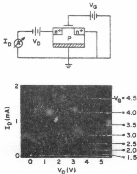
Fig.2 The effect of gate voltage on the current between source and drain is illustrated in this figure. The source-drain current is plotted against the voltage between these contacts. A circuit diagram defining the measured quantities is also given. The gate oxide of this device is 25 nm thick.
