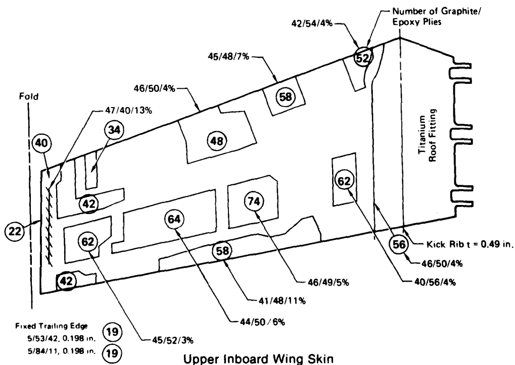
Figure 13. F-18 Inboard Wing Skin Lay-Up Distribution
