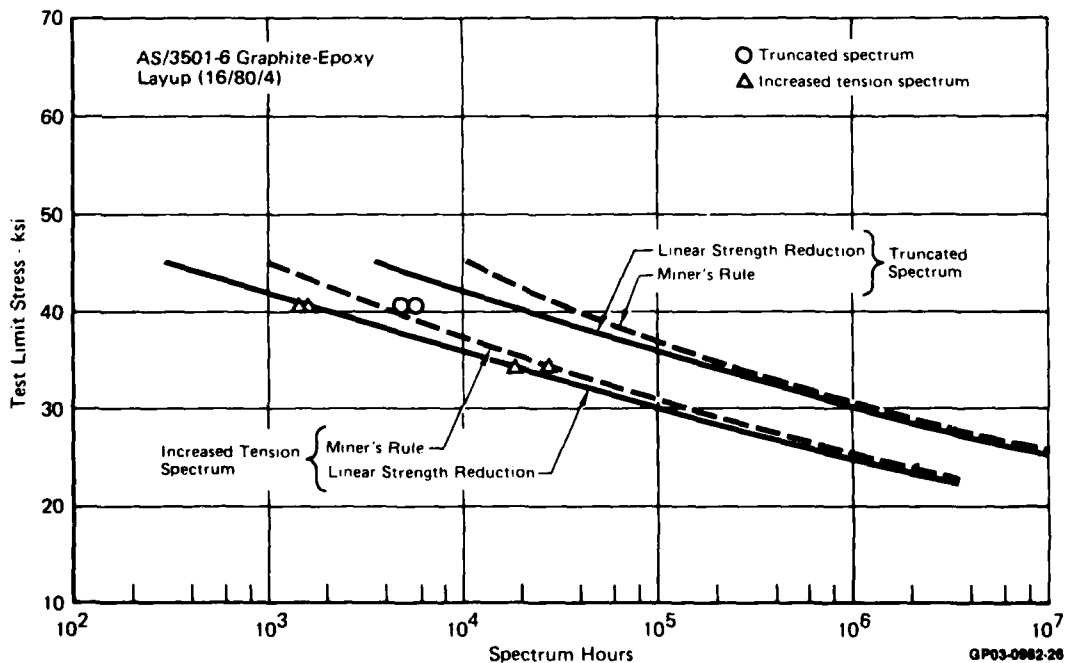
Figure 28. Comparison of Linear Strength Reduction and Miner's Rule Predictions
