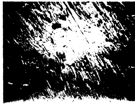
Fig. 29 — SEM micrographs of worn flutes on specimens 1F and 2B of the 7/16 in. diam. end mill. The lower left hand photograph shows the principal regions starting from the cutting edge at the bottom, land with wear region extending up from the cutting edge, and lighter region on back of flute with grinding marks readily visible. The unimplanted tool (top) has cracked and chipped in the worn region while the implanted tool shows abrasive wear and plastic flow along the worn surface.
